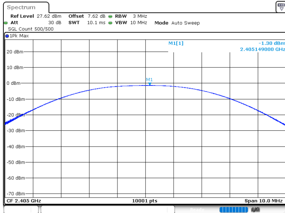
Power NVNT GFSK 2405MHz Ant1
