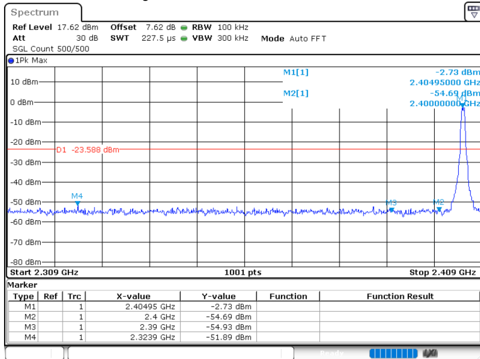
Band Edge NVNT GFSK 2405MHz Ant1 Emission
