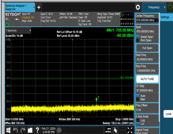
11AX20MIMO-Ant2-2412-30~1000-PASS
