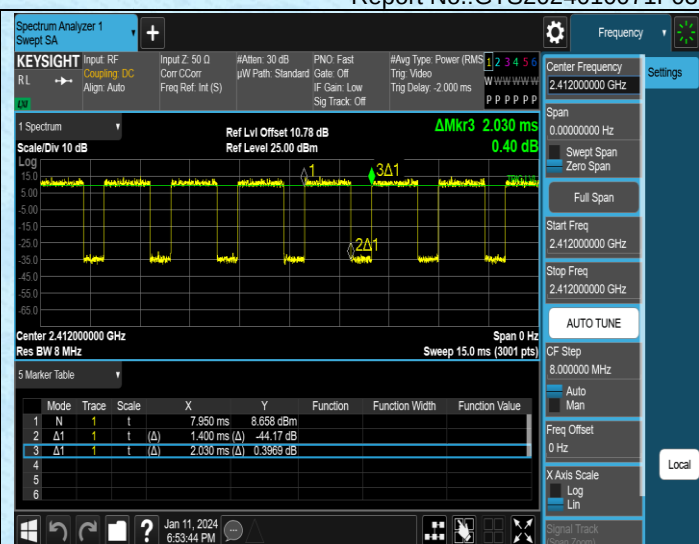
NTNV-11G-Ant2-2412
