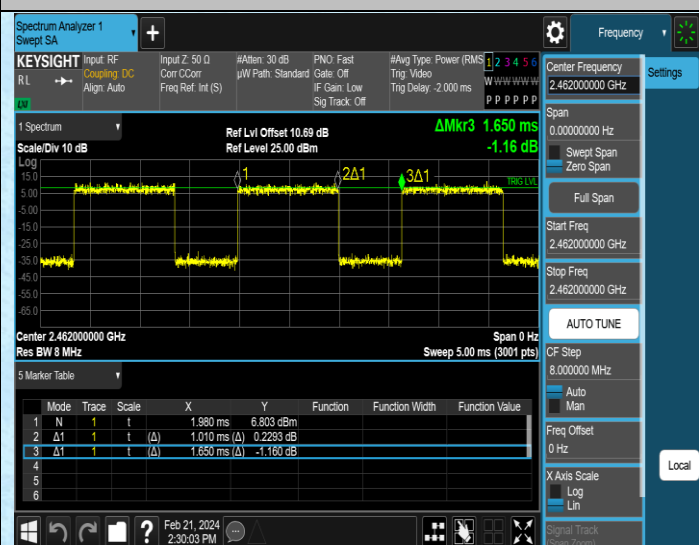
NTNV-11AX20SISO-Ant2-2462
