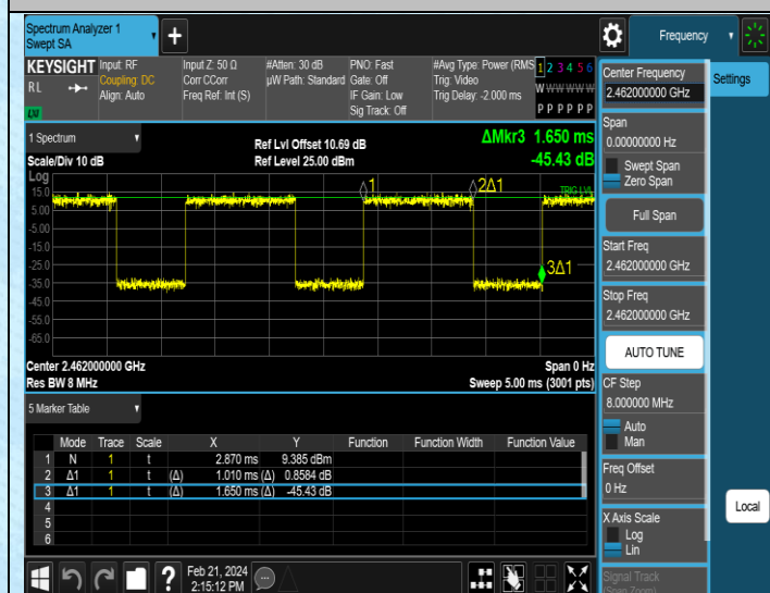
NTNV-11AX20SISO-Ant1-2462
