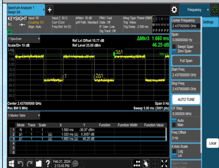
NTNV-11AX20SISO-Ant1-2437
