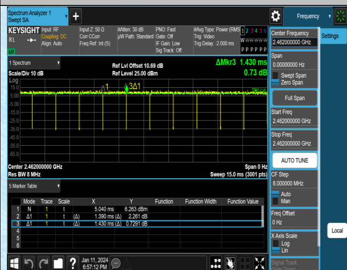
NTNV-11G-Ant2-2462
