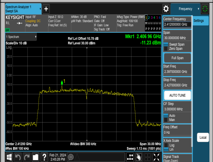
11AX20MIMO-Ant2-2412-0-Reference-PASS
