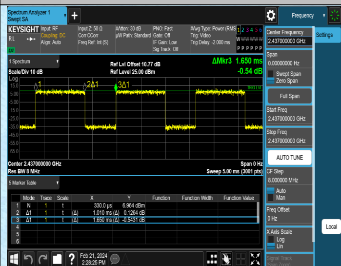
NTNV-11AX20SISO-Ant2-2437
