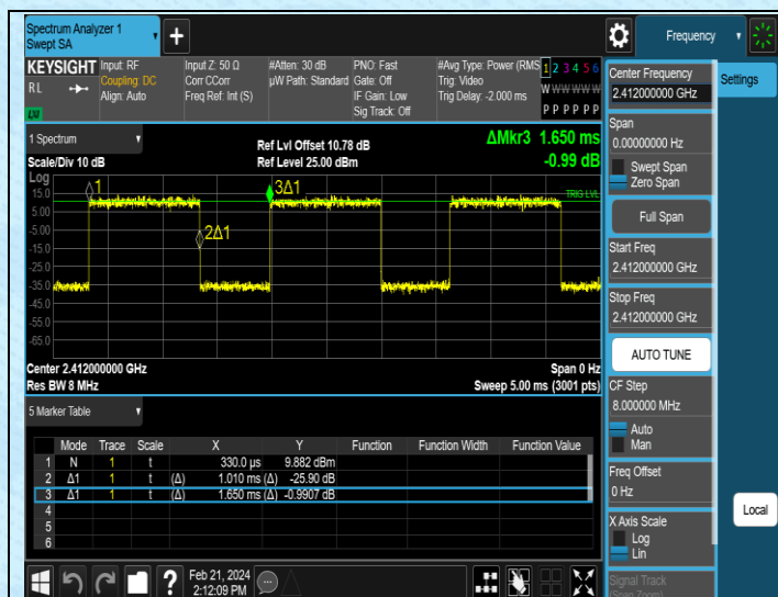
NTNV-11AX20SISO-Ant1-2412
