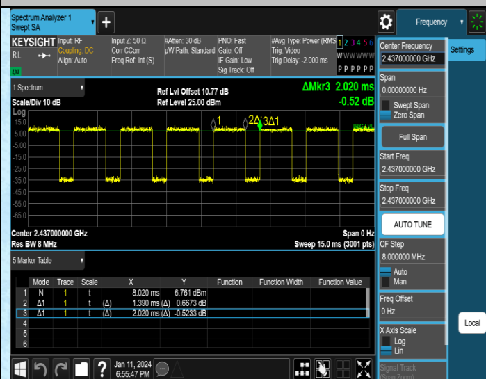
NTNV-11G-Ant2-2437
