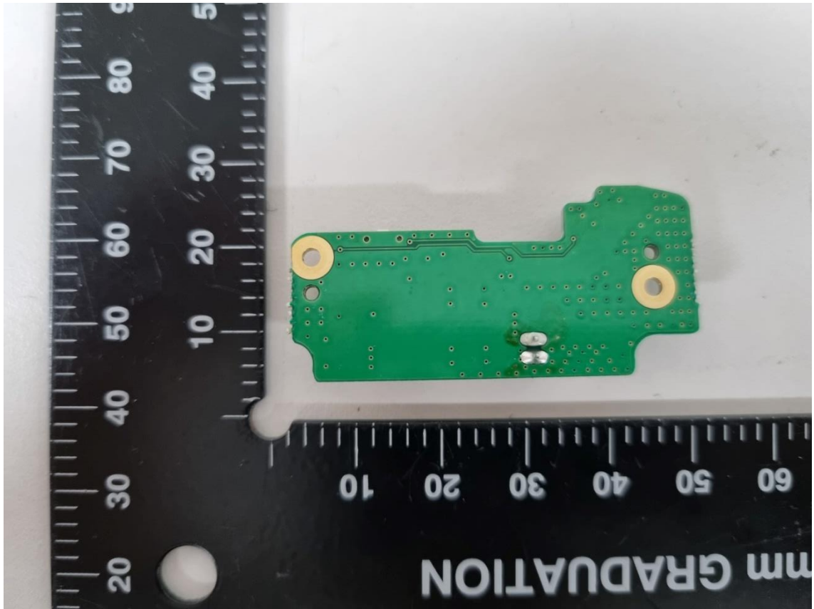
Sub Board (Battery, Rear)
