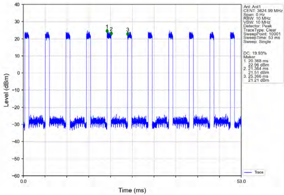
n48_30kHz_SISO_NTNV_30MHz_CP-OFDM QPSK_3624.99MHz_Inner_Full_Ant1
