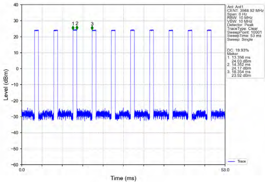
n48_30kHz_SISO_NTNV_40MHz_DFT-s-OFDM QPSK_3570MHz_Inner_Full_Ant1
