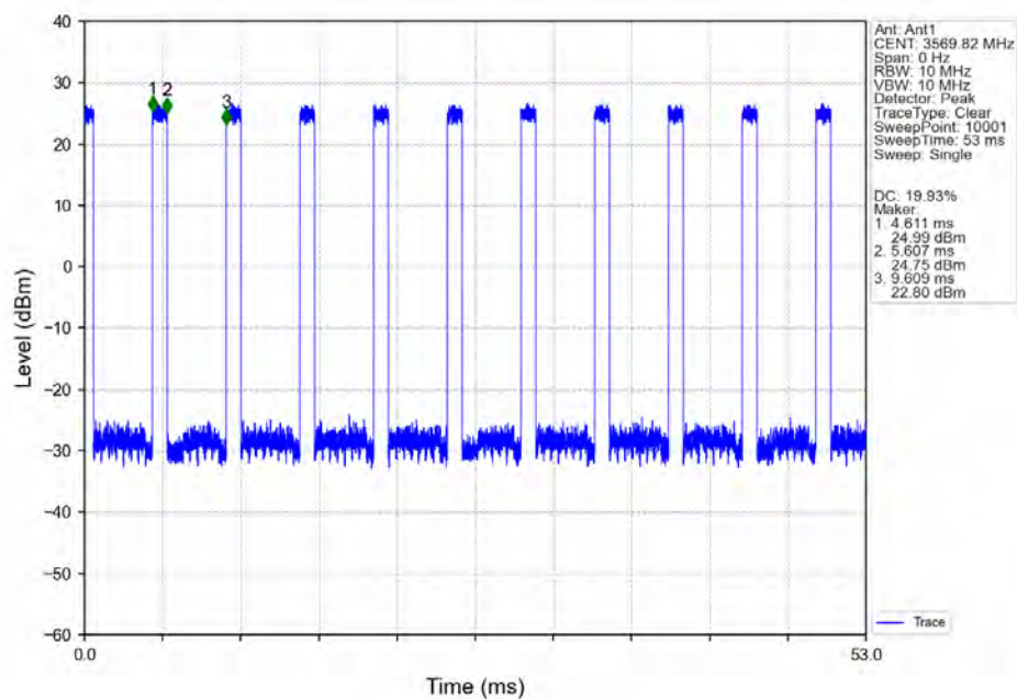
n48_30kHz_SISO_NTNV_40MHz_CP-OFDM_16_QAM_3570MHz_Inner_Full_Ant1
