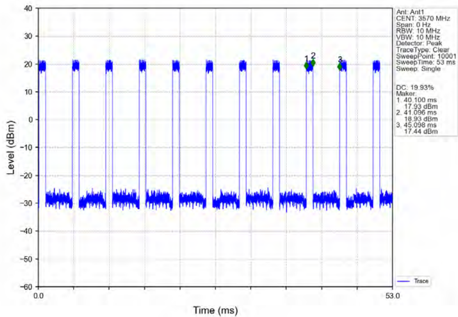
n48_30kHz_SISO_NTNV_40MHz_CP-OFDM_64_QAM_3570MHz_Inner_Full_Ant1
