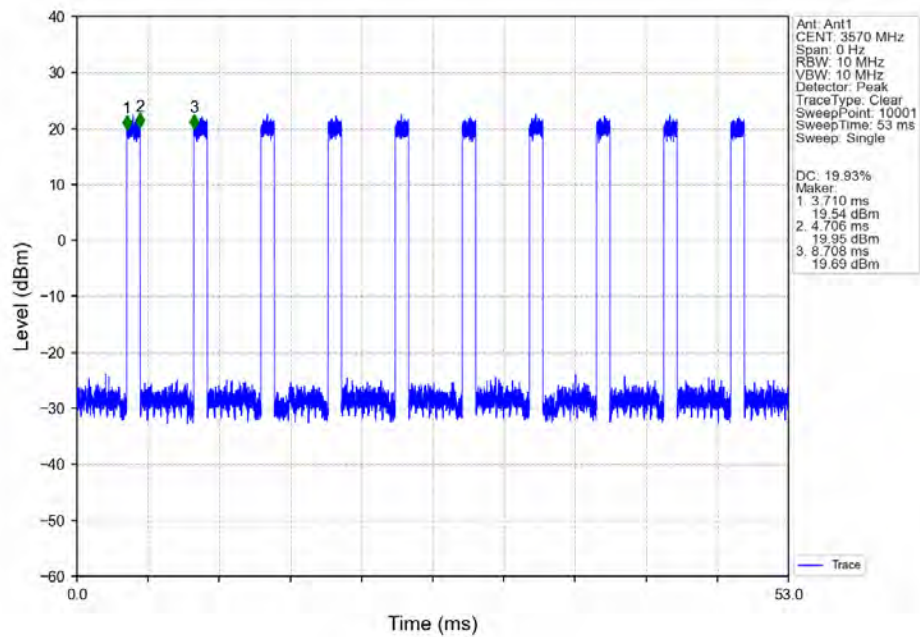
n48_30kHz_SISO_NTNV_40MHz_CP-OFDM_16_QAM_3570MHz_Inner_Full_Ant1
