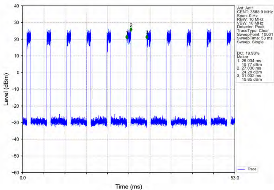
n48_30kHz_SISO_NTNV_40MHz_DFT-s-OFDM_256_QAM_3570MHz_Edge_1RB_Right_Ant1
