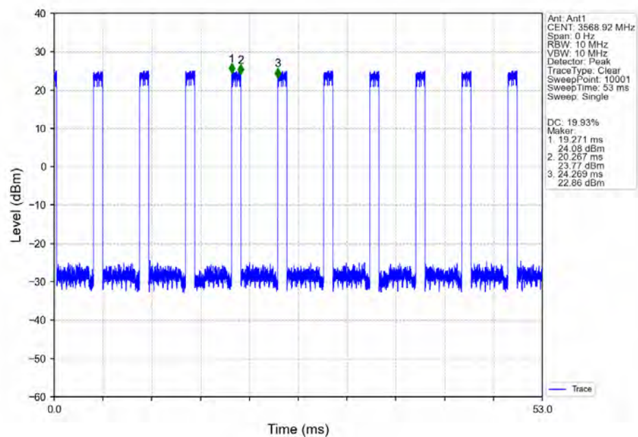
n48_30kHz_SISO_NTNV_40MHz_DFT-s-OFDM_64_QAM_3570MHz_Inner_Full_Ant1
