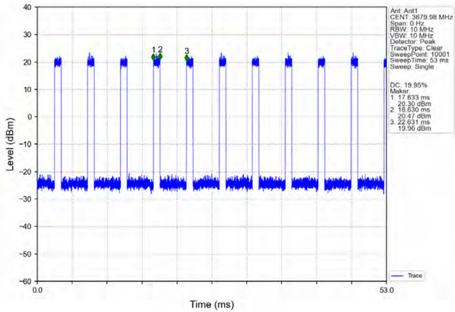
n48_30kHz_SISO_NTNV_40MHz_CP-OFDM QPSK_3679.98MHz_Inner_Full_Ant1
