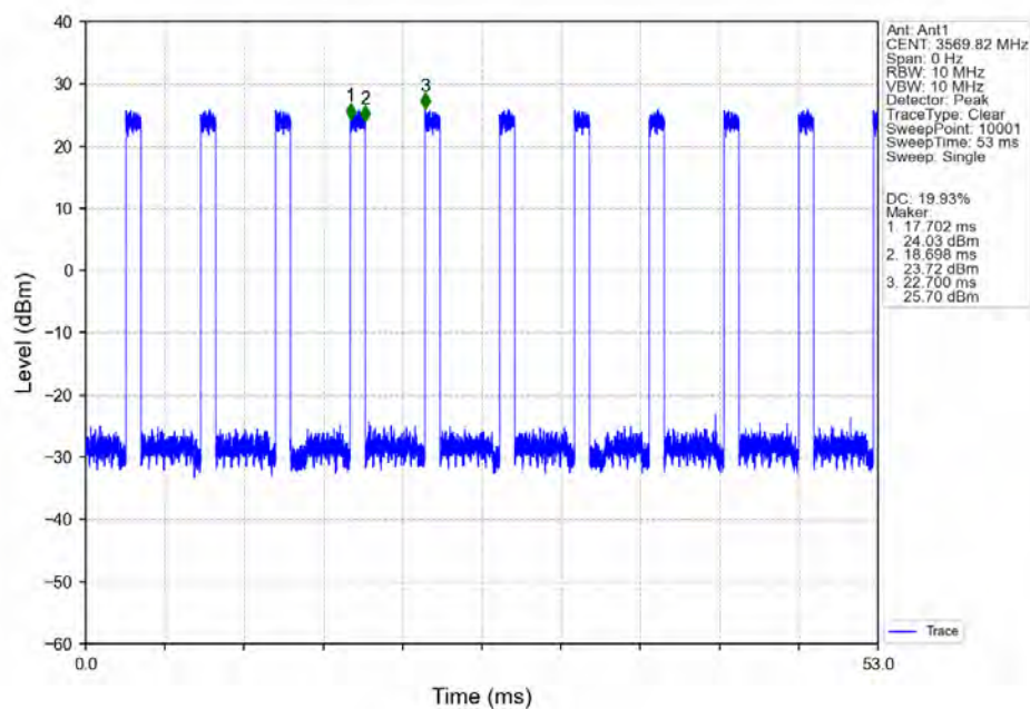
n48_30kHz_SISO_NTNV_40MHz_CP-OFDM_64_QAM_3570MHz_Inner_Full_Ant1
