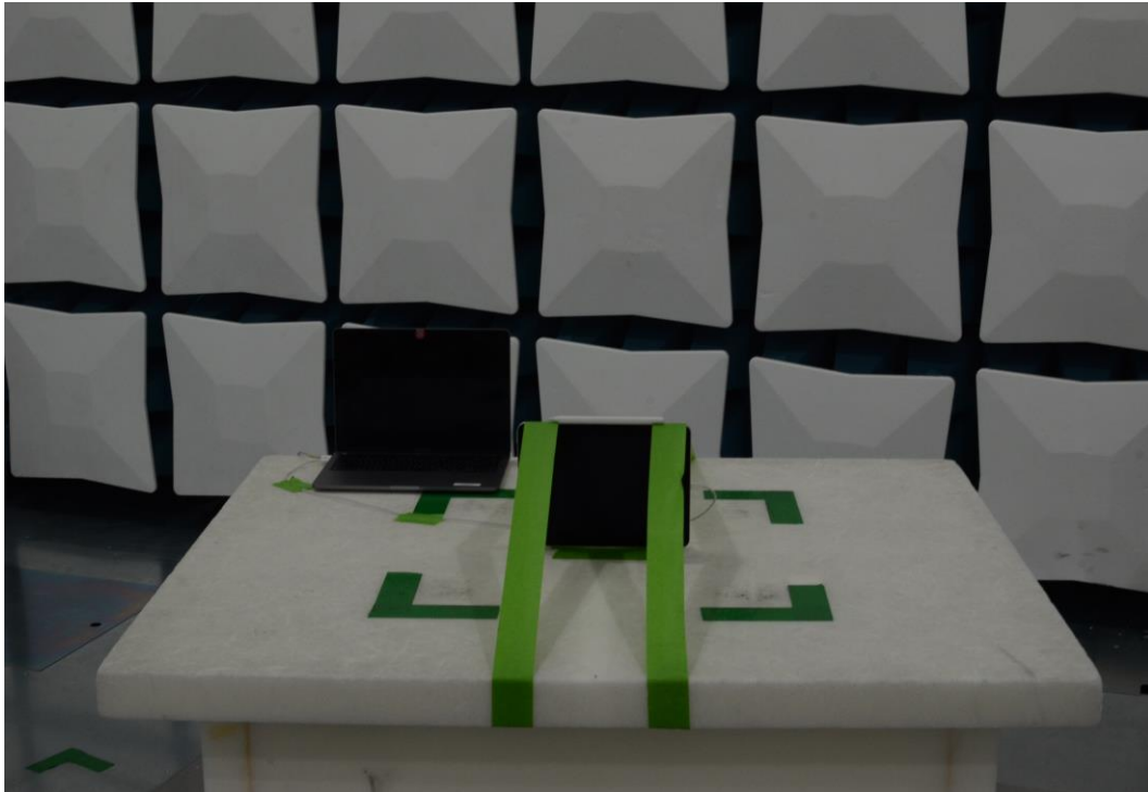
Figure 19: 30MHz-1GHz Test Setup (Front View)
