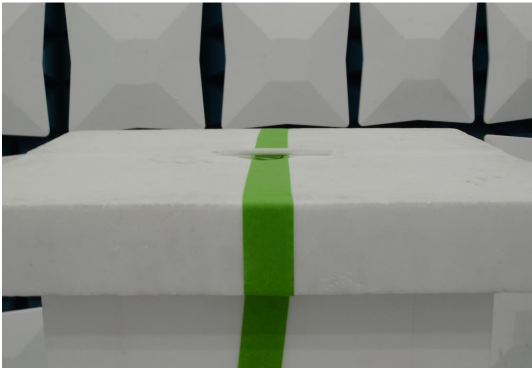
Figure 7: 1-18GHz Test Setup (Front View)
