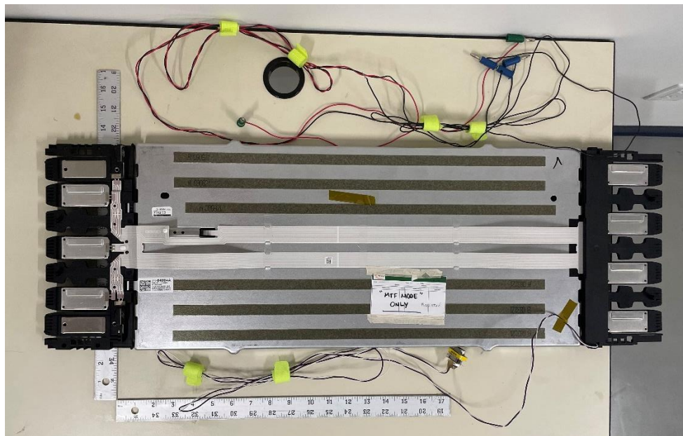
Figure B2. DUT and Harness
