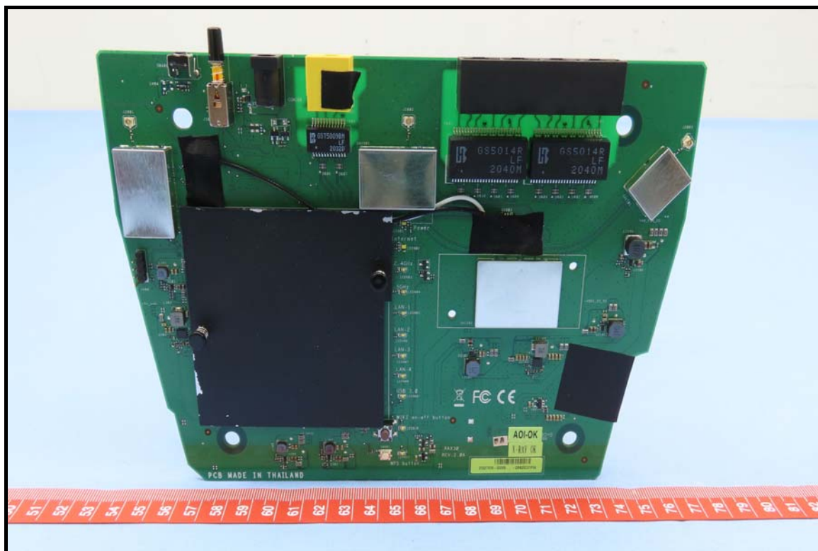
2nd FEM
