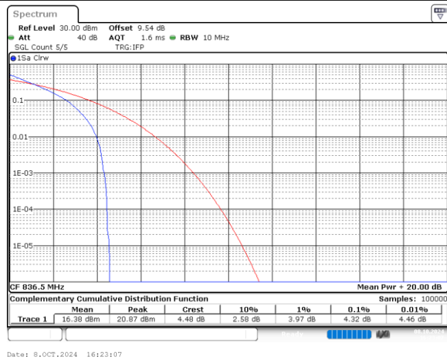
Band26-15MHz-16QAM-26915-6-0-Low-4.32-<=13-PASS
