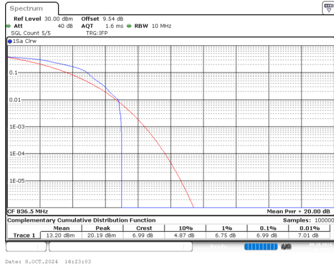
Band26-15MHz-16QAM-26915-1-0-Low-6.99-<=13-PASS
