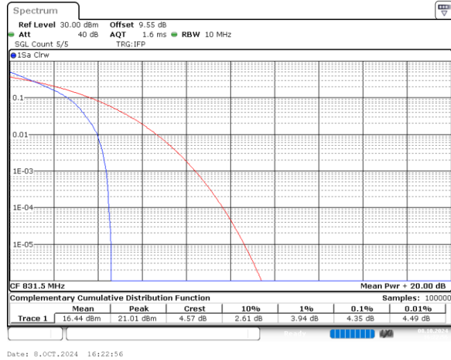
Band26-15MHz-16QAM-26865-6-0-Low-4.35-<=13-PASS
