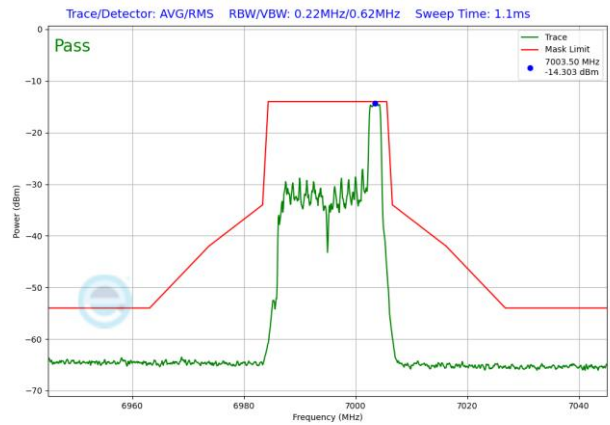
Plot 7-1509. LPI In-Band Emission Plot SDM Diversity Antenna WF8 (20MHz 802.11ax RU26 (UNII Band 8) – Ch. 209)
