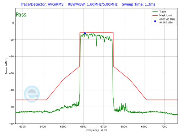
Plot 7-1504. LPI In-Band Emission Plot SDM Diversity Antenna WF7 (160MHz 802.11ax RU996x2 (UNII Band 7) – Ch. 143)
