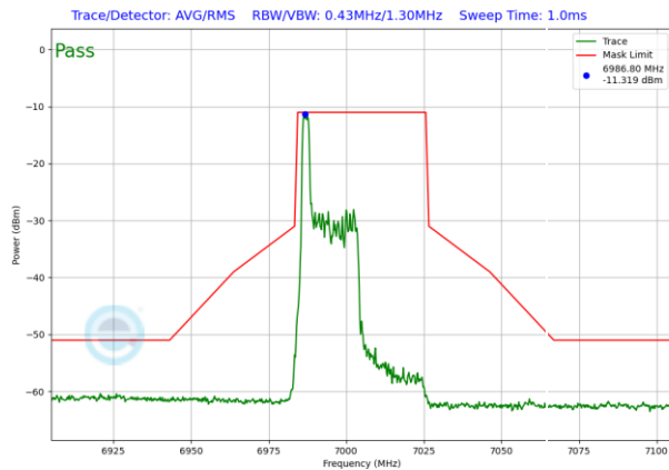
Plot 7-1513. LPI In-Band Emission Plot SDM Diversity Antenna WF8 (40MHz 802.11ax RU26 (UNII Band 8) – Ch. 211)
