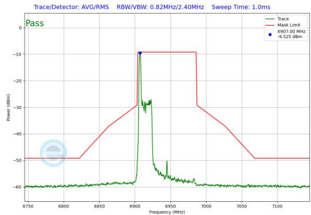
Plot 7-1521. LPI In-Band Emission Plot SDM Diversity Antenna WF8 (80MHz 802.11ax RU26 (UNII Band 8) – Ch. 199)
