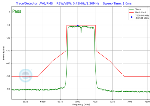
Plot 7-1519. LPI In-Band Emission Plot SDM Diversity Antenna WF8 (40MHz 802.11ax RU484 (UNII Band 8) – Ch. 211)
