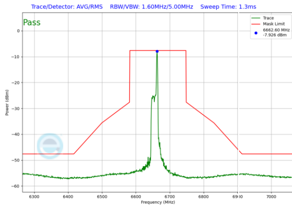
Plot 7-1499. LPI In-Band Emission Plot SDM Diversity Antenna WF8 (160MHz 802.11ax RU26 (UNII Band 7) – Ch. 143)
