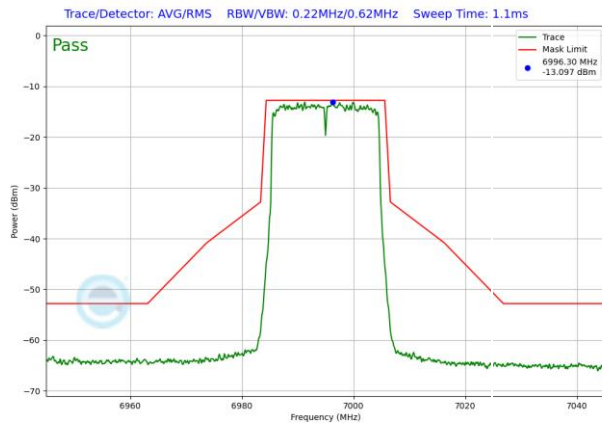
Plot 7-1511. LPI In-Band Emission Plot SDM Diversity Antenna WF8 (20MHz 802.11ax RU242 (UNII Band 8) – Ch. 209)
