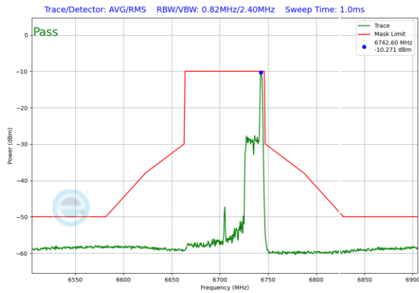
Plot 7-1493. LPI In-Band Emission Plot SDM Diversity Antenna WF8 (80MHz 802.11ax RU26 (UNII Band 7) – Ch. 151)
