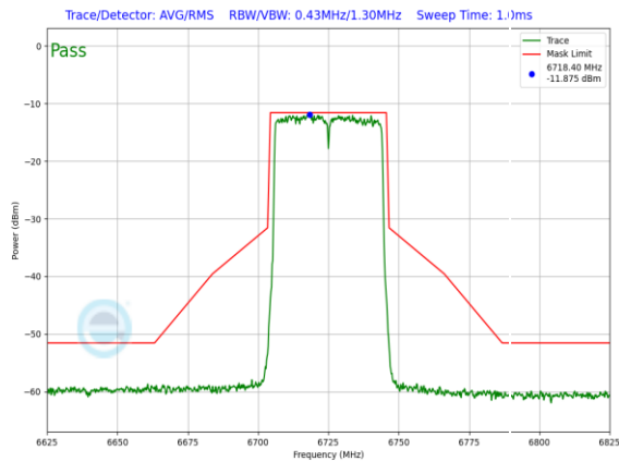
Plot 7-1488. LPI In-Band Emission Plot SDM Diversity Antenna WF7 (40MHz 802.11ax RU484 (UNII Band 7) – Ch. 155)
