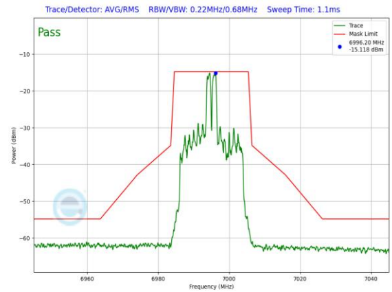
Plot 7-1508. LPI In-Band Emission Plot SDM Diversity Antenna WF7 (20MHz 802.11ax RU26 (UNII Band 8) – Ch. 209)
