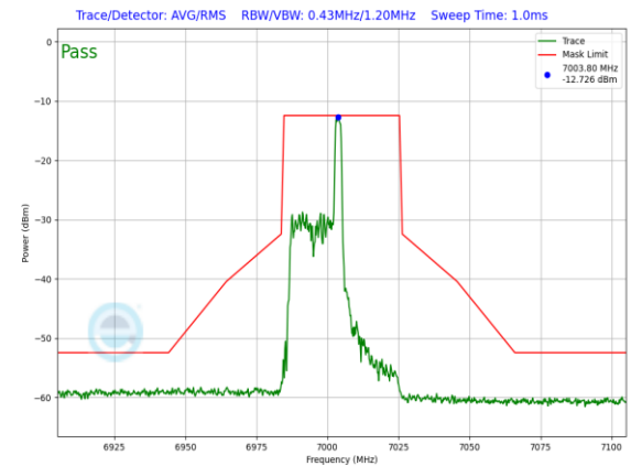
Plot 7-1516. LPI In-Band Emission Plot SDM Diversity Antenna WF7 (40MHz 802.11ax RU26 (UNII Band 8) – Ch. 211)
