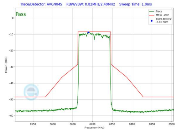
Plot 7-1496. LPI In-Band Emission Plot SDM Diversity Antenna WF7 (80MHz 802.11ax RU996 (UNII Band 7) – Ch. 151)
