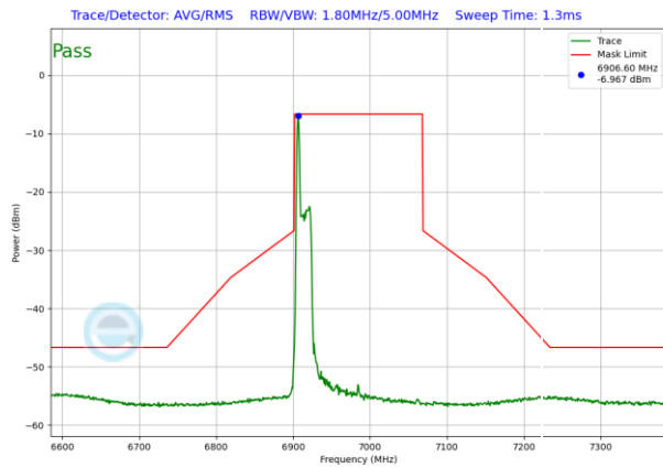
Plot 7-1529. LPI In-Band Emission Plot SDM Diversity Antenna WF8 (160MHz 802.11ax RU26 (UNII Band 8) – Ch. 207)
