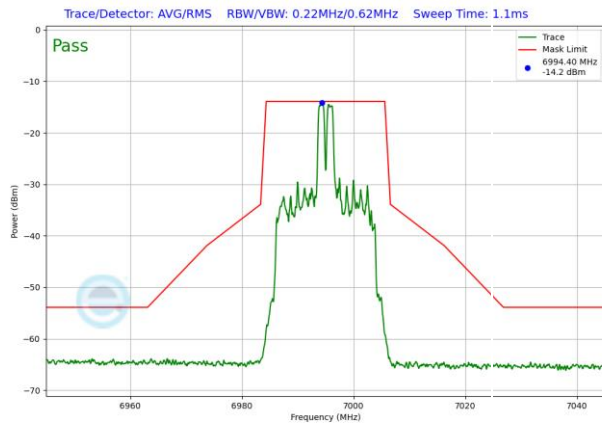
Plot 7-1507. LPI In-Band Emission Plot SDM Diversity Antenna WF8 (20MHz 802.11ax RU26 (UNII Band 8) – Ch. 209)
