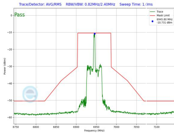
Plot 7-1524. LPI In-Band Emission Plot SDM Diversity Antenna WF7 (80MHz 802.11ax RU26 (UNII Band 8) – Ch. 199)
