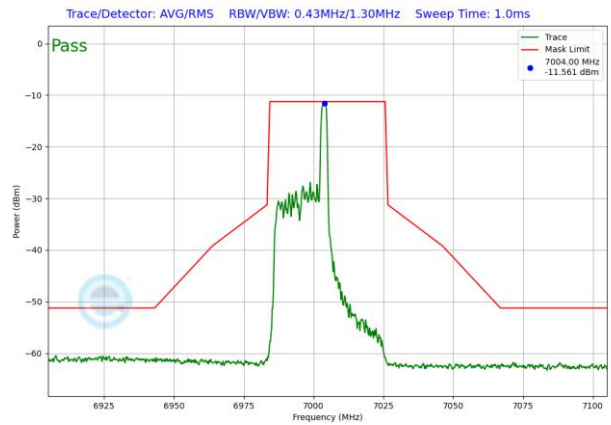
Plot 7-1515. LPI In-Band Emission Plot SDM Diversity Antenna WF8 (40MHz 802.11ax RU26 (UNII Band 8) – Ch. 211)
