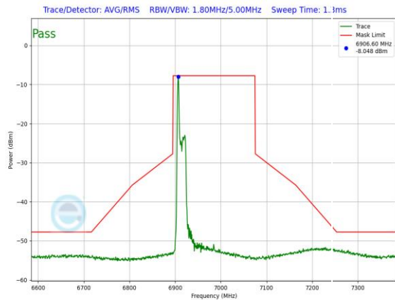
Plot 7-1530. LPI In-Band Emission Plot SDM Diversity Antenna WF7 (160MHz 802.11ax RU26 (UNII Band 8) – Ch. 207)
