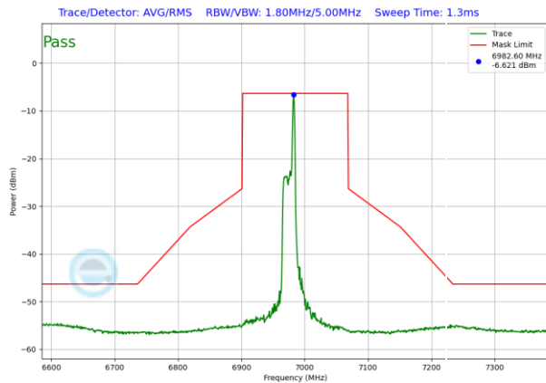
Plot 7-1531. LPI In-Band Emission Plot SDM Diversity Antenna WF8 (160MHz 802.11ax RU26 (UNII Band 8) – Ch. 207)
