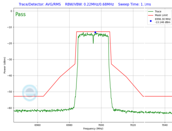
Plot 7-1512. LPI In-Band Emission Plot SDM Diversity Antenna WF7 (20MHz 802.11ax RU242 (UNII Band 8) – Ch. 209)
