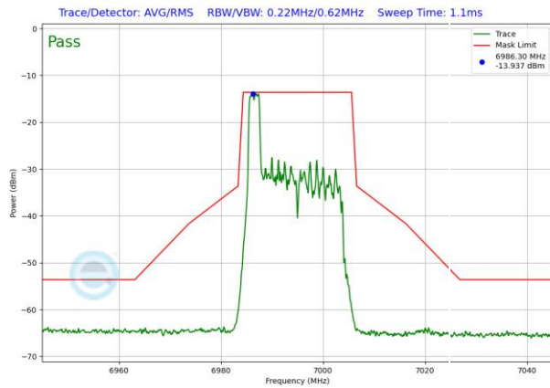
Plot 7-1505. LPI In-Band Emission Plot SDM Diversity Antenna WF8 (20MHz 802.11ax RU26 (UNII Band 8) – Ch. 209)
