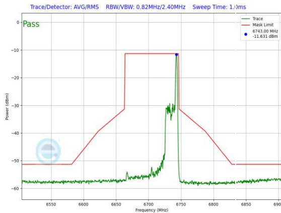
Plot 7-1494. LPI In-Band Emission Plot SDM Diversity Antenna WF7 (80MHz 802.11ax RU26 (UNII Band 7) – Ch. 151)
