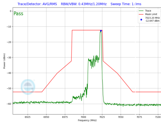
Plot 7-1518. LPI In-Band Emission Plot SDM Diversity Antenna WF7 (40MHz 802.11ax RU26 (UNII Band 8) – Ch. 211)
