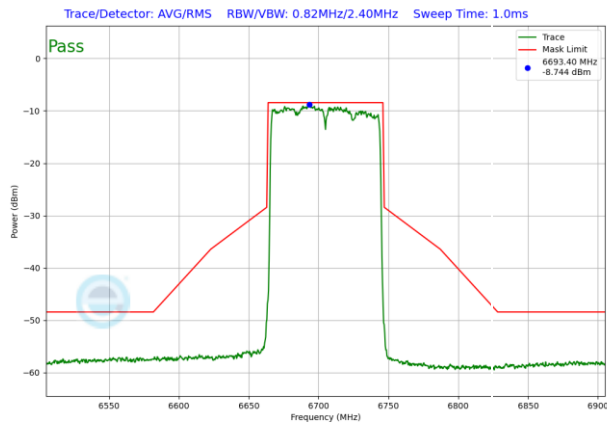
Plot 7-1495. LPI In-Band Emission Plot SDM Diversity Antenna WF8 (80MHz 802.11ax RU996 (UNII Band 7) – Ch. 151)
