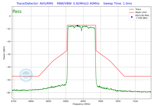
Plot 7-1527. LPI In-Band Emission Plot SDM Diversity Antenna WF8 (80MHz 802.11ax RU996 (UNII Band 8) – Ch. 199)
