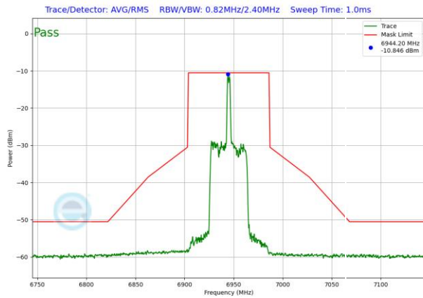
Plot 7-1523. LPI In-Band Emission Plot SDM Diversity Antenna WF8 (80MHz 802.11ax RU26 (UNII Band 8) – Ch. 199)
