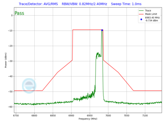
Plot 7-1526. LPI In-Band Emission Plot SDM Diversity Antenna WF7 (80MHz 802.11ax RU26 (UNII Band 8) – Ch. 199)
