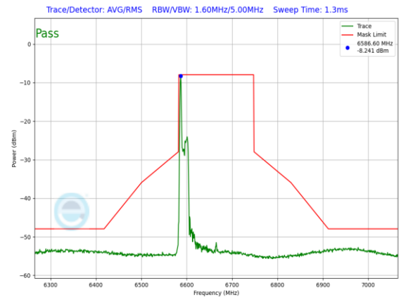
Plot 7-1498. LPI In-Band Emission Plot SDM Diversity Antenna WF7 (160MHz 802.11ax RU26 (UNII Band 7) – Ch. 143)
