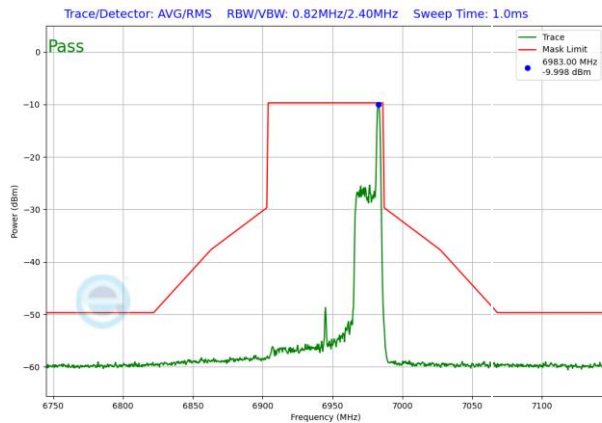
Plot 7-1525. LPI In-Band Emission Plot SDM Diversity Antenna WF8 (80MHz 802.11ax RU26 (UNII Band 8) – Ch. 199)
