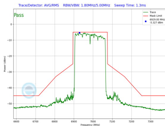
Plot 7-1536. LPI In-Band Emission Plot SDM Diversity Antenna WF7 (160MHz 802.11ax RU996x2 (UNII Band 8) – Ch. 207)
