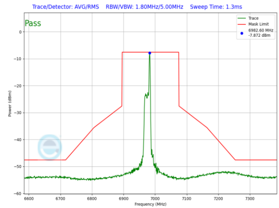
Plot 7-1532. LPI In-Band Emission Plot SDM Diversity Antenna WF7 (160MHz 802.11ax RU26 (UNII Band 8) – Ch. 207)
