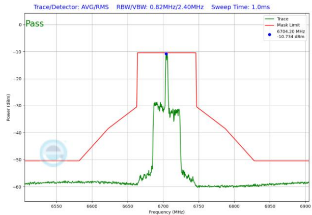
Plot 7-1491. LPI In-Band Emission Plot SDM Diversity Antenna WF8 (80MHz 802.11ax RU26 (UNII Band 7) – Ch. 151)
