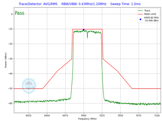
Plot 7-1520. LPI In-Band Emission Plot SDM Diversity Antenna WF7 (40MHz 802.11ax RU484 (UNII Band 8) – Ch. 211)
