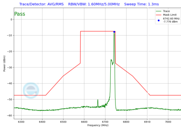
Plot 7-1501. LPI In-Band Emission Plot SDM Diversity Antenna WF8 (160MHz 802.11ax RU26 (UNII Band 7) – Ch. 143)
