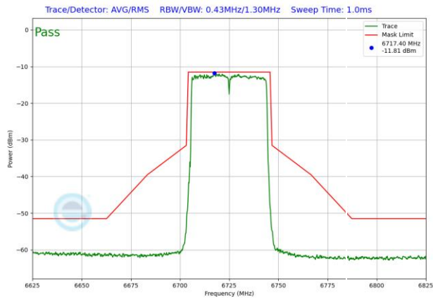
Plot 7-1487. LPI In-Band Emission Plot SDM Diversity Antenna WF8 (40MHz 802.11ax RU484 (UNII Band 7) – Ch. 155)
