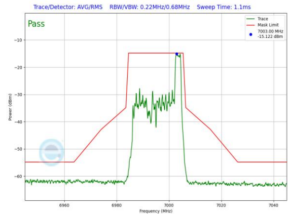
Plot 7-1510. LPI In-Band Emission Plot SDM Diversity Antenna WF7 (20MHz 802.11ax RU26 (UNII Band 8) – Ch. 209)
