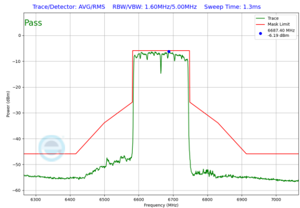
Plot 7-1503. LPI In-Band Emission Plot SDM Diversity Antenna WF8 (160MHz 802.11ax RU996x2 (UNII Band 7) – Ch. 143)
