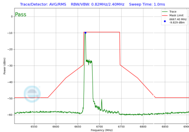
Plot 7-1489. LPI In-Band Emission Plot SDM Diversity Antenna WF8 (80MHz 802.11ax RU26 (UNII Band 7) – Ch. 151)
