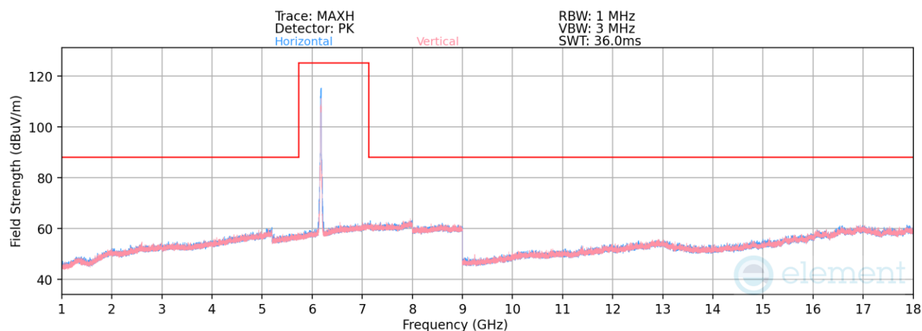
Plot 7-1586. Radiated Spurious Emissions above 1GHz Antenna WF5B (802.11ax – Ch. 45 – RU242)
