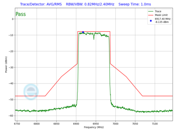
Plot 7-1528. LPI In-Band Emission Plot SDM Diversity Antenna WF7 (80MHz 802.11ax RU996 (UNII Band 8) – Ch. 199)
