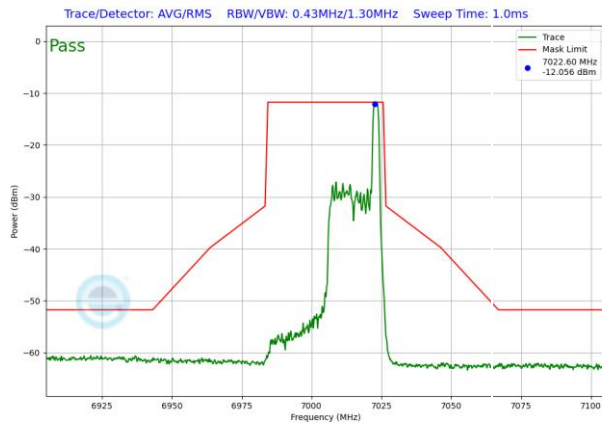
Plot 7-1517. LPI In-Band Emission Plot SDM Diversity Antenna WF8 (40MHz 802.11ax RU26 (UNII Band 8) – Ch. 211)
