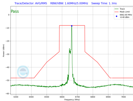
Plot 7-1500. LPI In-Band Emission Plot SDM Diversity Antenna WF7 (160MHz 802.11ax RU26 (UNII Band 7) – Ch. 143)
