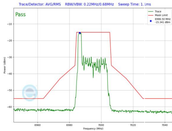
Plot 7-1506. LPI In-Band Emission Plot SDM Diversity Antenna WF7 (20MHz 802.11ax RU26 (UNII Band 8) – Ch. 209)
