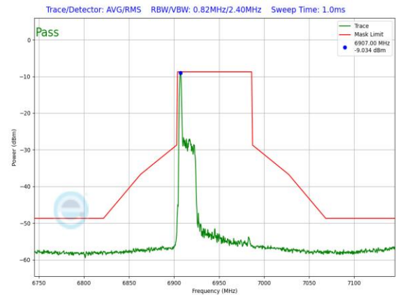
Plot 7-1522. LPI In-Band Emission Plot SDM Diversity Antenna WF7 (80MHz 802.11ax RU26 (UNII Band 8) – Ch. 199)
