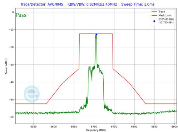
Plot 7-1492. LPI In-Band Emission Plot SDM Diversity Antenna WF7 (80MHz 802.11ax RU26 (UNII Band 7) – Ch. 151)
