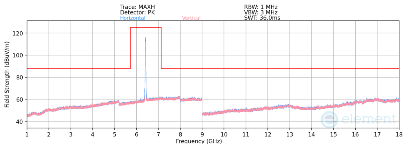
Plot 7-1587. Radiated Spurious Emissions above 1GHz Antenna WF5B (802.11ax – Ch. 93 – RU242)
