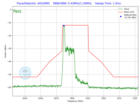
Plot 7-1514. LPI In-Band Emission Plot SDM Diversity Antenna WF7 (40MHz 802.11ax RU26 (UNII Band 8) – Ch. 211)
