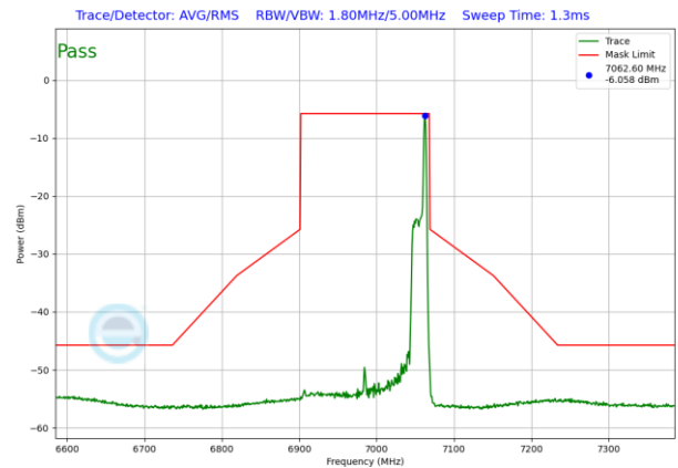
Plot 7-1533. LPI In-Band Emission Plot SDM Diversity Antenna WF8 (160MHz 802.11ax RU26 (UNII Band 8) – Ch. 207)
