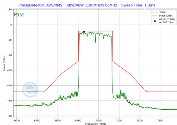
Plot 7-1535. LPI In-Band Emission Plot SDM Diversity Antenna WF8 (160MHz 802.11ax RU996x2 (UNII Band 8) – Ch. 207)
