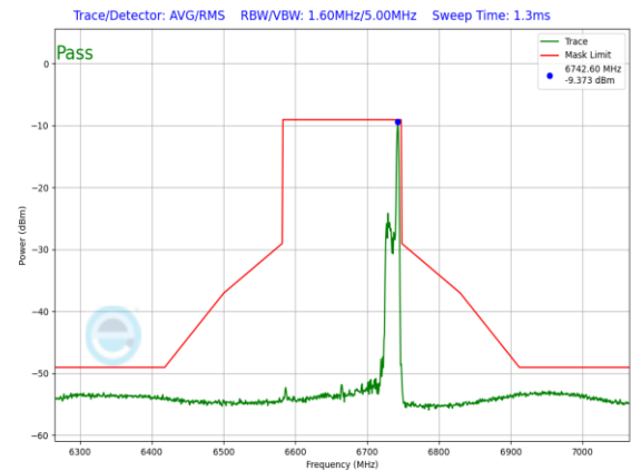
Plot 7-1502. LPI In-Band Emission Plot SDM Diversity Antenna WF7 (160MHz 802.11ax RU26 (UNII Band 7) – Ch. 143)
