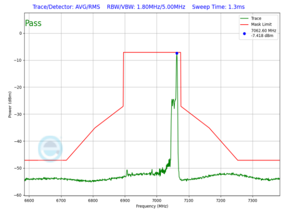
Plot 7-1534. LPI In-Band Emission Plot SDM Diversity Antenna WF7 (160MHz 802.11ax RU26 (UNII Band 8) – Ch. 207)
