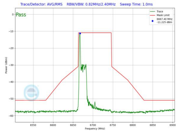
Plot 7-1490. LPI In-Band Emission Plot SDM Diversity Antenna WF7 (80MHz 802.11ax RU26 (UNII Band 7) – Ch. 151)
