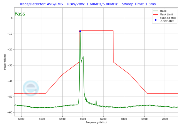
Plot 7-1497. LPI In-Band Emission Plot SDM Diversity Antenna WF8 (160MHz 802.11ax RU26 (UNII Band 7) – Ch. 143)
