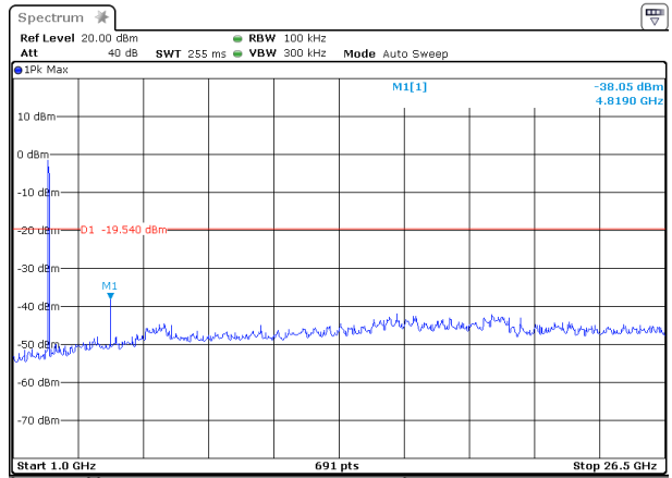
8-DPSK on channel 00
