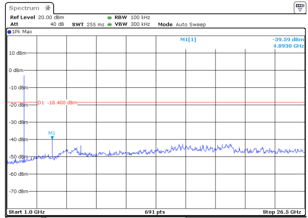
8-DPSK on channel 39
