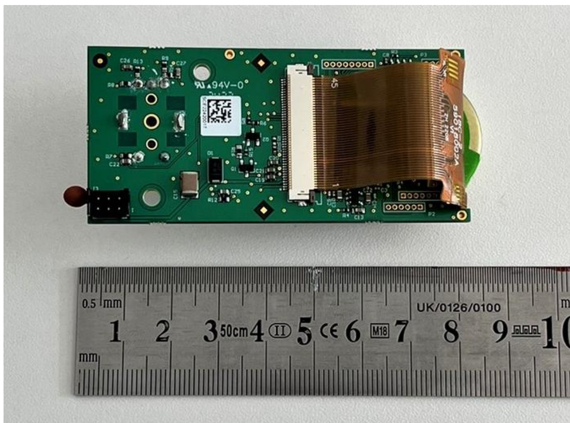
Receiver Station: LCD Unit PCB Top View
