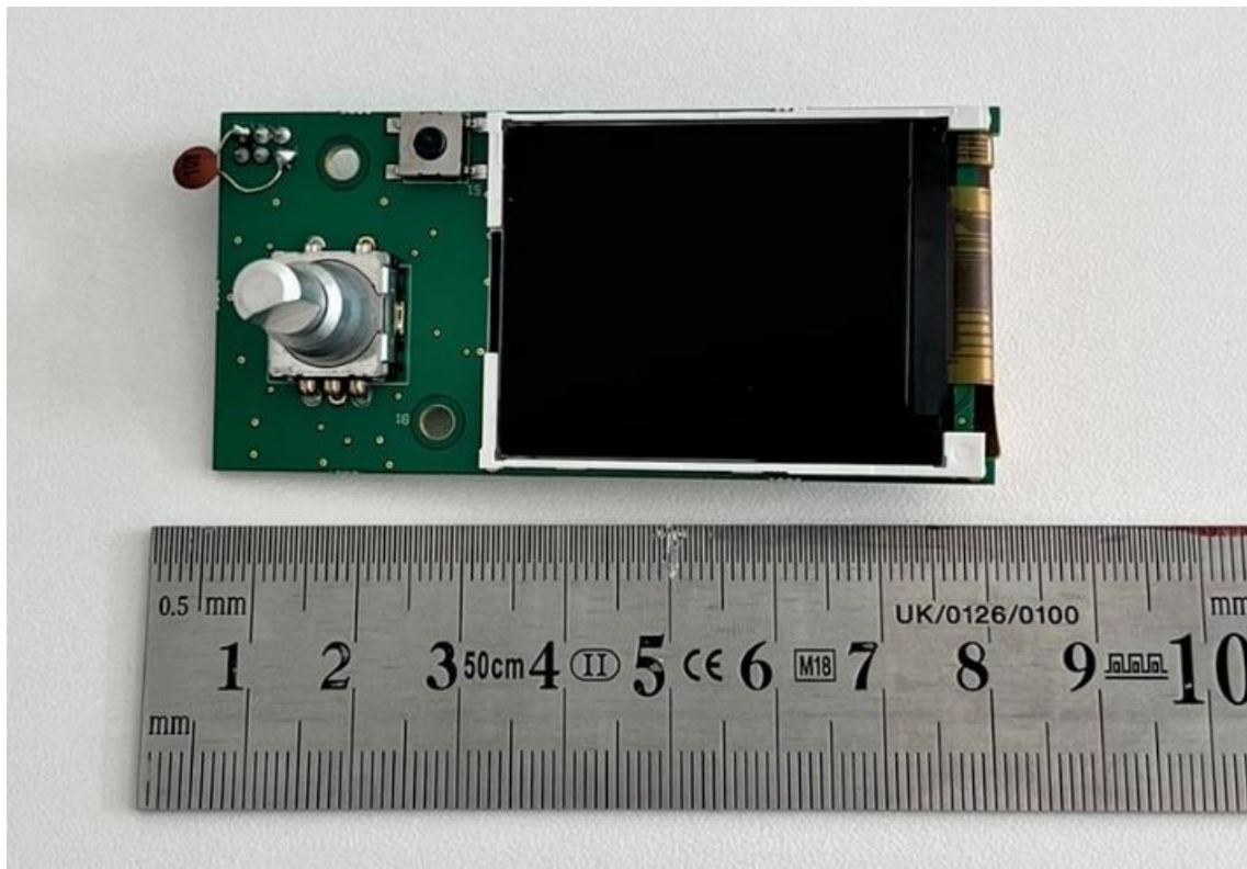
Receiver Station: LCD Unit PCB Bottom View
