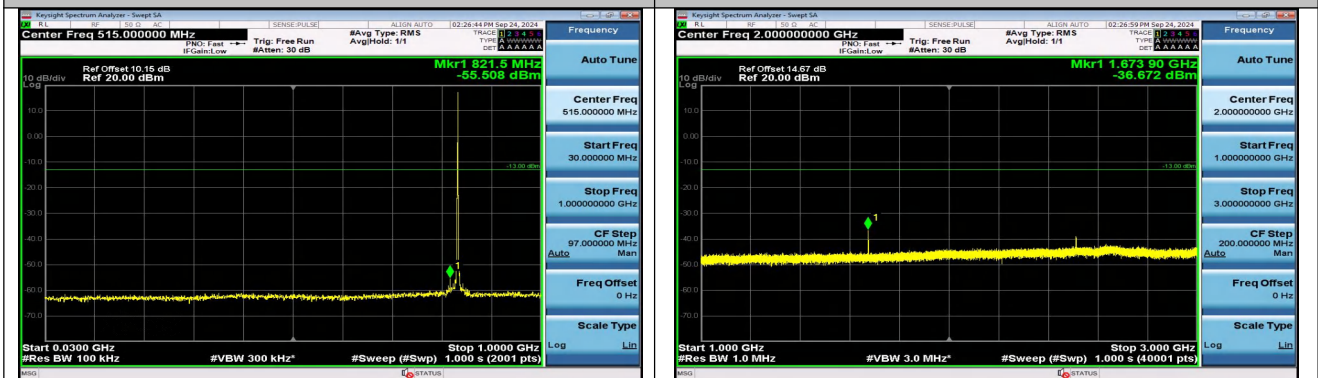
Band5_1.4MHz_QPSK_20525_1RB#5_30~1000_30~100
