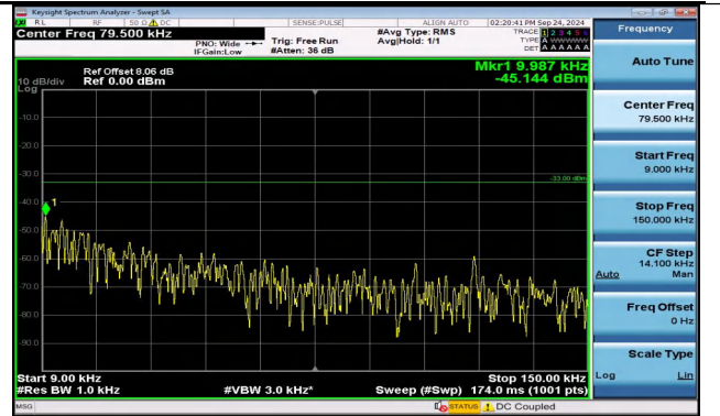
Band5_1.4MHz_16QAM_20407_1RB#0_0.009~0.15_0.009 ~0.15
