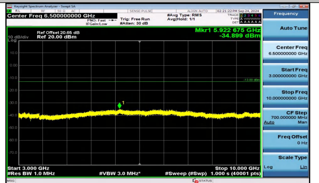
Band5_1.4MHz_16QAM_20407_1RB#0_3000~10000_300 0~10000
