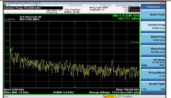
Band5_1.4MHz_16QAM_20407_6RB#0_0.009~0.15_0.009 ~0.15
