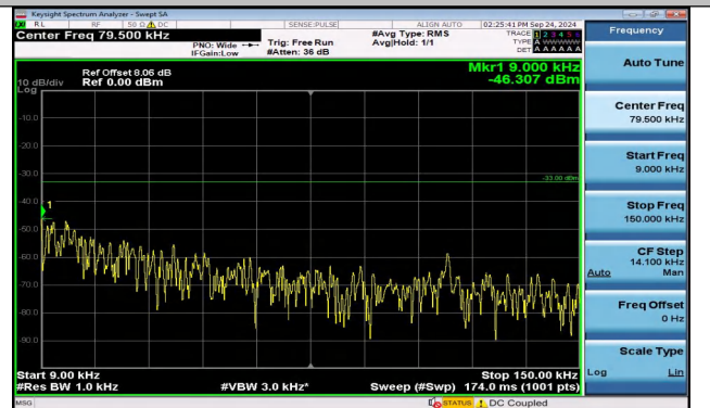
Band5_1.4MHz_16QAM_20525_1RB#0_0.009~0.15_0.009 ~0.15
