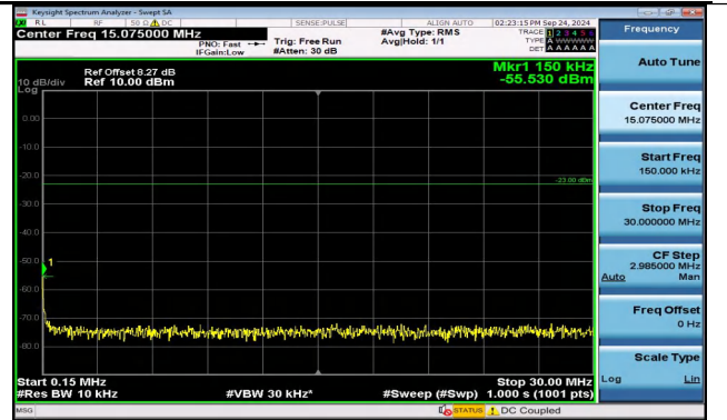
Band5_1.4MHz_QPSK_20407_6RB#0_0.15~30_0.15~30
