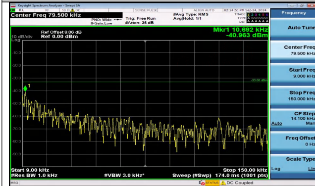
Band5_1.4MHz_QPSK_20525_1RB#0_0.009~0.15_0.009 ~0.15
