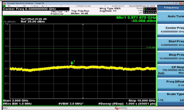
Band5_1.4MHz_QPSK_20407_6RB#0_3000~10000_300 0~10000
