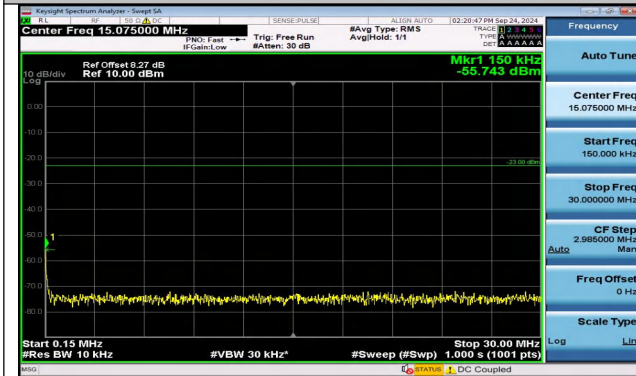
Band5_1.4MHz_16QAM_20407_1RB#0_0.15~30_0.15~3 0
