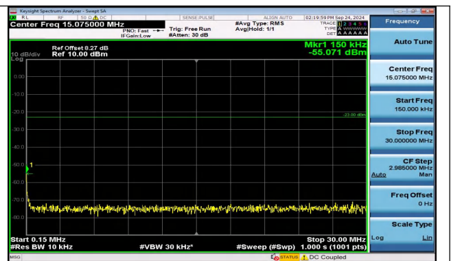
Band5_1.4MHz_QPSK_20407_1RB#0_0.15~30_0.15~30
