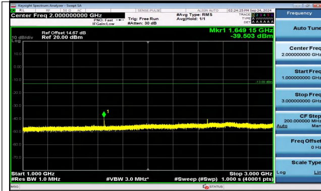
Band5_1.4MHz_16QAM_20407_6RB#0_1000~3000_100 0~3000
