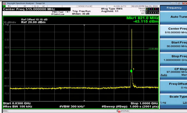
Band5_1.4MHz_QPSK_20407_6RB#0_30~1000_30~100 0
