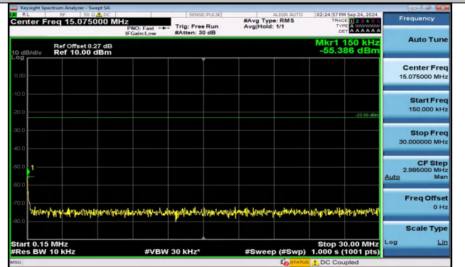
Band5_1.4MHz_QPSK_20525_1RB#0_0.15~30_0.15~30
