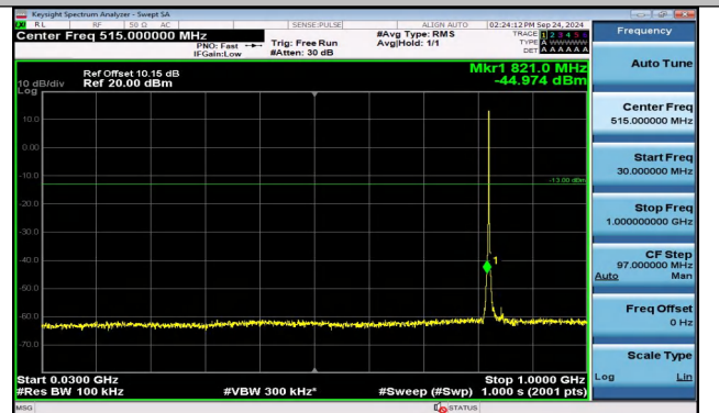
Band5_1.4MHz_16QAM_20407_6RB#0_30~1000_30~100 0
