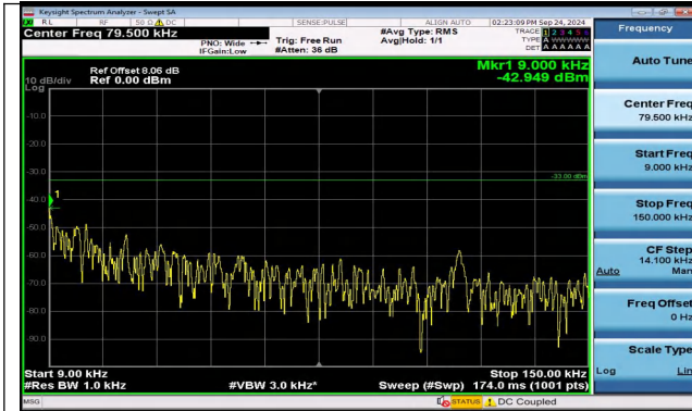
Band5_1.4MHz_QPSK_20407_6RB#0_0.009~0.15_0.009 ~0.15
