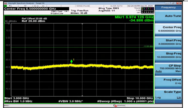
Band5_1.4MHz_16QAM_20407_6RB#0_3000~10000_300 0~10000
