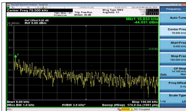
Band5_1.4MHz_QPSK_20407_1RB#0_0.009~0.15_0.009~0.15
