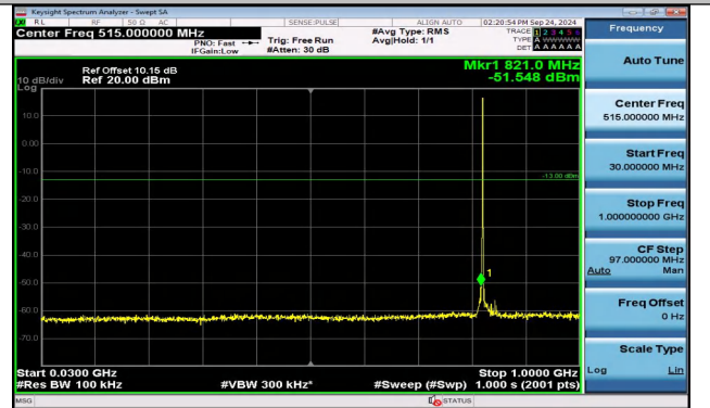
Band5_1.4MHz_16QAM_20407_1RB#0_30~1000_30~100 0
