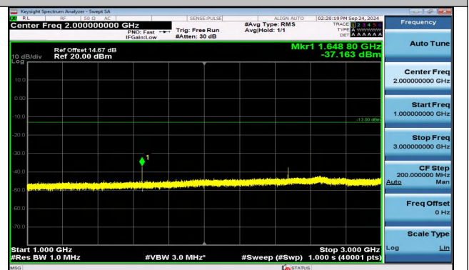
Band5_1.4MHz_QPSK_20407_1RB#0_1000~3000_1000~3000
