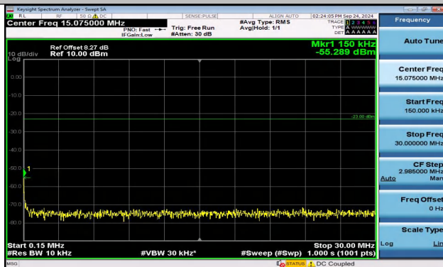
Band5_1.4MHz_16QAM_20407_6RB#0_0.15~30_0.15~3 0
