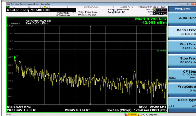
Band5_1.4MHz_QPSK_20407_1RB#5_0.009~0.15_0.009 ~0.15
