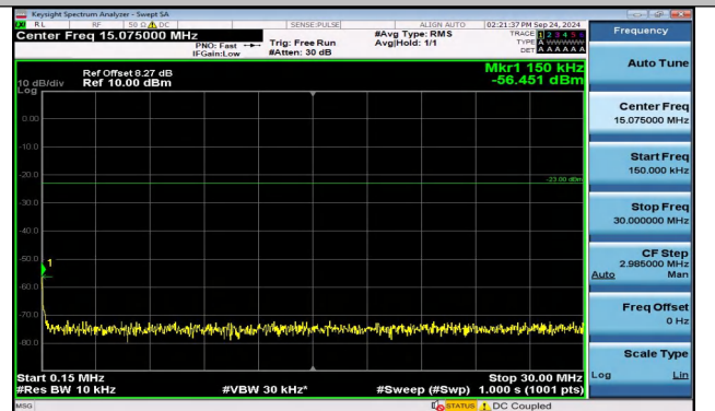
Band5_1.4MHz_QPSK_20407_1RB#5_0.15~30_0.15~30
