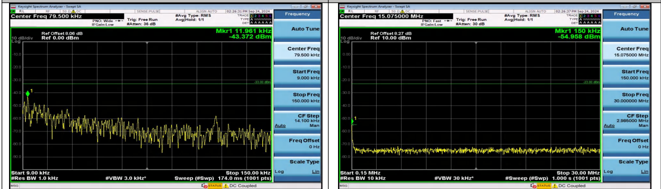
Band5_1.4MHz_QPSK_20525_1RB#5_0.009~0.15_0.009
