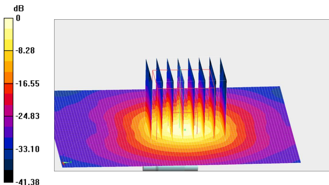
Fig.B.4 validation 5750 MHz 100mW
