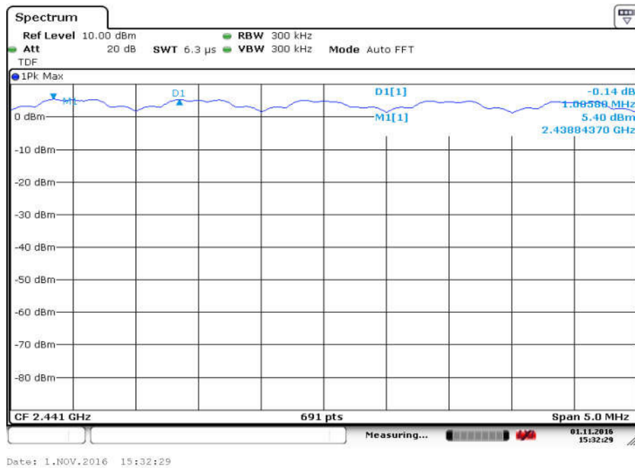
Fig. 105 Carrier Frequency Separation ( \pi/4 DQPSK, Ch39)
