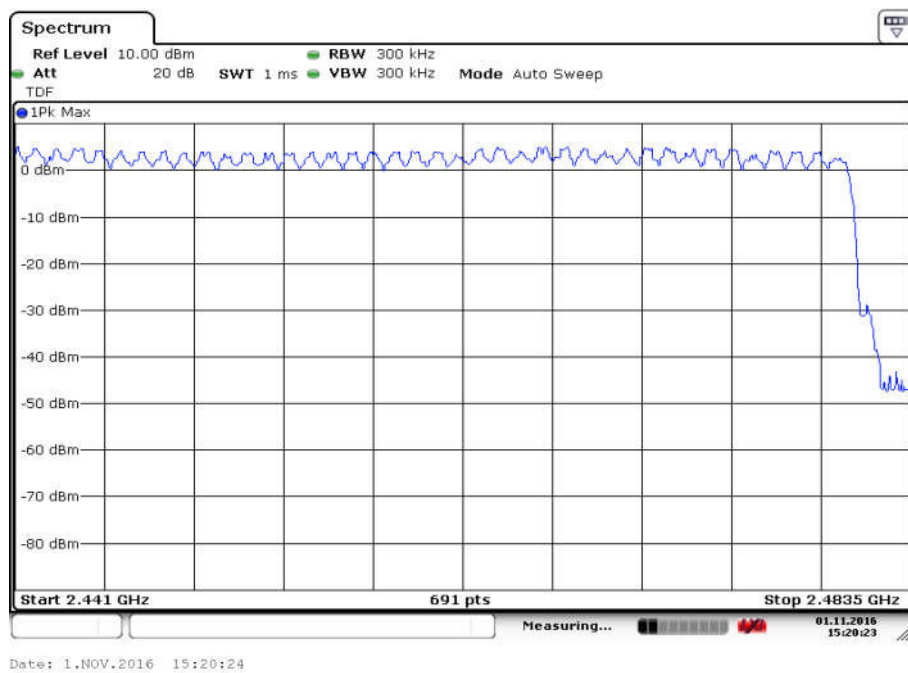
Fig. 101 Hopping channel ch39~78 ( \pi/4 DQPSK, Ch39)
