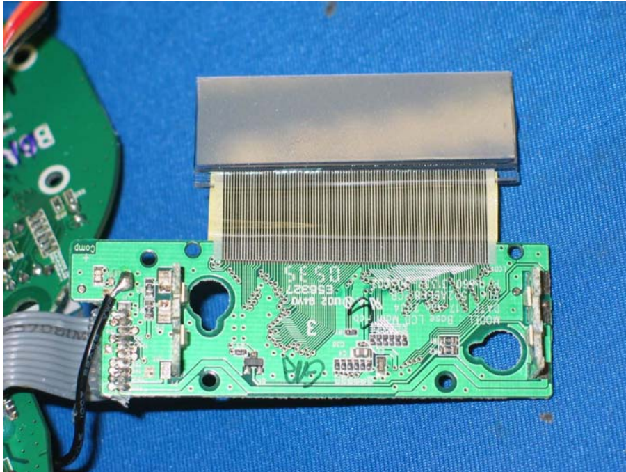
LCD display front side (View 2)
