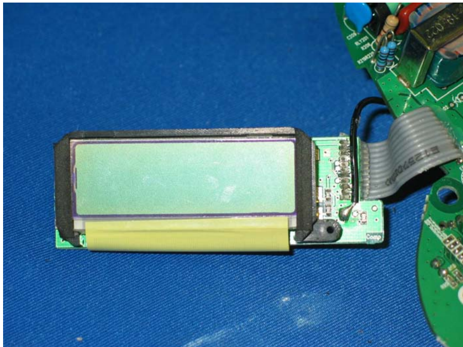
LCD display front side (View 1)
