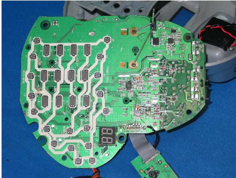
Base Unit Main PCB keypad side
