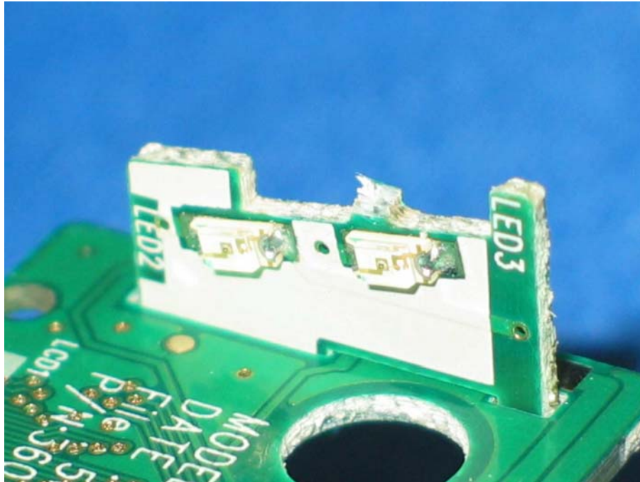
LCD display front side (View 4)
