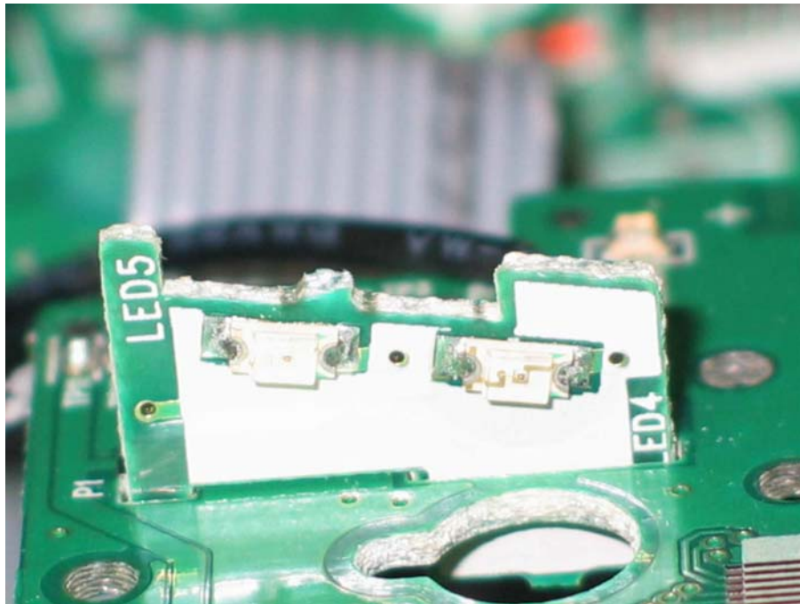
LCD display front side (View 6)
