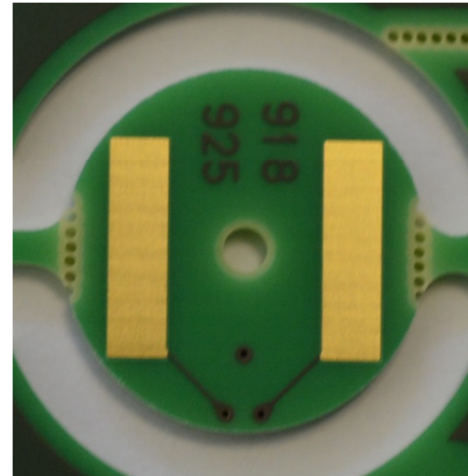
Antenna Top
