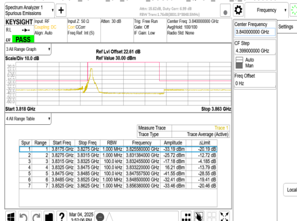
Band77-Part27_15MHz_CP_OFDM_SCS30kHz_QPSK_RB1_0_CH656000
