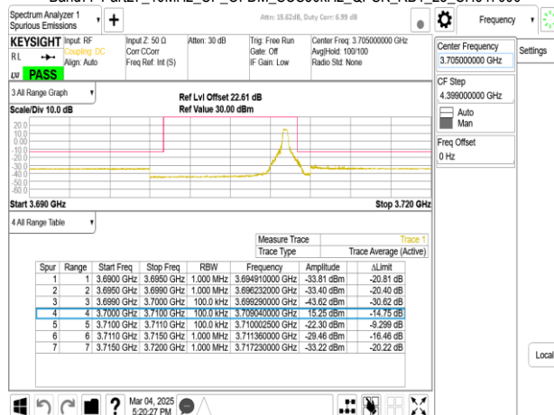
Band77-Part27_10MHz_CP_OFDM_SCS30kHz_QPSK_RB24_0_CH647000
