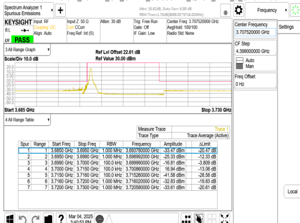
Band77-Part27_15MHz_CP_OFDM_SCS30kHz_QPSK_RB1_0_CH647168
