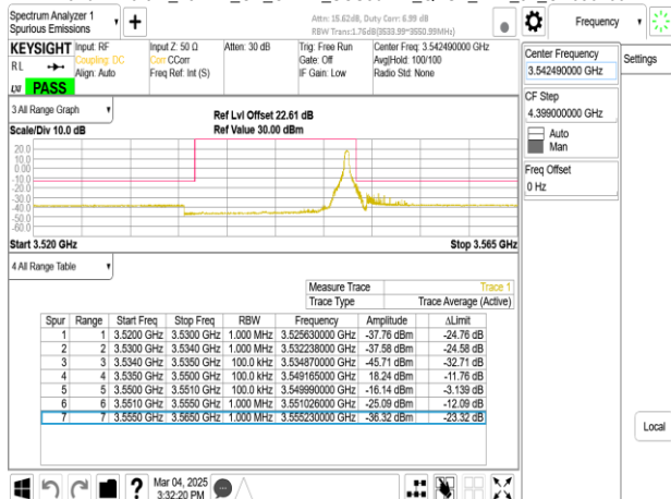
Band77-Part27_15MHz_CP_OFDM_SCS30kHz_QPSK_RB38_0_CH636166
