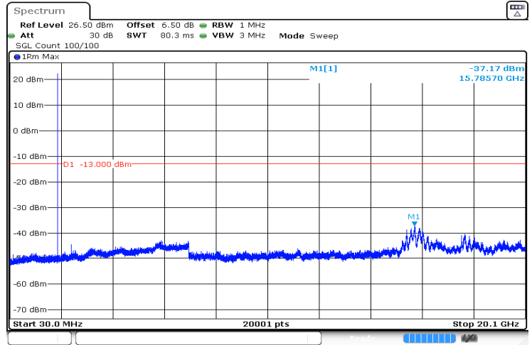
1.4MHz_Mid_QPSK_6@0 -37.17 dBm
