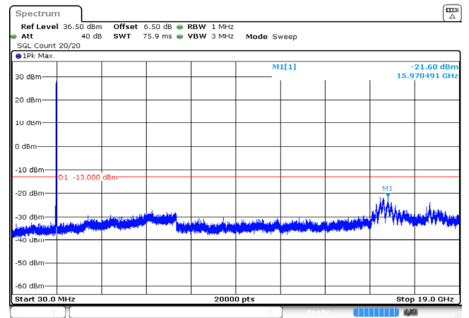
20MHz_High_QPSK_1@0 -21.60dBm
