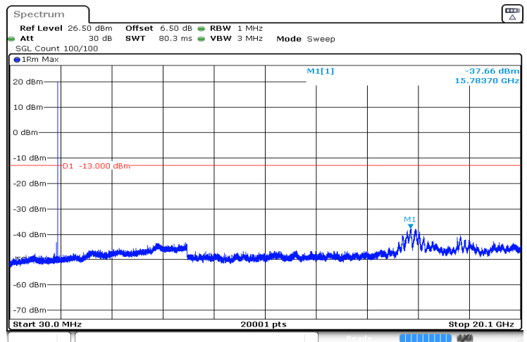
3MHz_High_QPSK_15@0 -37.66 dBm
