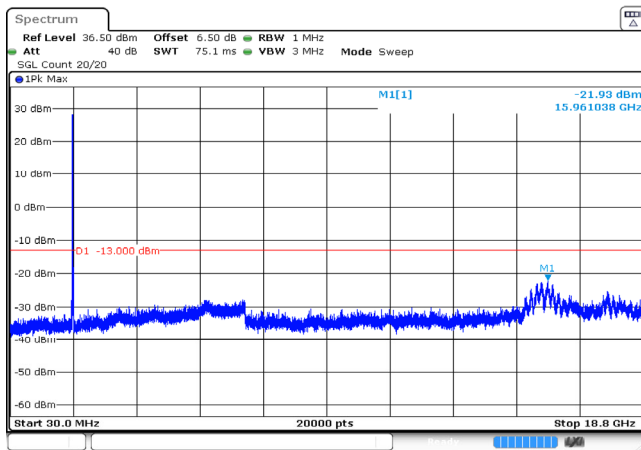
20MHz_Middle_QPSK_1@0 -21.93dBm
