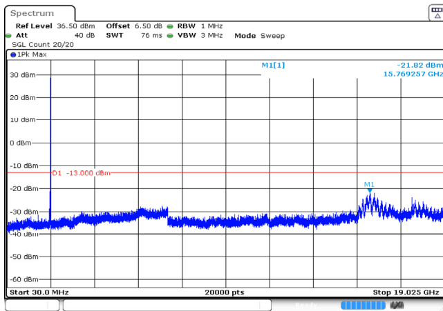
15MHz_High_QPSK_1@0 -21.82dBm
