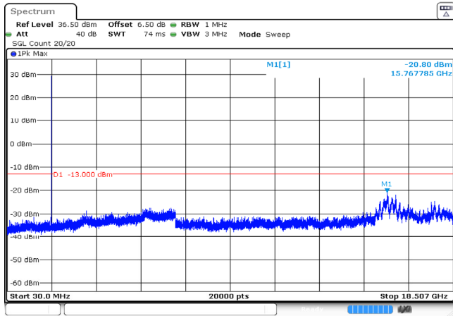
1.4MHz_Low_QPSK_1@0 -20.80dBm
