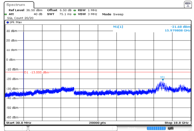
1.4MHz_Middle_QPSK_1@0 -21.68dBm
