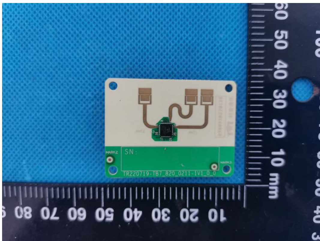
24GHz Antenna
