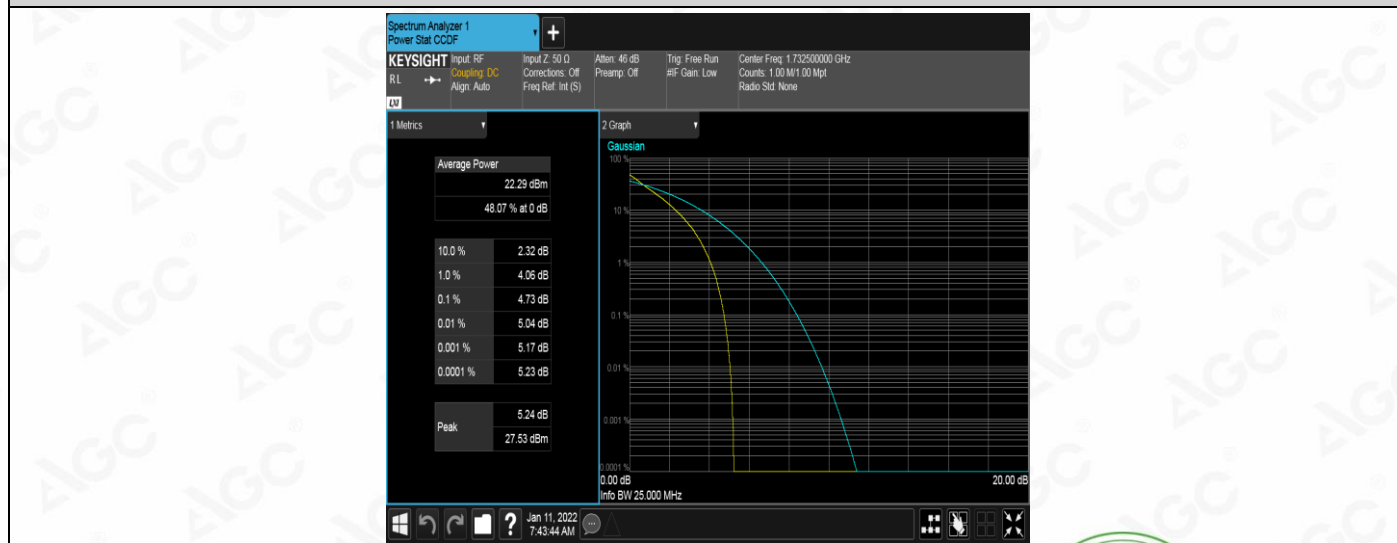
Band4-10MHz-QPSK-20175-50RB#0
