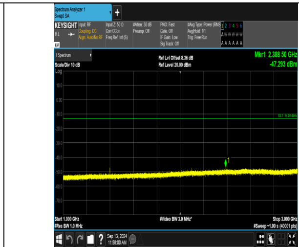
Band12_3MHz_QPSK_23025_1RB#0_1000~3000_1000~3000
