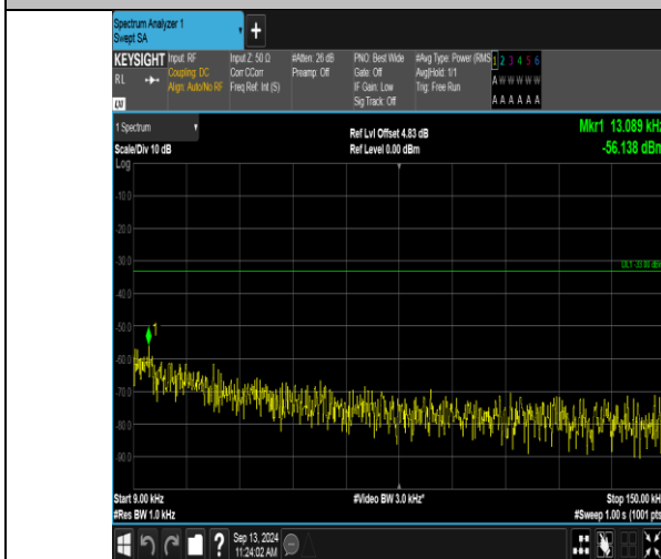
Band12_1.4MHz_QPSK_23173_1RB#0_0.009~0.15_0.009~0.15
