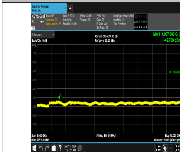
Band12_1.4MHz_QPSK_23173_6RB#0_3000~10000_3000~10000
