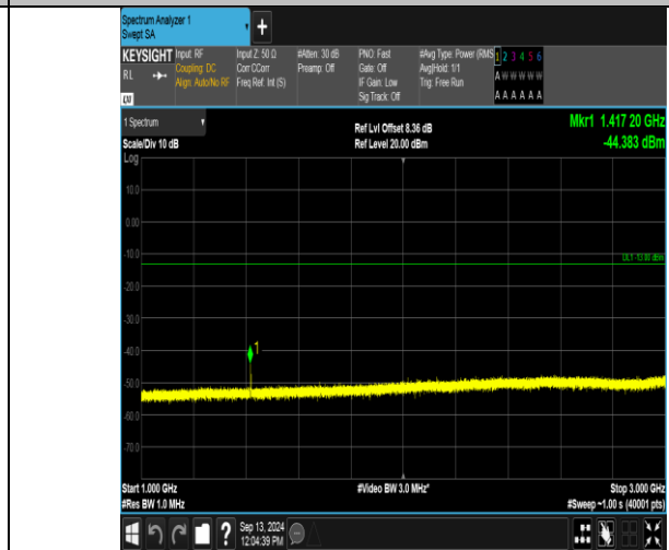
Band12_3MHz_QPSK_23095_1RB#14_1000~3000_1000~3000
