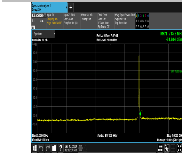
Band12_3MHz_QPSK_23095_15RB#0_30~1000_30~1000
