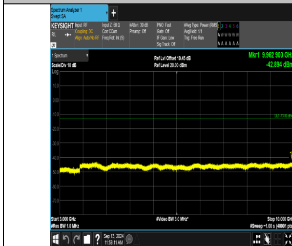
Band12_3MHz_QPSK_23025_1RB#0_3000~10000_3000~10000
