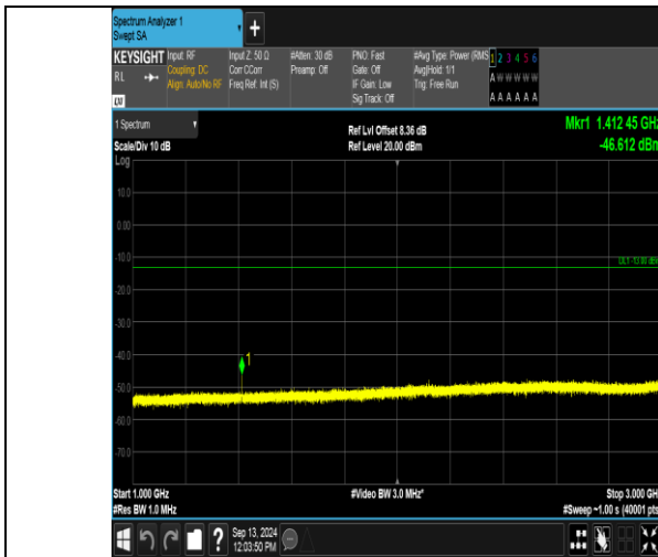
Band12_3MHz_16QAM_23095_1RB#0_1000~3000_1000~3000
