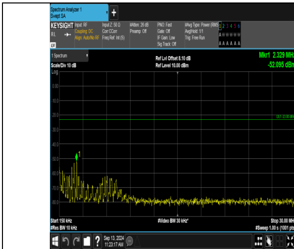
Band12_1.4MHz_16QAM_23095_6RB#0_0.15~30_0.15~30
