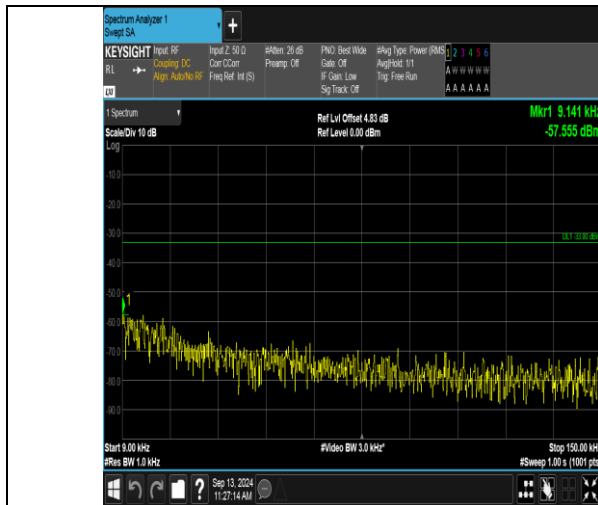
Band12_1.4MHz_QPSK_23173_6RB#0_0.009~0.15_0.009~0.15
