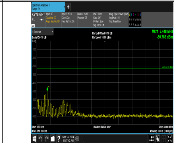
Band12_3MHz_QPSK_23025_1RB#0_0.15~30_0.15~30
