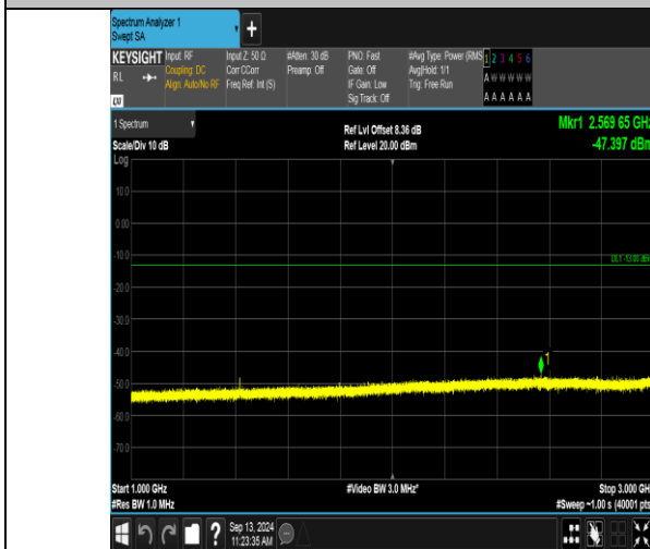
Band12_1.4MHz_16QAM_23095_6RB#0_1000~3000_1000~3000
