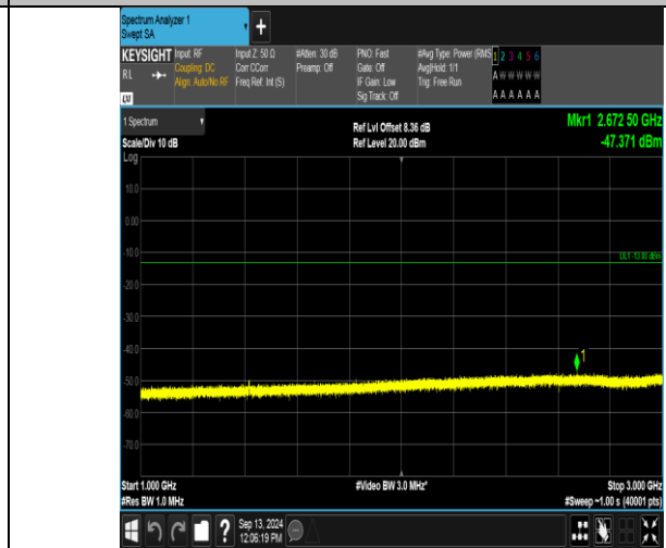
Band12_3MHz_QPSK_23095_15RB#0_1000~3000_1000~3000
