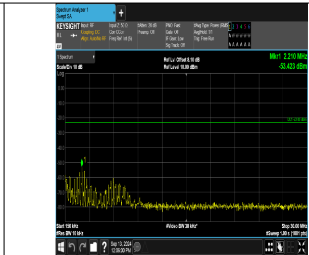
Band12_3MHz_QPSK_23095_15RB#0_0.15~30_0.15~30
