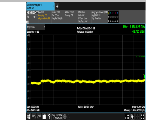
Band12_1.4MHz_16QAM_23095_6RB#0_3000~10000_3000~10000
