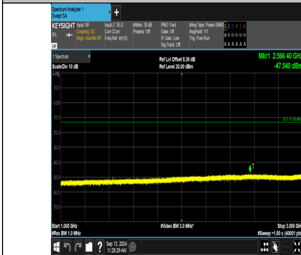
Band12_1.4MHz_16QAM_23173_6RB#0_1000~3000_1000~3000
