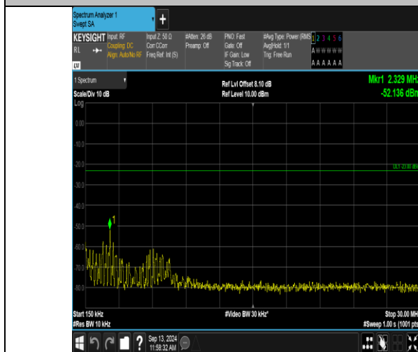
Band12_3MHz_16QAM_23025_1RB#0_0.15~30_0.15~30
