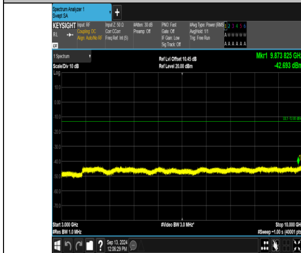
Band12_3MHz_QPSK_23095_15RB#0_3000~10000_3000~10000
