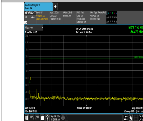
Band12_1.4MHz_16QAM_23173_1RB#0_0.15~30_0.15~30
