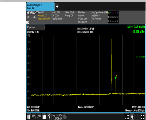
Band12_1.4MHz_16QAM_23173_1RB#0_30~1000_30~1000
