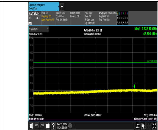
Band12_1.4MHz_QPSK_23173_1RB#0_1000~3000_1000~3000
