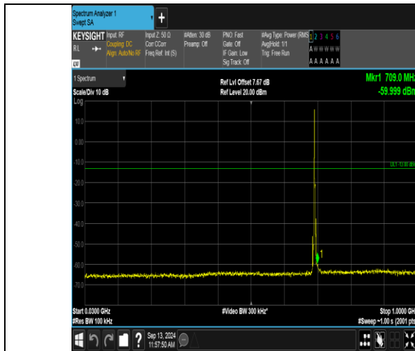
Band12_3MHz_QPSK_23025_1RB#0_30~1000_30~1000
