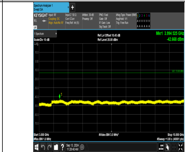
Band12_1.4MHz_16QAM_23173_6RB#0_3000~10000_3000~10000
