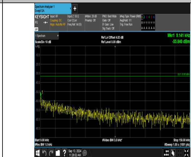
Band12_1.4MHz_16QAM_23173_6RB#0_0.009~0.15_0.009~0.15
