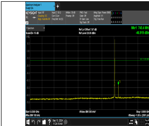
Band12_1.4MHz_QPSK_23173_1RB#0_30~1000_30~1000
