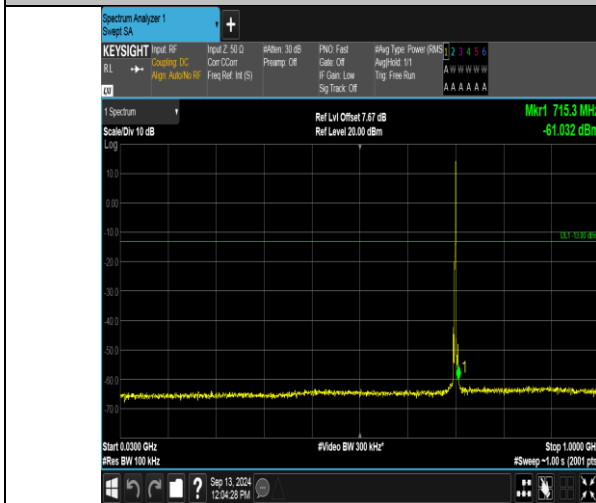
Band12_3MHz_QPSK_23095_1RB#14_30~1000_30~1000
