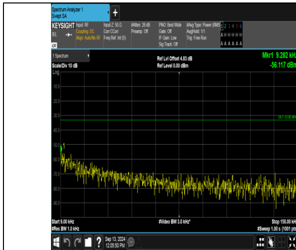
Band12_3MHz_QPSK_23095_15RB#0_0.009~0.15_0.009~0.15
