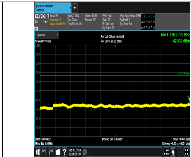
Band12_3MHz_16QAM_23095_1RB#0_3000~10000_3000~10000
