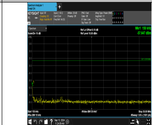
Band12_1.4MHz_QPSK_23173_1RB#0_0.15~30_0.15~30
