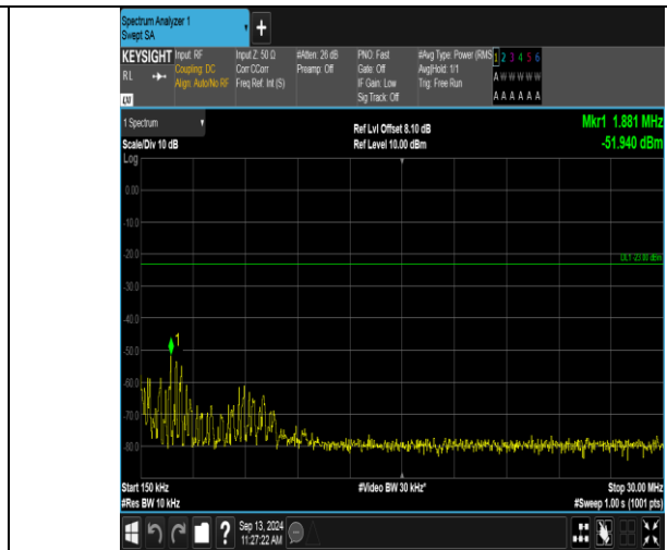
Band12_1.4MHz_QPSK_23173_6RB#0_0.15~30_0.15~30
