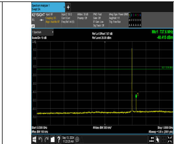
Band12_1.4MHz_16QAM_23095_6RB#0_30~1000_30~1000
