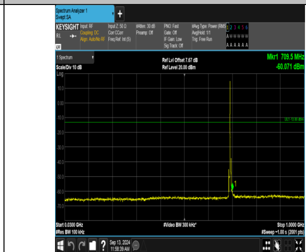
Band12_3MHz_16QAM_23025_1RB#0_30~1000_30~1000
