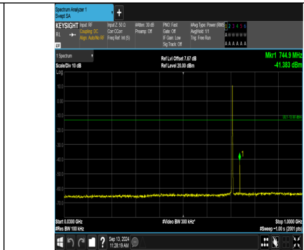
Band12_1.4MHz_16QAM_23173_6RB#0_30~1000_30~1000
