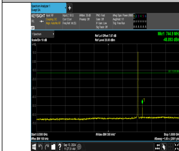
Band12_1.4MHz_QPSK_23173_6RB#0_30~1000_30~1000
