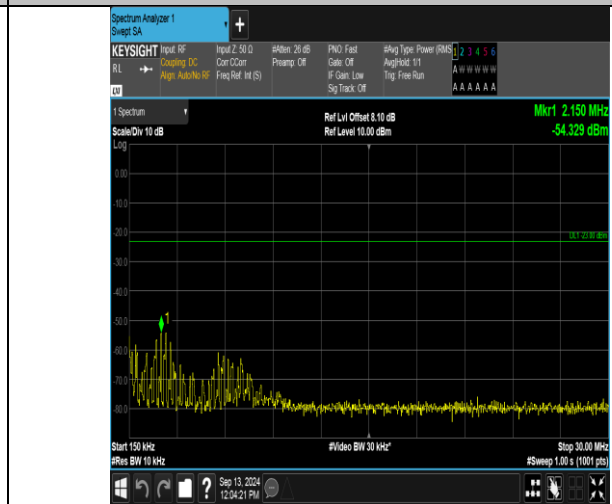
Band12_3MHz_QPSK_23095_1RB#14_0.15~30_0.15~30
