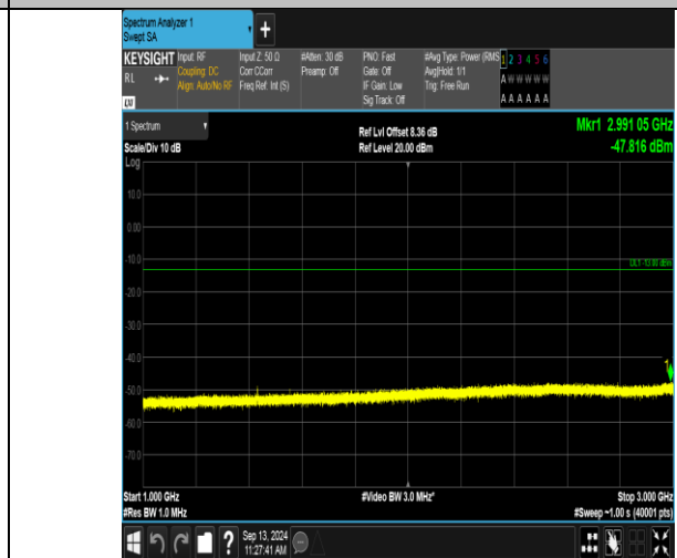
Band12_1.4MHz_QPSK_23173_6RB#0_1000~3000_1000~3000
