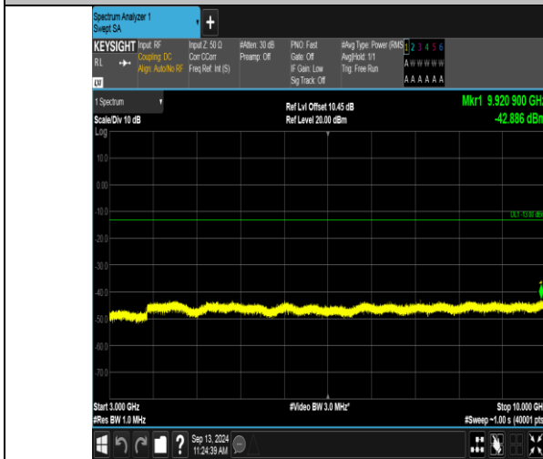
Band12_1.4MHz_QPSK_23173_1RB#0_3000~10000_3000~10000
