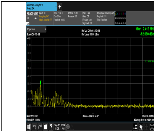
Band12_1.4MHz_16QAM_23173_6RB#0_0.15~30_0.15~30
