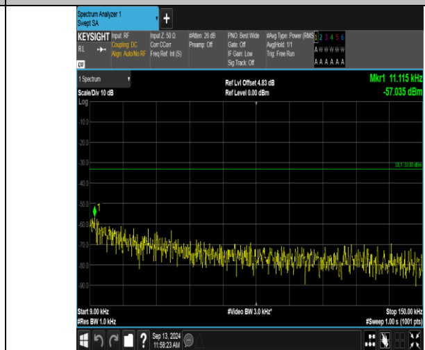
Band12_3MHz_16QAM_23025_1RB#0_0.009~0.15_0.009~0.15
