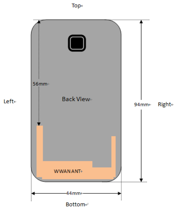
Fig.14.1 EUT Antenna Locations
