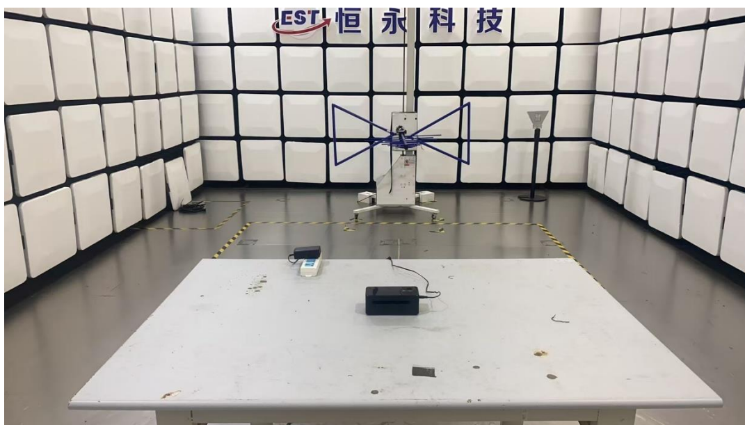
Radiated emission test: Below 1GHz
