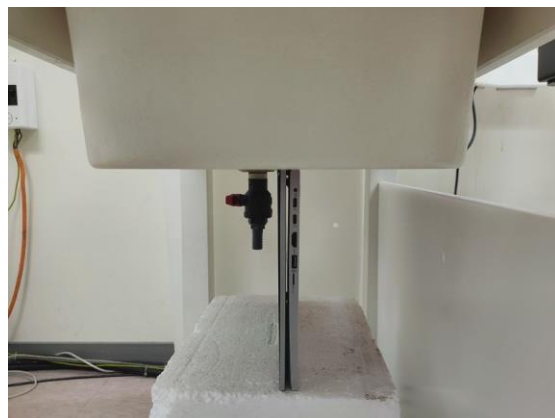
Fig.5 EUT Bottom side (TB mode) to flat phantom
