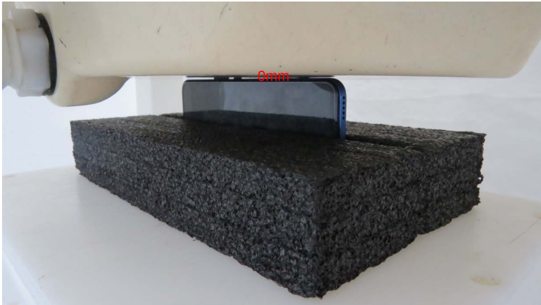
Picture 15: Right Side, the distance from handset to the bottom of the Phantom is 0mm
