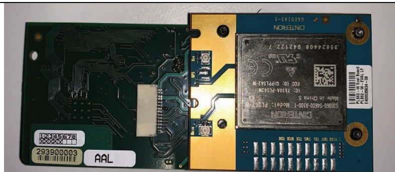
Top-side of main PCB
