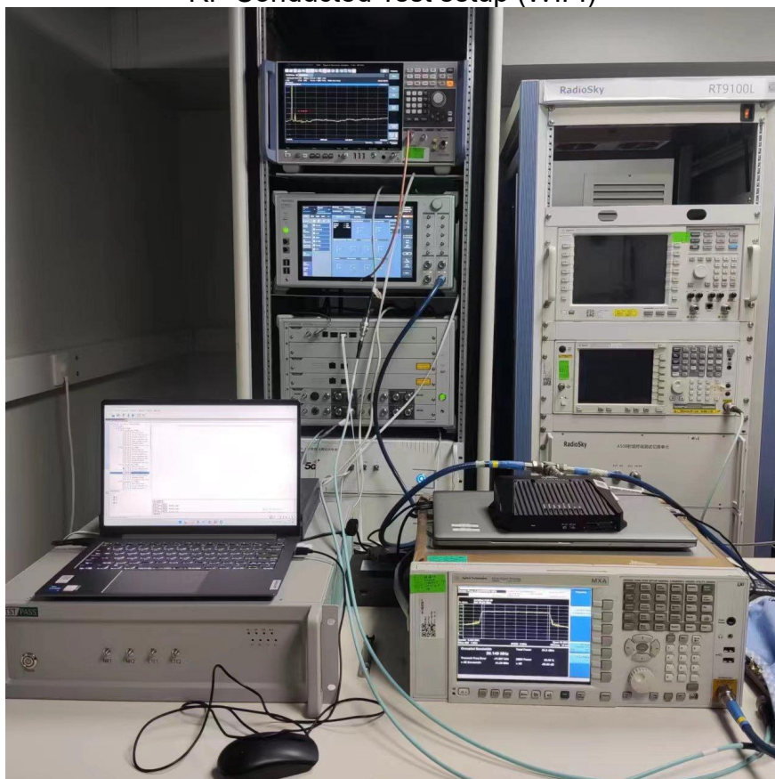
RF Conducted Test setup (LTE)
