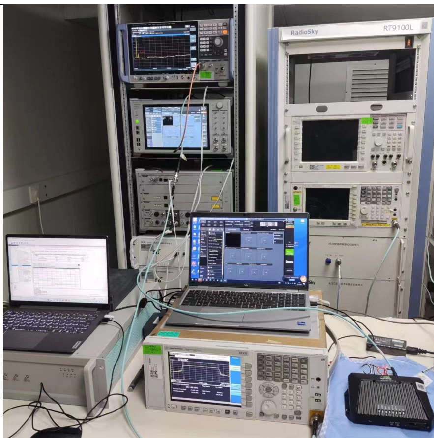
RF Conducted Test setup (NR)
