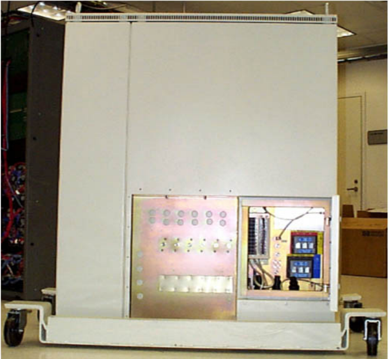
IHET5EG1 SC4812ET 1X/EVDO @ 800 MHz Rear View without Panel
