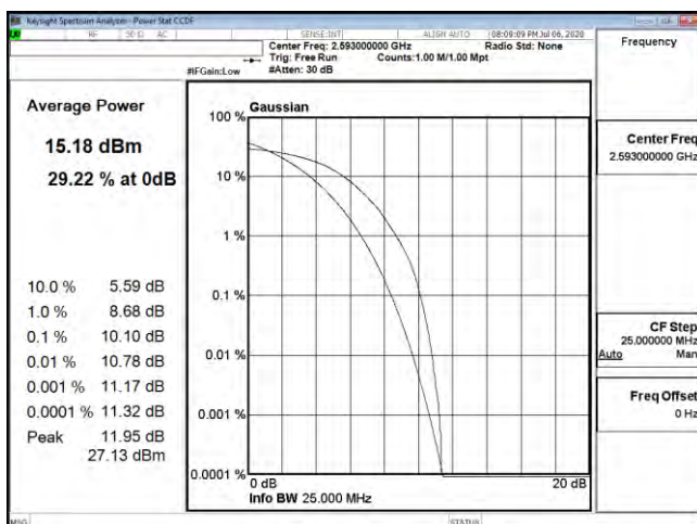
PTAR B41 20M CH40620 64QAM
