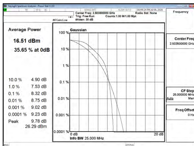
PTAR B41 15M CH39725 QPSK
