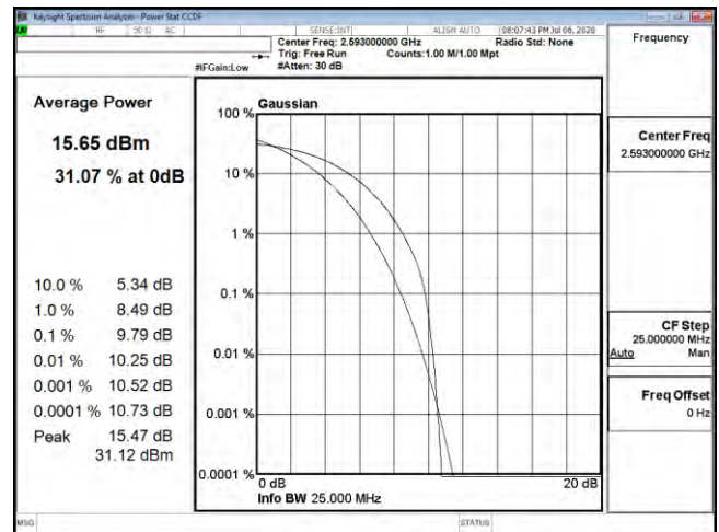
PTAR B41 15M CH40620 64QAM
