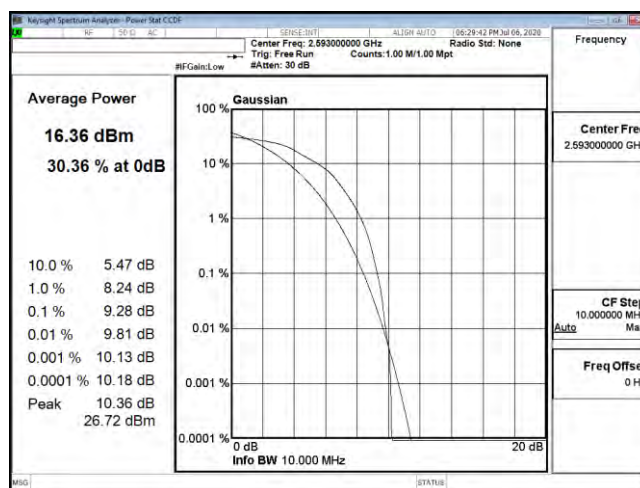
PTAR B41 10M CH40620 16QAM
