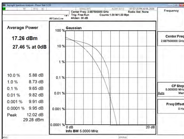
PTAR B41 5M CH41565 64QAM
