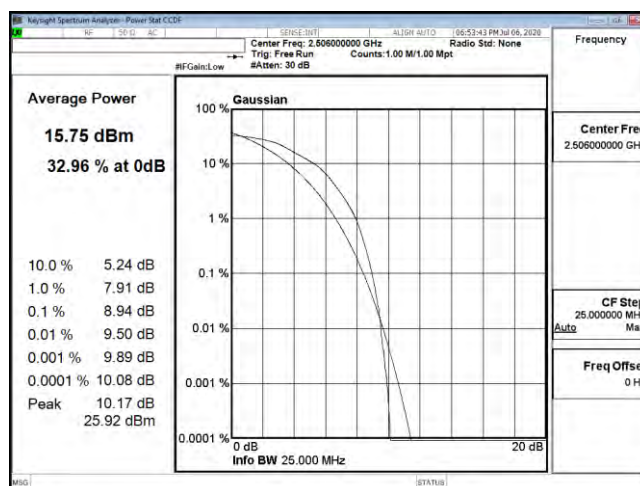
PTAR B41 20M CH39750 16QAM
