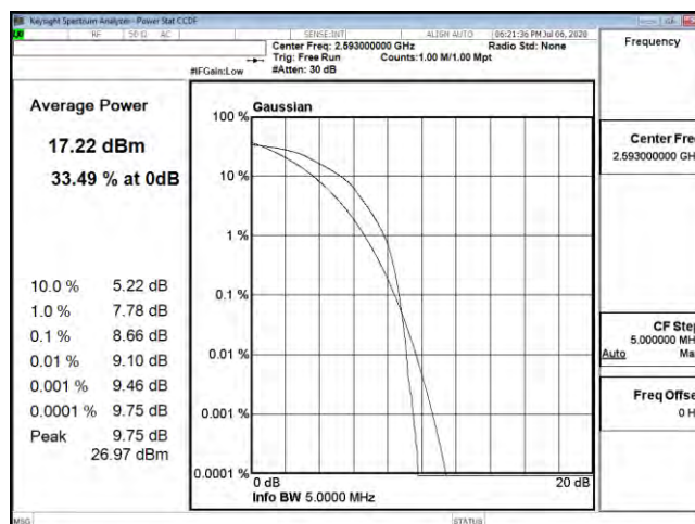
PTAR B41 5M CH40620 16QAM
