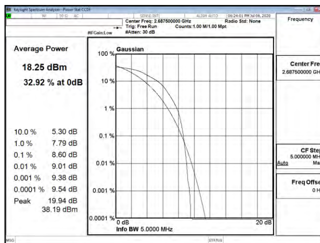
PTAR B41 5M CH41565 16QAM
