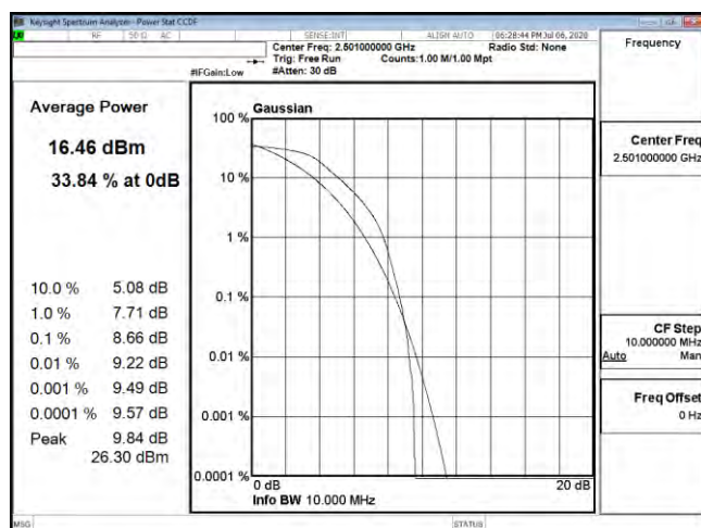
PTAR B41 10M CH39700 QPSK
