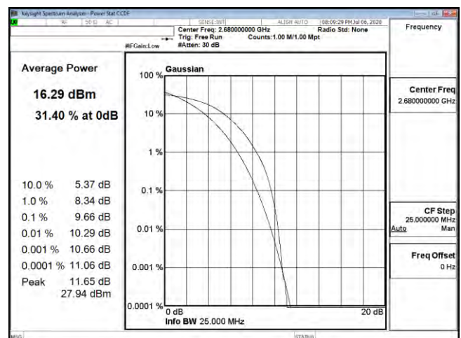
PTAR B41 20M CH41490 64QAM
