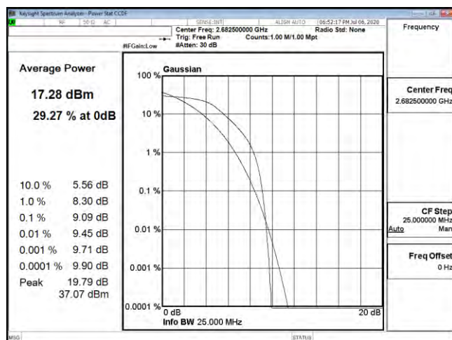
PTAR B41 15M CH41515 QPSK
