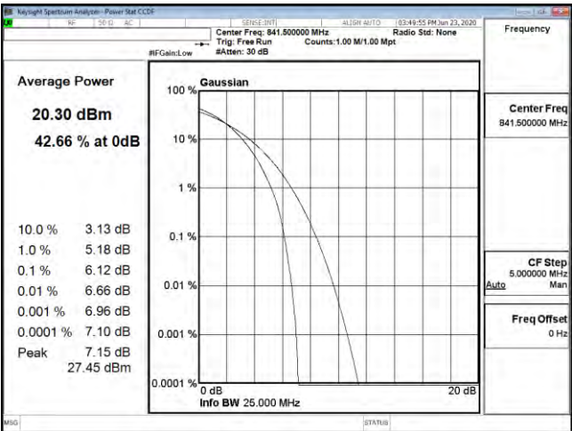
PTAR B26 15M CH26965 64QAM
