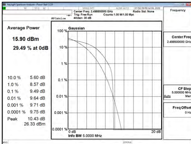
PTAR B41 5M CH39675 64QAM
