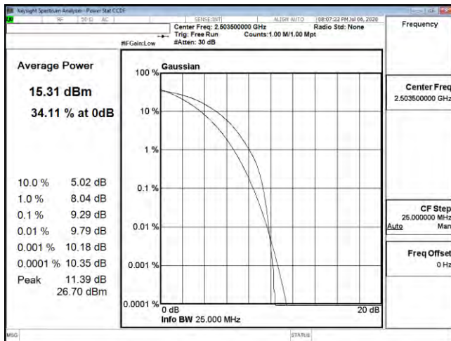
PTAR B41 15M CH39725 64QAM
