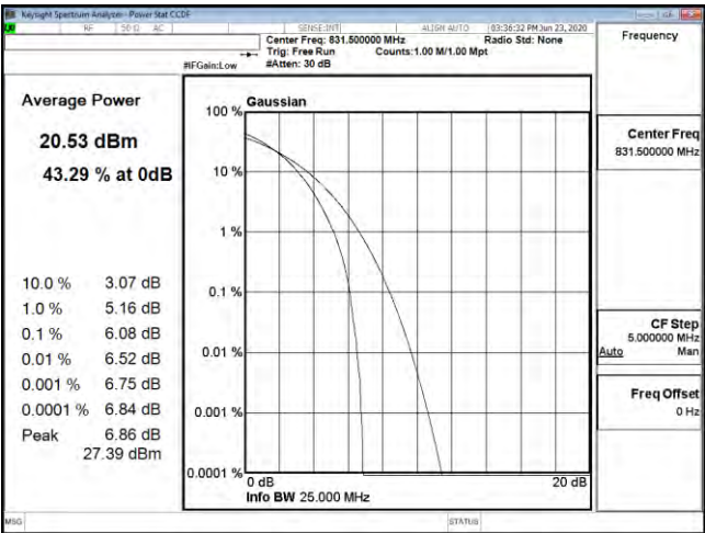
PTAR B26 15M CH26865 64QAM
