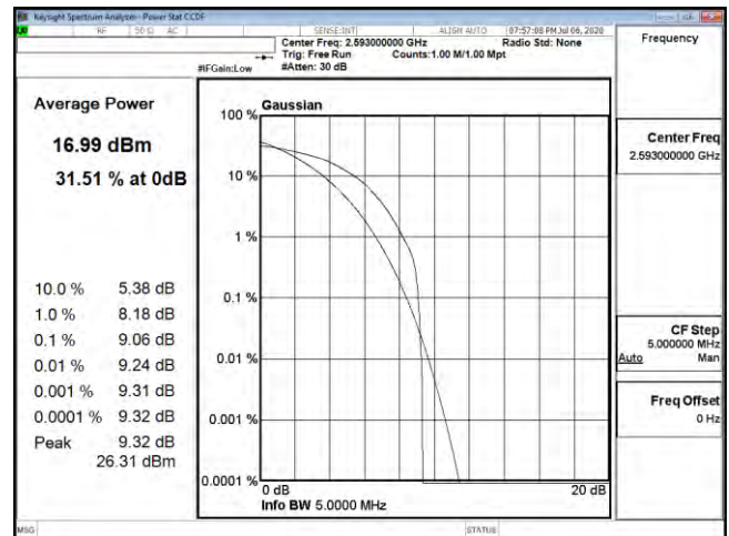
PTAR B41 5M CH40620 64QAM
