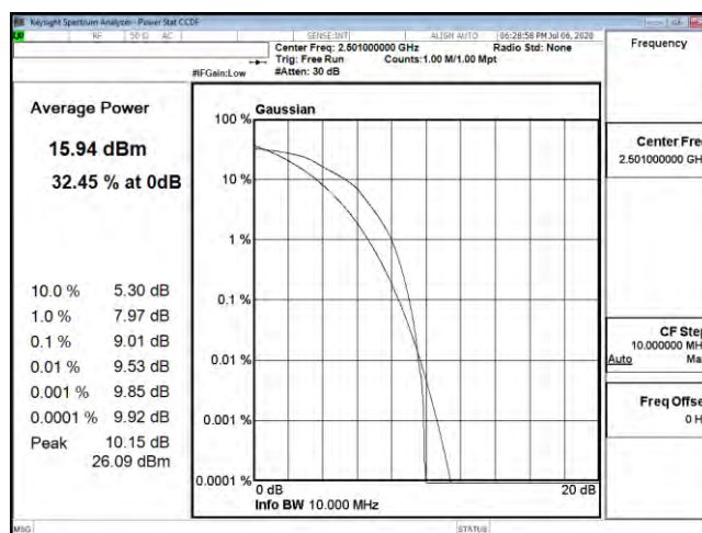
PTAR B41 10M CH39700 16QAM
