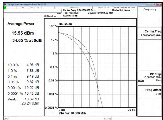
PTAR B41 10M CH39700 64QAM
