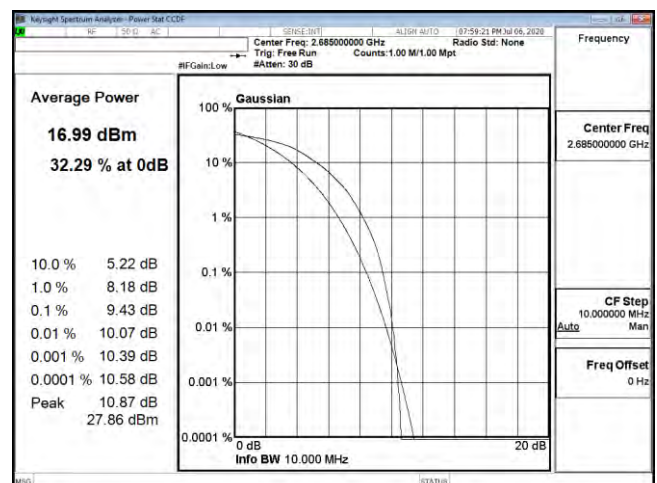
PTAR B41 10M CH41540 64QAM
