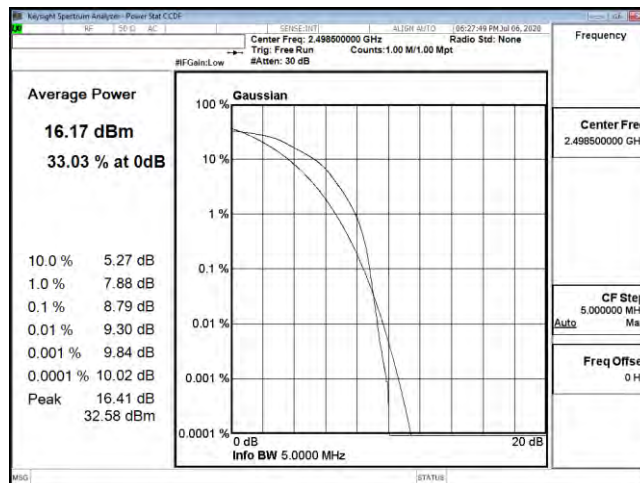
PTAR B41 5M CH39675 16QAM
