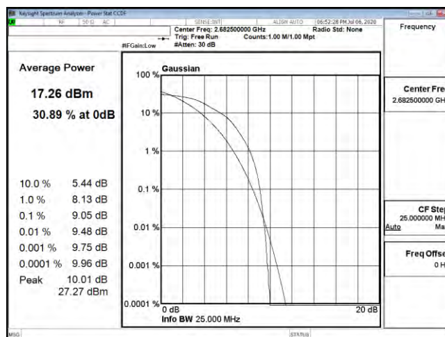
PTAR B41 15M CH41515 16QAM
