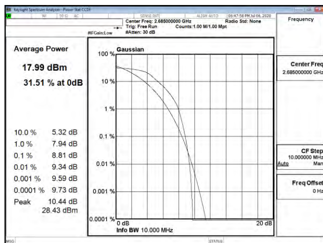
PTAR B41 10M CH41540 QPSK
