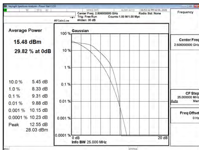
PTAR B41 20M CH39750 QPSK
