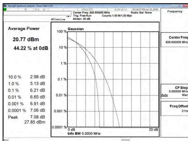
PTAR B26 5M CH26815 64QAM
