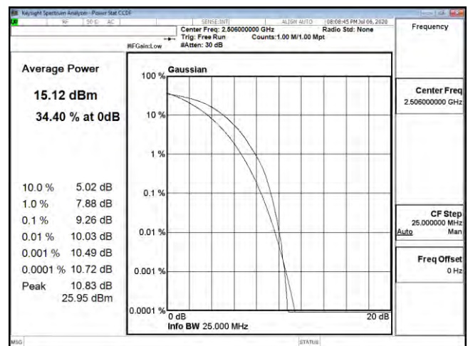
PTAR B41 20M CH39750 64QAM
