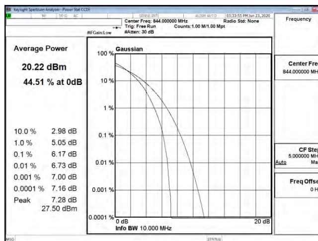
PTAR B26 10M CH26990 64QAM
