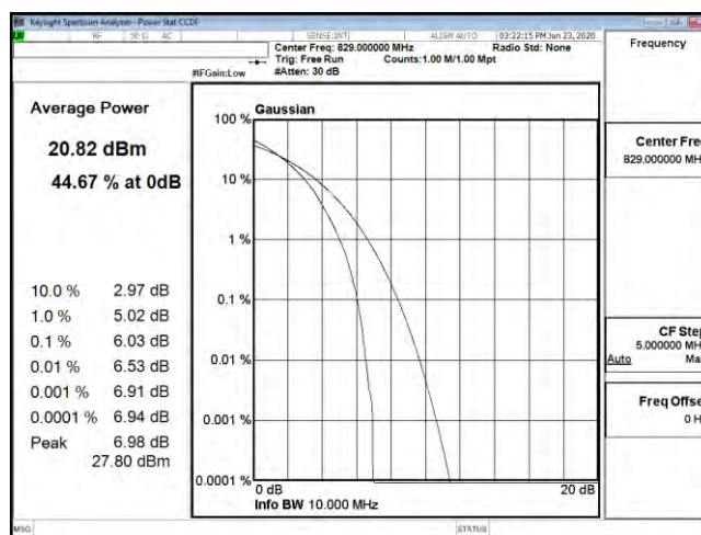
PTAR B26 10M CH26840 64QAM
