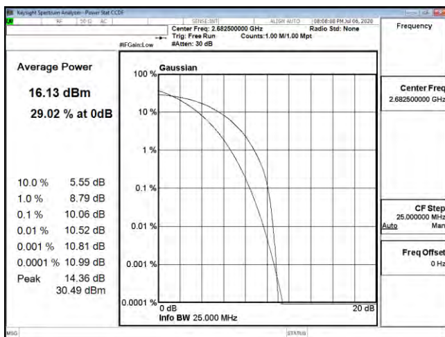
PTAR B41 15M CH41515 64QAM
