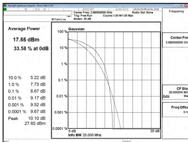
PTAR B41 20M CH41490 16QAM
