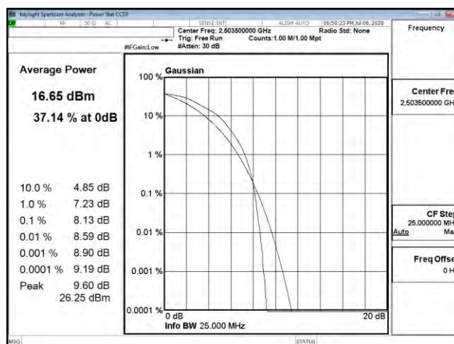
PTAR B41 15M CH39725 16QAM
