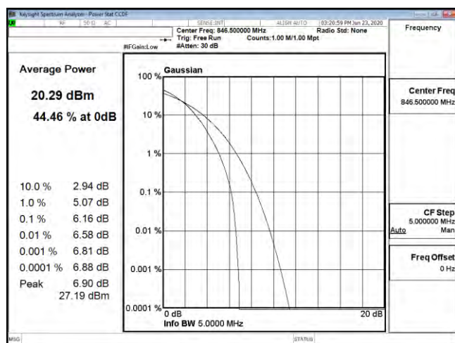
PTAR B26 5M CH27015 64QAM
