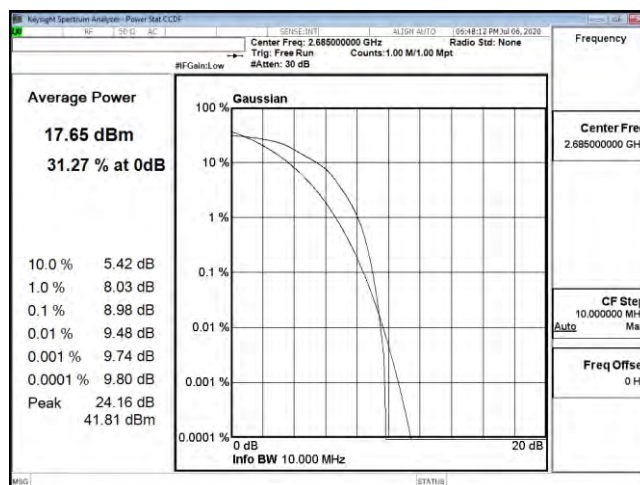
PTAR B41 10M CH41540 16QAM
