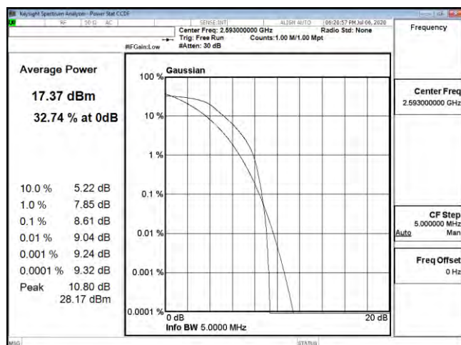
PTAR B41 5M CH40620 QPSK
