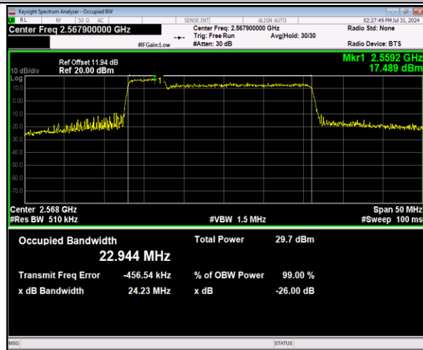
41-41-5MHz-20MHz-64QAM-64QAM-40273-40390-25RB#0-100RB#0-PASS
