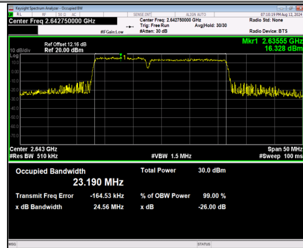
41-41-10MHz-15MHz-16QAM-16QAM-41045-41165-50RB#0-75RB#0-PASS
