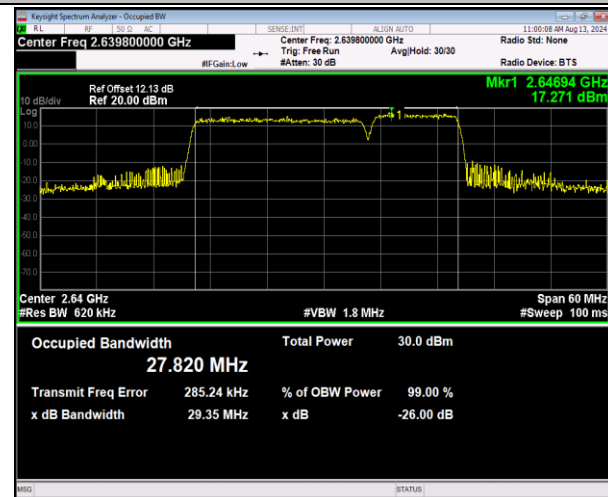
41-41-20MHz-10MHz-16QAM-16QAM-41041-41185-100RB #0-50RB#0-PASS
