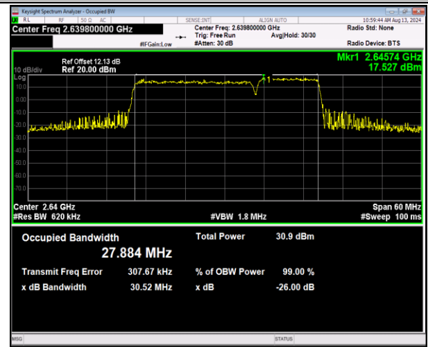
41-41-20MHz-10MHz-QPSK-QPSK-41041-41185-100RB #0-50RB#0-PASS
