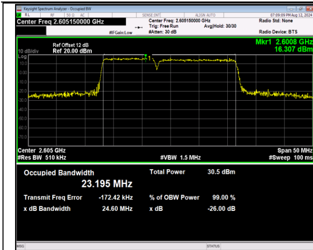
41-41-10MHz-15MHz-QPSK-QPSK-40669-40789-50RB#0-75RB#0-PASS
