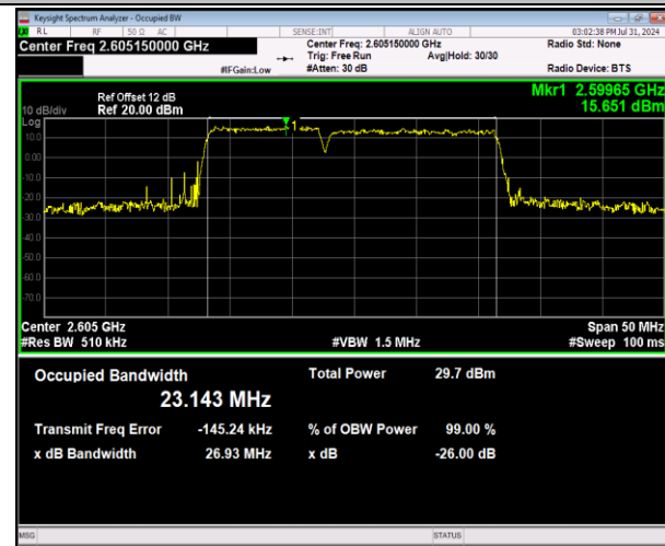
41-41-10MHz-15MHz-64QAM-64QAM-40669-40789-50RB#0-75RB#0-PASS
