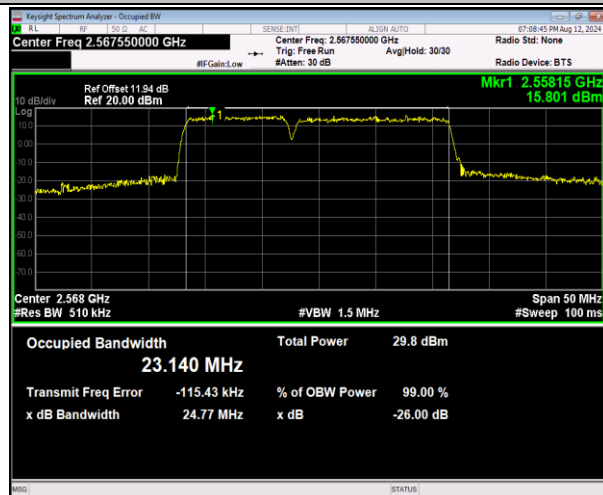
41-41-10MHz-15MHz-16QAM-16QAM-40293-40413-50RB#0-75RB#0-PASS
