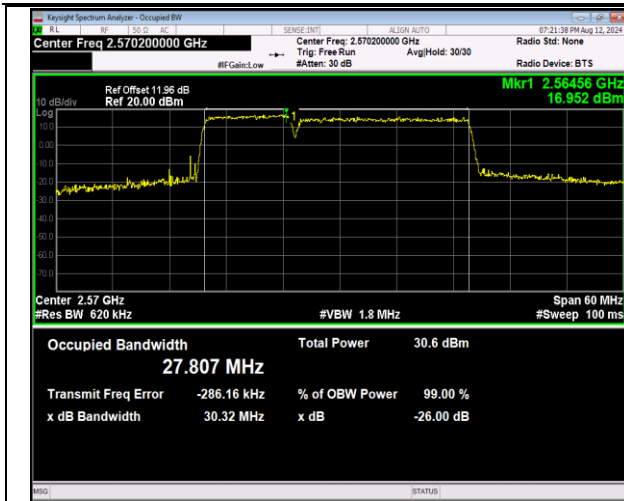
41-41-10MHz-20MHz-QPSK-QPSK-40295-40439-50RB#0-100RB#0-PASS
