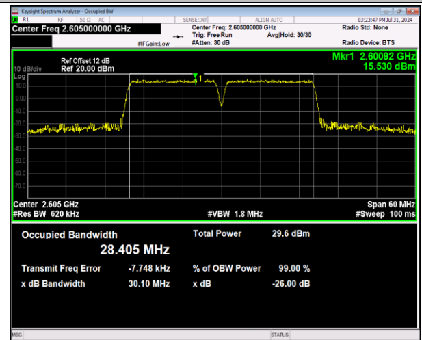
41-41-15MHz-15MHz-64QAM-64QAM-40665-40815-75RB#0-75RB#0-PASS
