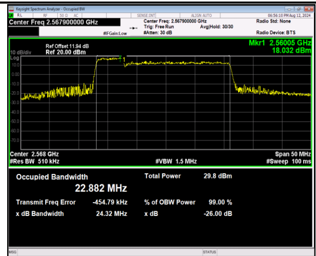
41-41-5MHz-20MHz-16QAM-16QAM-40273-40390-25RB#0-100RB#0-PASS
