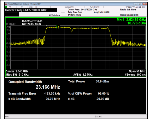
41-41-10MHz-15MHz-QPSK-QPSK-41045-41165-50RB#0-75RB#0-PASS
