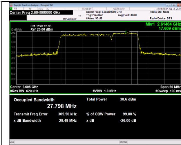
41-41-20MHz-10MHz-QPSK-QPSK-40691-40835-100RB #0-50RB#0-PASS
