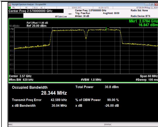
41-41-15MHz-15MHz-QPSK-QPSK-40315-40465-75RB#0-75RB#0-PASS
