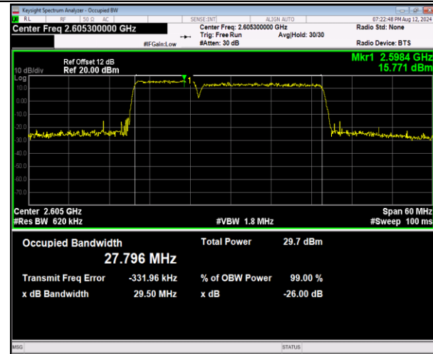
41-41-10MHz-20MHz-16QAM-16QAM-40646-40790-50RB#0-100RB#0-PASS
