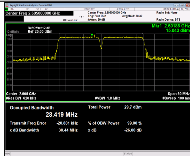
41-41-15MHz-15MHz-16QAM-16QAM-40665-40815-75RB#0-75RB#0-PASS
