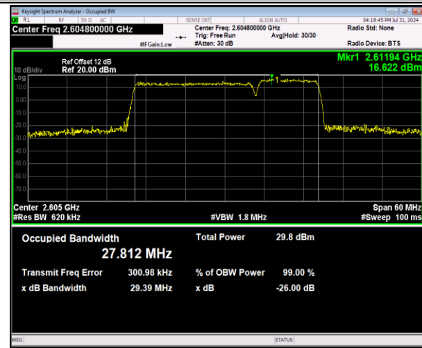
41-41-20MHz-10MHz-64QAM-64QAM-40691-40835-100RB #0-50RB#0-PASS
