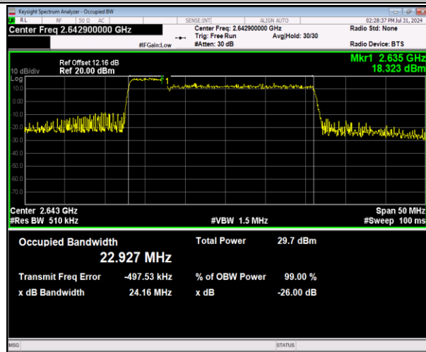
41-41-5MHz-20MHz-64QAM-64QAM-41023-41140-25RB#0-100RB#0-PASS
