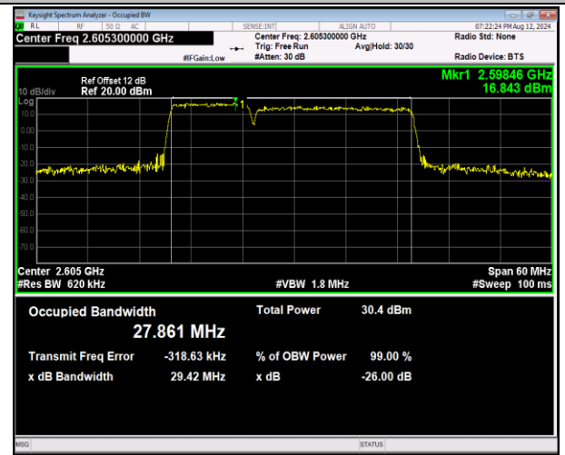
41-41-10MHz-20MHz-QPSK-QPSK-40646-40790-50RB#0-100RB#0-PASS
