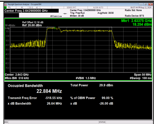
41-41-5MHz-20MHz-16QAM-16QAM-41023-41140-25RB#0-100RB#0-PASS
