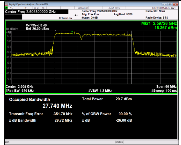
41-41-10MHz-20MHz-64QAM-64QAM-40646-40790-50RB#0-100RB#0-PASS
