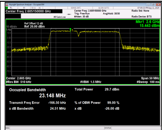
41-41-10MHz-15MHz-16QAM-16QAM-40669-40789-50RB#0-75RB#0-PASS
