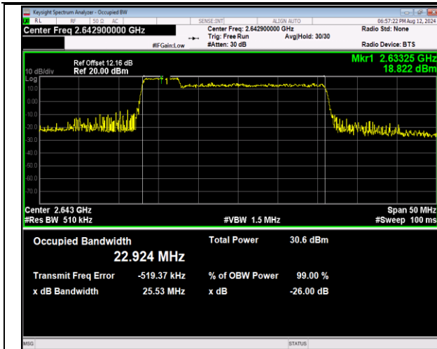
41-41-5MHz-20MHz-QPSK-QPSK-41023-41140-25RB#0-100RB#0-PASS
