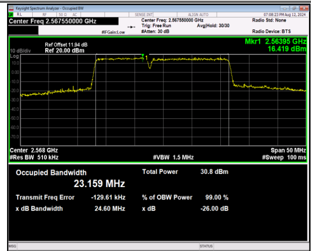
41-41-10MHz-15MHz-QPSK-QPSK-40293-40413-50RB#0-75RB#0-PASS
