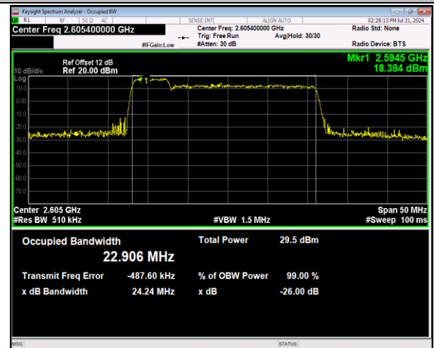
41-41-5MHz-20MHz-64QAM-64QAM-40648-40765-25RB#0-100RB#0-PASS
