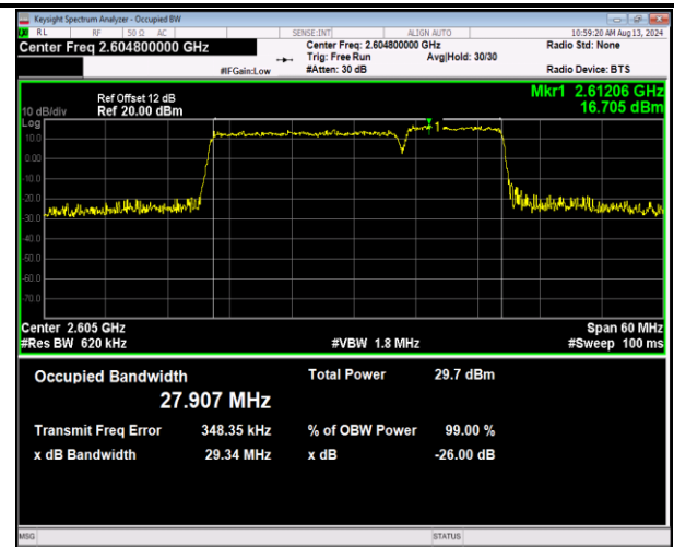
41-41-20MHz-10MHz-16QAM-16QAM-40691-40835-100RB #0-50RB#0-PASS
