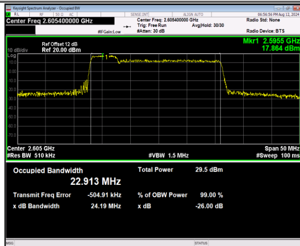
41-41-5MHz-20MHz-16QAM-16QAM-40648-40765-25RB#0-100RB#0-PASS
