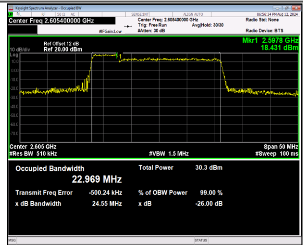
41-41-5MHz-20MHz-QPSK-QPSK-40648-40765-25RB#0-100RB#0-PASS
