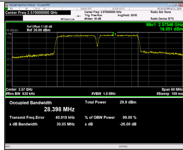
41-41-15MHz-15MHz-64QAM-64QAM-40315-40465-75RB#0-75RB#0-PASS
