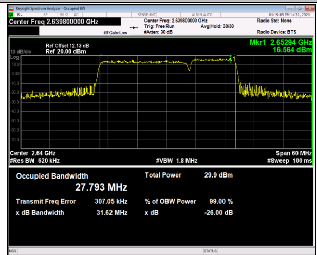
41-41-20MHz-10MHz-64QAM-64QAM-41041-41185-100RB #0-50RB#0-PASS
