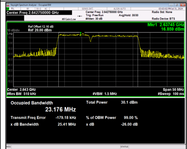
41-41-10MHz-15MHz-64QAM-64QAM-41045-41165-50RB#0-75RB#0-PASS
