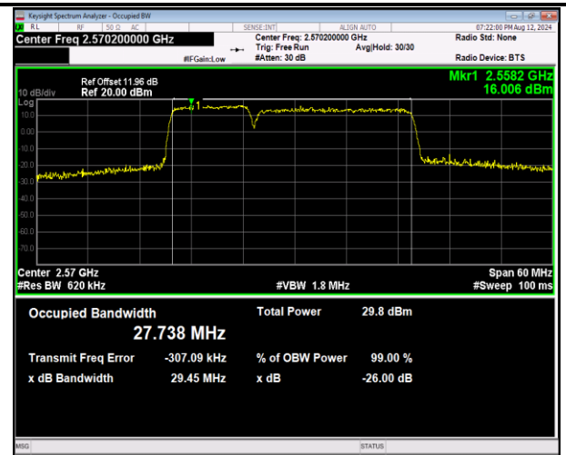
41-41-10MHz-20MHz-16QAM-16QAM-40295-40439-50RB#0-100RB#0-PASS
