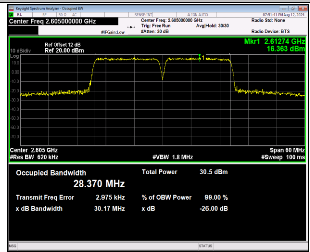
41-41-15MHz-15MHz-QPSK-QPSK-40665-40815-75RB#0-75RB#0-PASS
