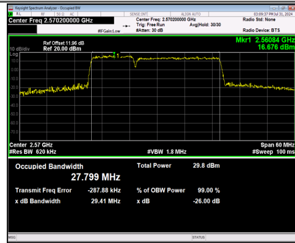
41-41-10MHz-20MHz-64QAM-64QAM-40295-40439-50RB#0-100RB#0-PASS
