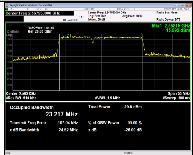
41-41-10MHz-15MHz-64QAM-64QAM-40293-40413-50RB#0-75RB#0-PASS
