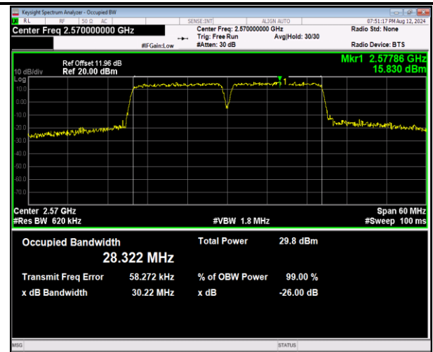
41-41-15MHz-15MHz-16QAM-16QAM-40315-40465-75RB#0-75RB#0-PASS
