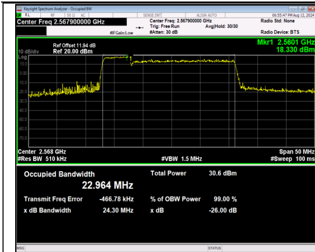
41-41-5MHz-20MHz-QPSK-QPSK-40273-40390-25RB#0-100RB#0-PASS
