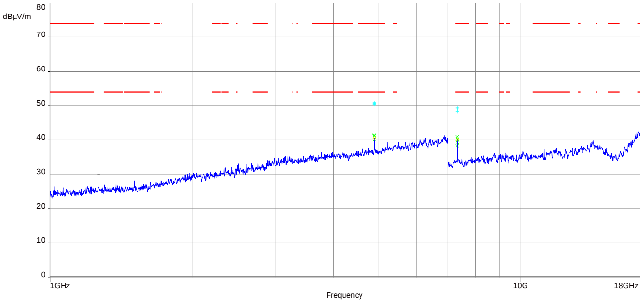
Plot 1: 1 GHz to 18 GHz, TX mode, 2440 MHz, vertical & horizontal polarization
