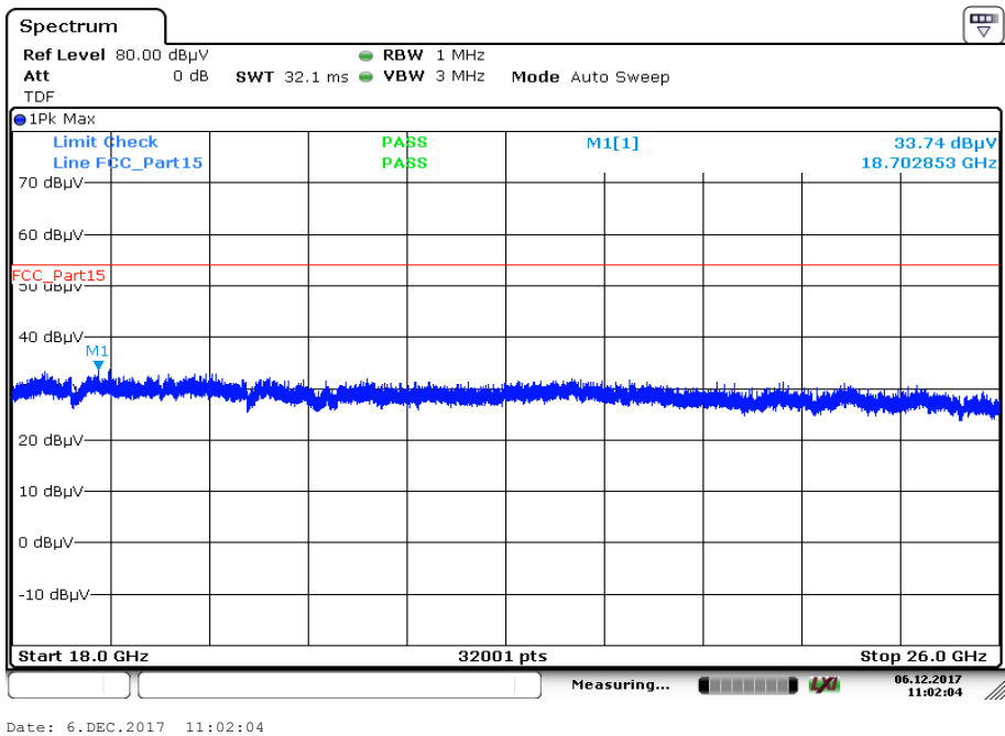
Plot 2: 18 GHz to 26 GHz, TX mode, 2440 MHz, vertical & horizontal polarization
