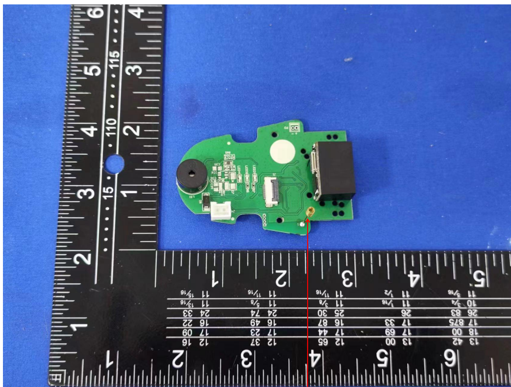
BT ANT and 2.4G ANT
