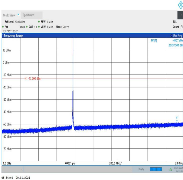
Band66_5MHz_16QAM_132647_1RB#24_1000~3000_1000~3000
