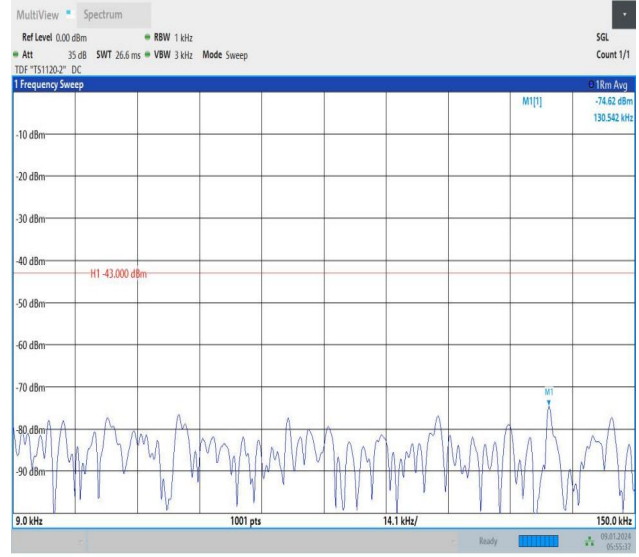
Band66_5MHz_16QAM_132647_25RB#0_0.009~0.15_0.009~0.15
