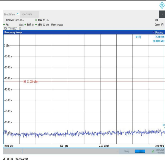
Band66_10MHz_QPSK_132022_1RB#0_0.15~30_0.15~30
