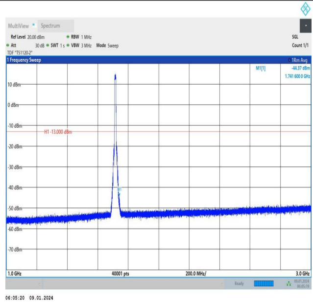
Band66_10MHz_QPSK_132022_50RB#0_1000~3000_1000~3000
