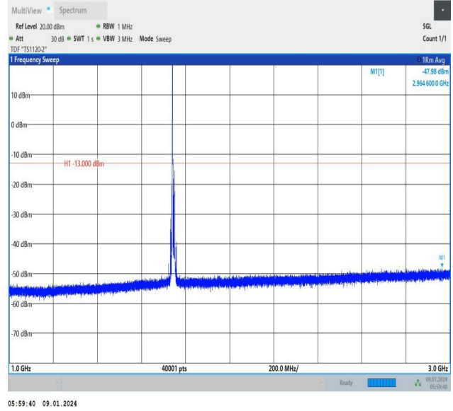
Band66_10MHz_QPSK_132322_1RB#0_1000~3000_1000~3000
