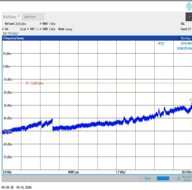
Band66_10MHz_QPSK_132022_50RB#0_3000~20000_3000~20000
