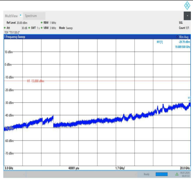
Band66_10MHz_16QAM_132322_1RB#49_3000~20000_300 0~20000
