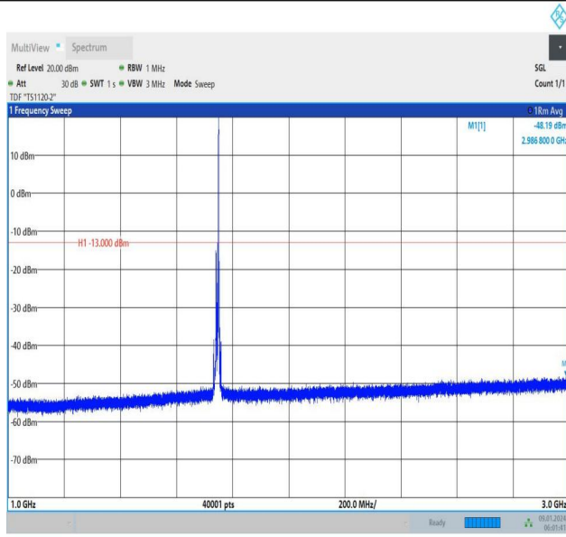
Band66_10MHz_16QAM_132322_1RB#49_1000~3000_1000 ~3000
