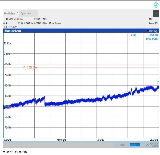
Band66_5MHz_16QAM_132647_25RB#0_3000~20000_3000~20000
