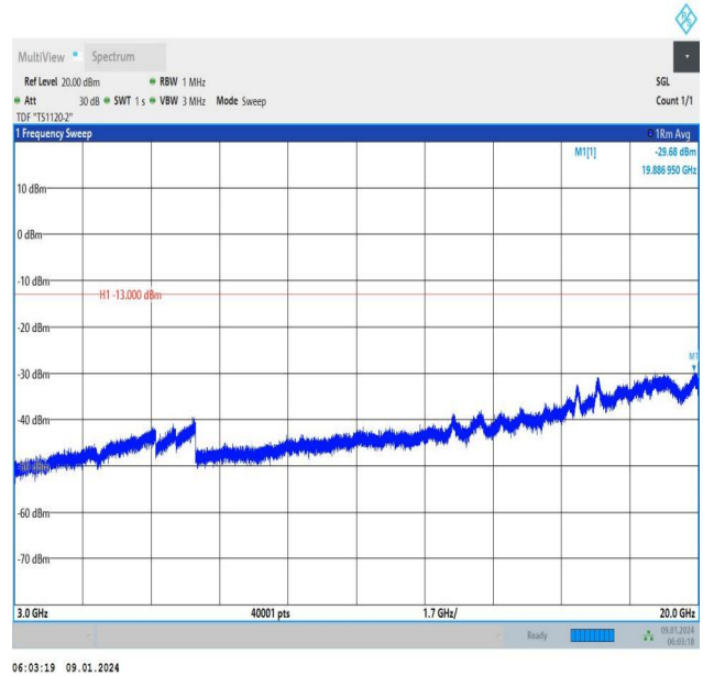
Band66_10MHz_16QAM_132622_1RB#0_3000~20000_3000~20000
