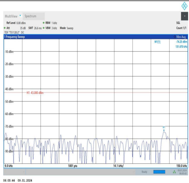
Band66_10MHz_QPSK_132322_50RB#0_0.009~0.15_0.009~0.15
