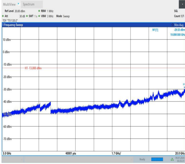
Band66_5MHz_QPSK_132647_25RB#0_3000~20000_3000~20000
