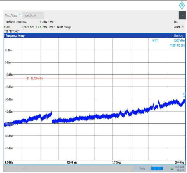
Band66_10MHz_16QAM_132622_1RB#49_3000~20000_300 0~20000
