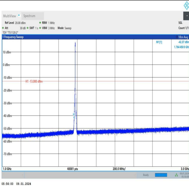
Band66_5MHz_16QAM_132647_25RB#0_1000~3000_1000~3000
