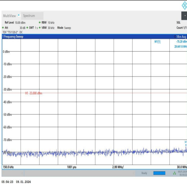
Band66_5MHz_16QAM_132647_1RB#24_0.15~30_0.15~30
