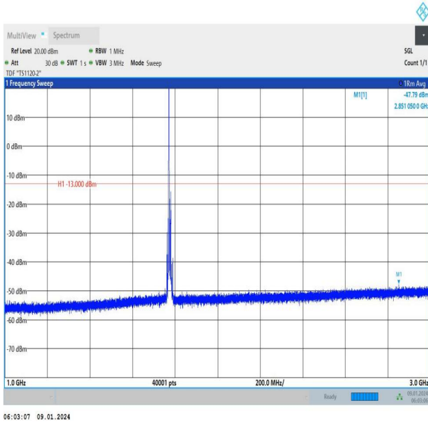
Band66_10MHz_16QAM_132622_1RB#0_1000~3000_1000~3000
