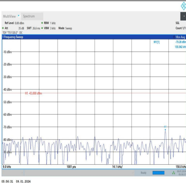
Band66_10MHz_QPSK_132022_1RB#0_0.009~0.15_0.009~0.15
