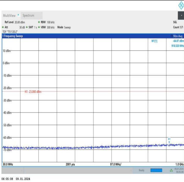
Band66_10MHz_QPSK_132022_50RB#0_30~1000_30~1000
