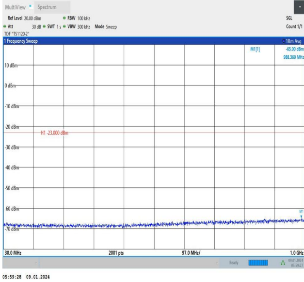
Band66_10MHz_QPSK_132322_1RB#0_30~1000_30~1000
