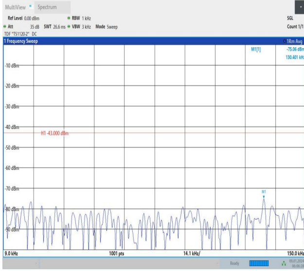
Band66_10MHz_QPSK_132622_50RB#0_0.009~0.15_0.009~0.15
