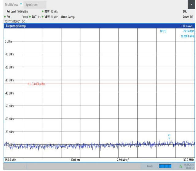
Band66_10MHz_QPSK_132622_50RB#0_0.15~30_0.15~30
