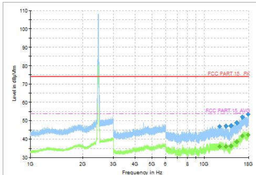
Fig.126 Radiated Spurious Emission (802.11n-HT20, CH11, 1GHz-18GHz, MIMO)
