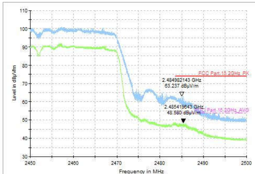
Fig.148 Radiated Restricted Band (802.11-VHT40, CH9, 2.45GHz~2.50GHz, MIMO)
