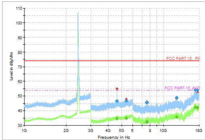
Fig.135 Radiated Spurious Emission (802.11ax-HE20, CH6, 1GHz-18GHz, MIMO)
