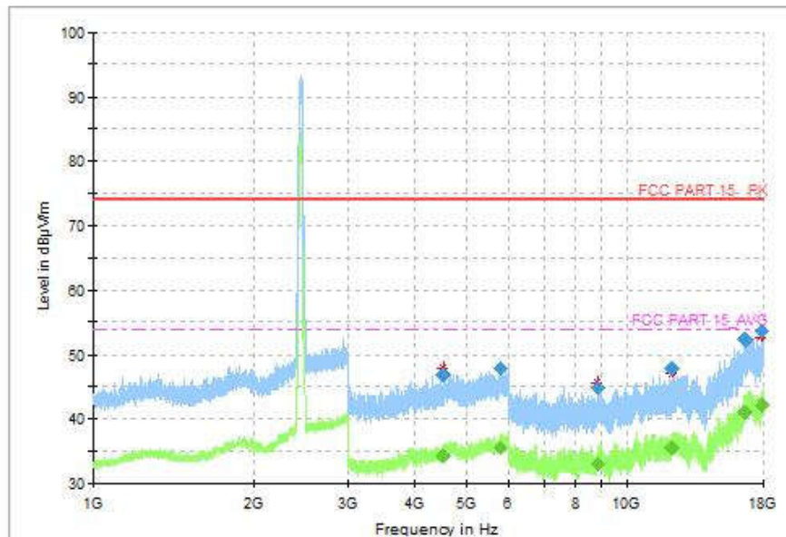
Fig.108 Radiated Spurious Emission (802.11n-HT40, CH9, 1GHz-18GHz)
