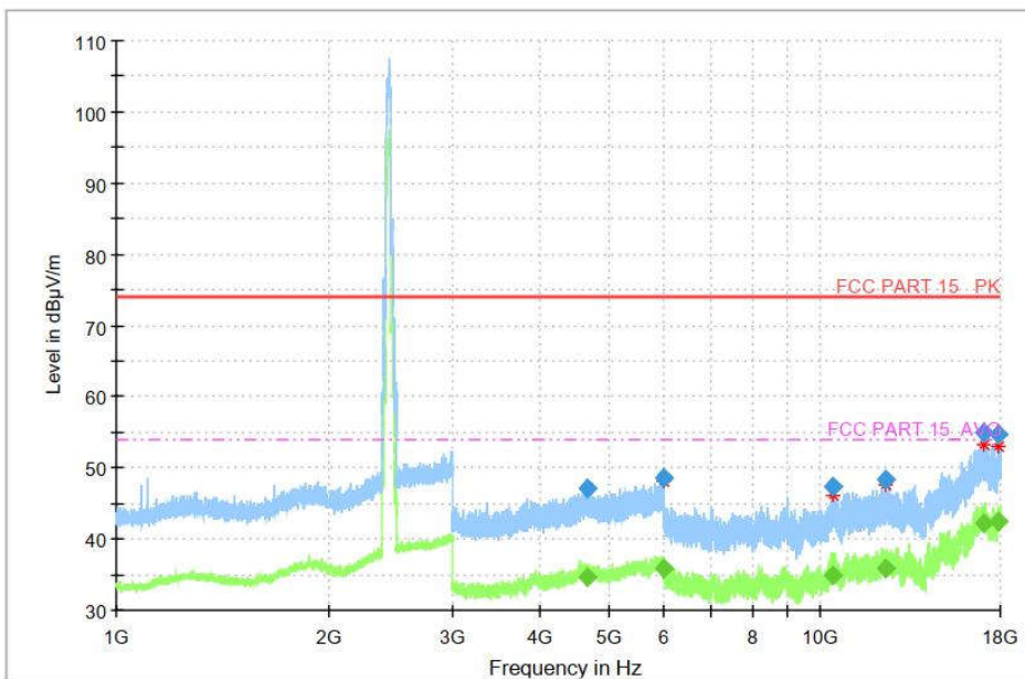
Fig.150 Radiated Spurious Emission (802.11ax-HE40, CH6, 1GHz-18GHz, MIMO)
