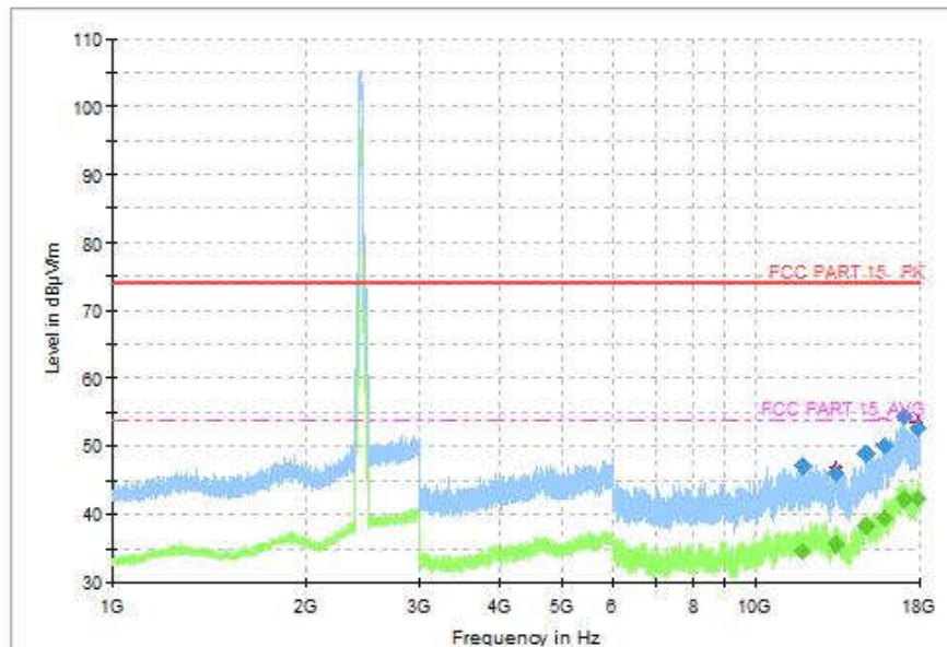
Fig.140 Radiated Spurious Emission (802.11n-HT40, CH6, 1GHz-18GHz, MIMO)
