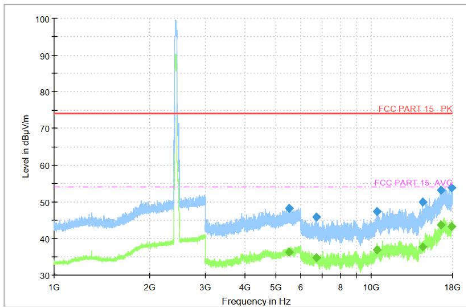
Fig.116 Radiated Spurious Emission (802.11ax-HE40, CH3, 1GHz-18GHz)
