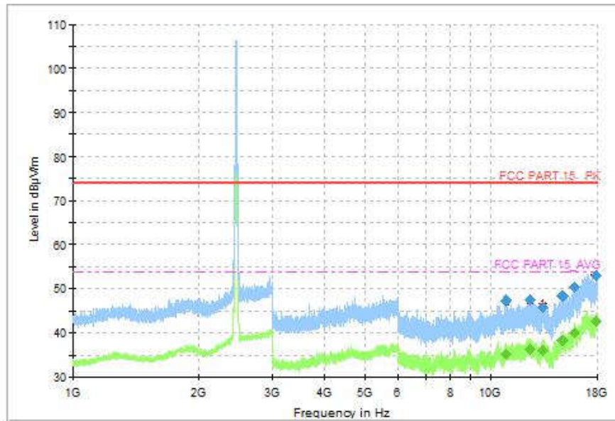
Fig.131 Radiated Spurious Emission (802.11-VHT20, CH11, 1GHz-18GHz, MIMO)
