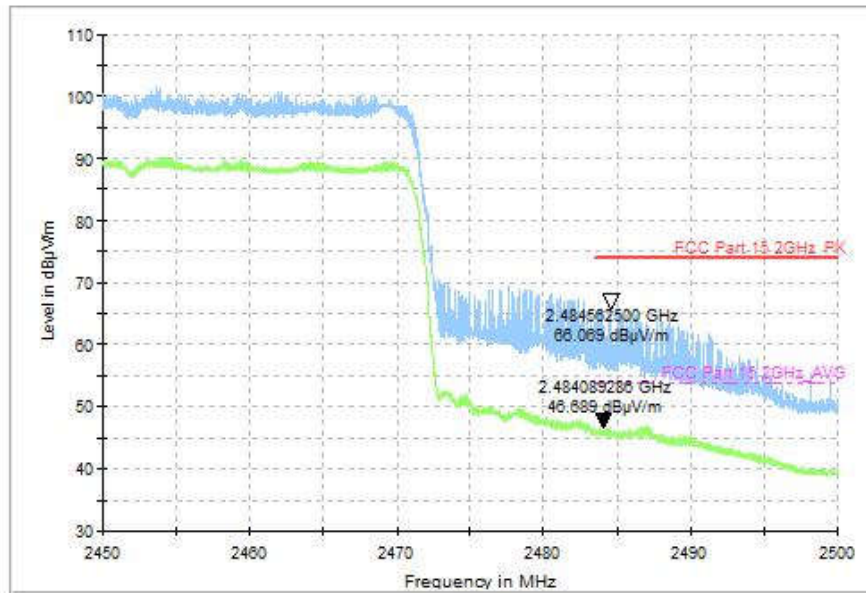
Fig.153 Radiated Restricted Band (802.11ax-HE40, CH9, 2.45GHz~2.50GHz, MIMO)
