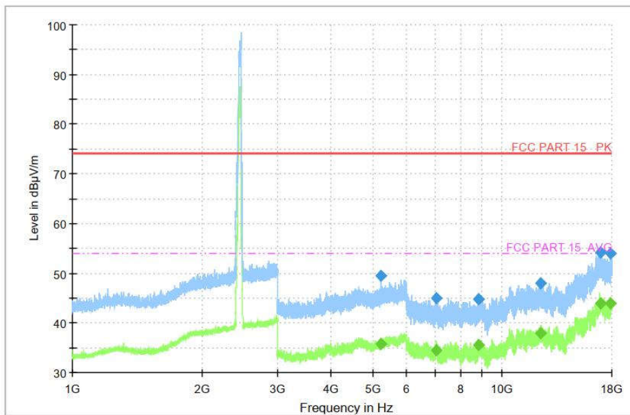
Fig.118 Radiated Spurious Emission (802.11ax-HE40, CH9, 1GHz-18GHz)
