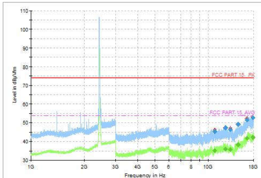
Fig.130 Radiated Spurious Emission (802.11-VHT20, CH6, 1GHz-18GHz, MIMO)
