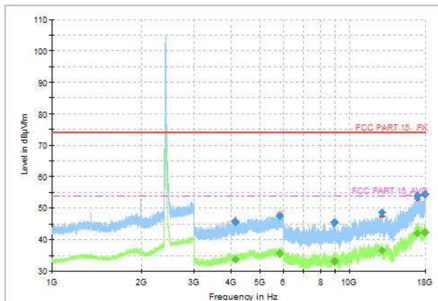
Fig.134 Radiated Spurious Emission (802.11ax-HE20, CH1, 1GHz-18GHz, MIMO)
