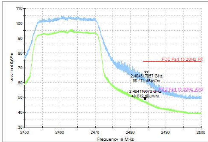
Fig.133 Radiated Restricted Band (802.11-VHT20, CH11, 2.45GHz~2.50GHz, MIMO)
