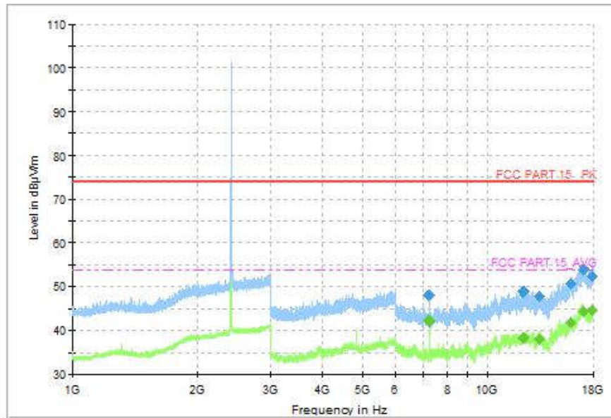
Fig.111 Radiated Spurious Emission (802.11-VHT40, CH3, 1GHz-18GHz)
