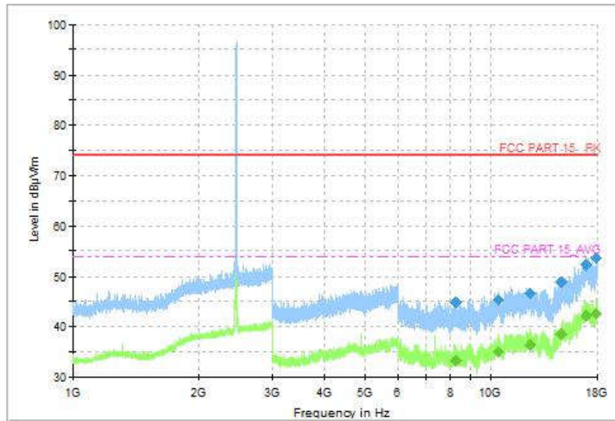
Fig.113 Radiated Spurious Emission (802.11-VHT40, CH9, 1GHz-18GHz)
