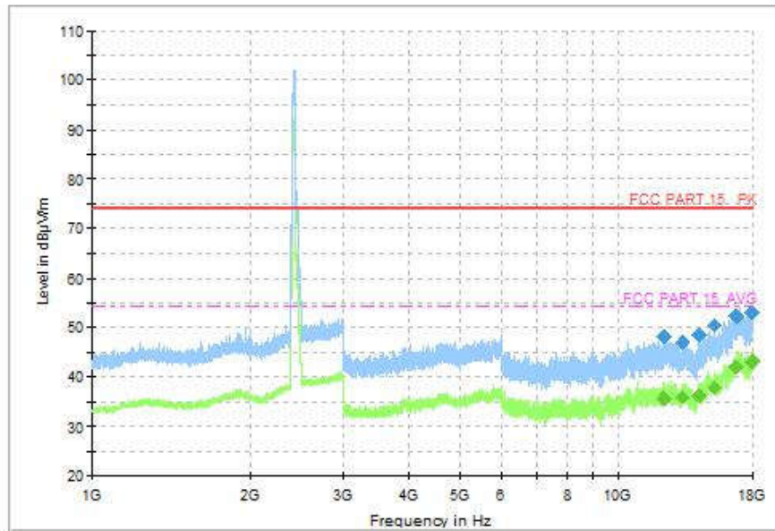
Fig.139 Radiated Spurious Emission (802.11n-HT40, CH3, 1GHz-18GHz, MIMO)
