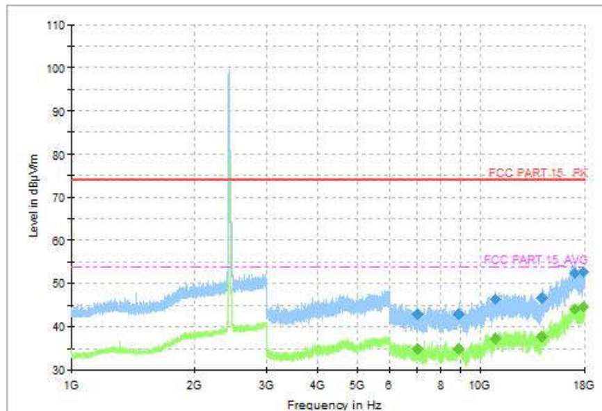
Fig.102 Radiated Spurious Emission (802.11ax-HE20, CH6, 1GHz-18GHz)
