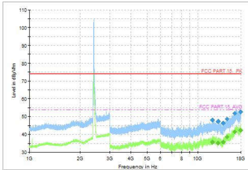
Fig.129 Radiated Spurious Emission (802.11-VHT20, CH1, 1GHz-18GHz, MIMO)
