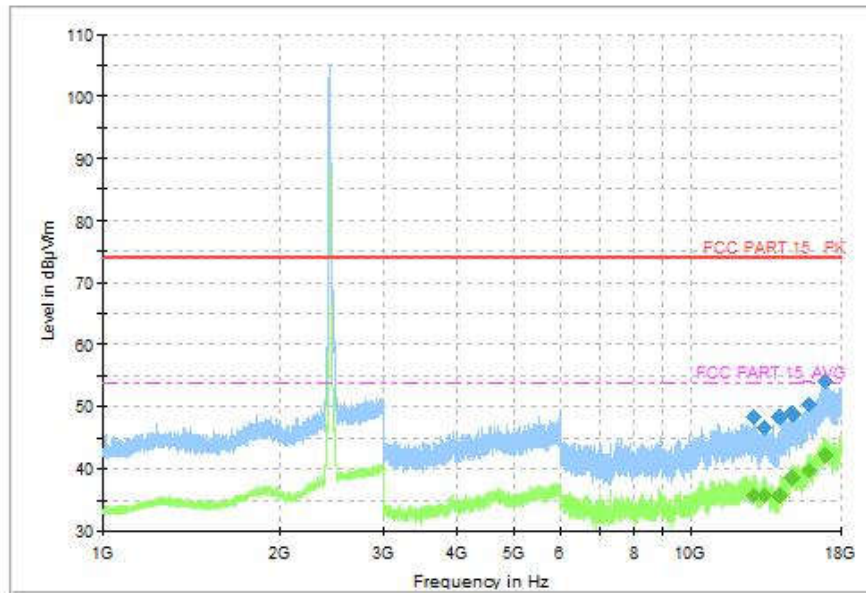
Fig.125 Radiated Spurious Emission (802.11n-HT20, CH6, 1GHz-18GHz, MIMO)
