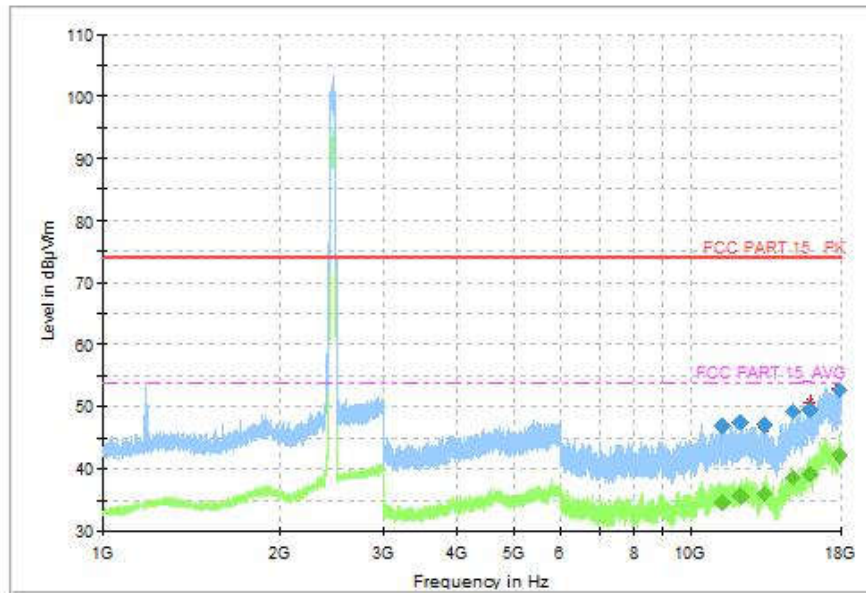
Fig.141 Radiated Spurious Emission (802.11n-HT40, CH9, 1GHz-18GHz, MIMO)
