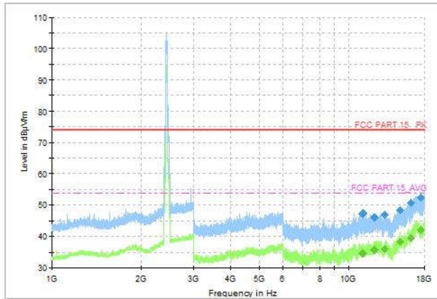
Fig.145 Radiated Spurious Emission (802.11-VHT40, CH6, 1GHz-18GHz, MIMO)
