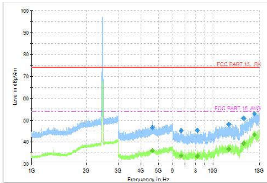
Fig.103 Radiated Spurious Emission (802.11ax-HE20, CH11, 1GHz-18GHz)
