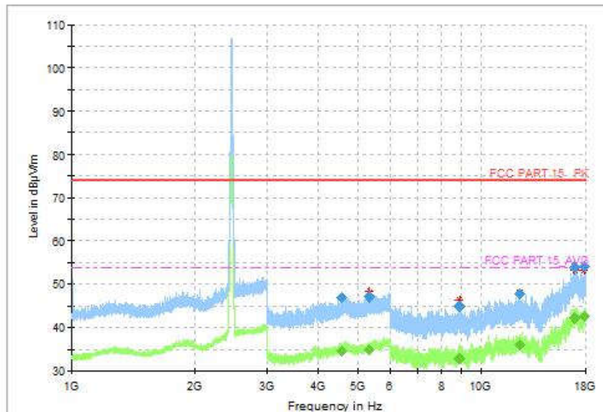
Fig.136 Radiated Spurious Emission (802.11ax-HE20, CH11, 1GHz-18GHz, MIMO)
