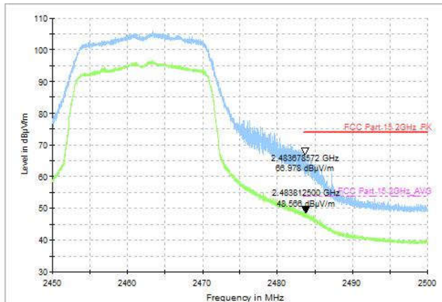
Fig.128 Radiated Restricted Band (802.11n-HT20, CH11, 2.45GHz~2.50GHz, MIMO)
