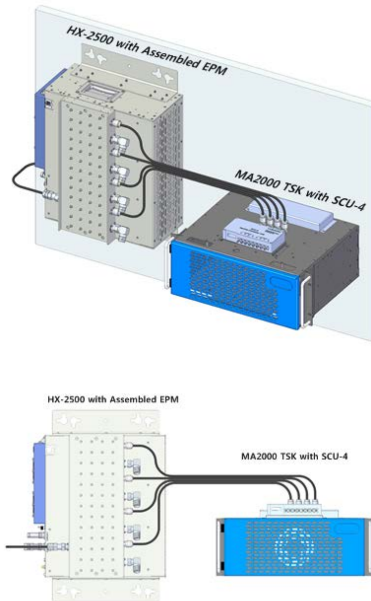
Example of HX 2.5 GHz TDD with Assembled EPM Alongside MA2000 TSX Remote | Figure 3-8
