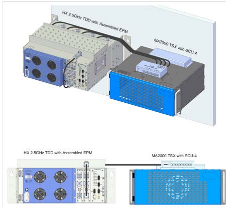
Example of HX 2.5 GHz TDD with Assembled EPM Alongside MA2000 TSX Remote | Figure 3-11
