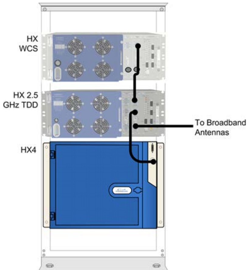
Example of Connections between HX 2.5 GHz TDD, HX WCS and HX4 | Figure 3-19
