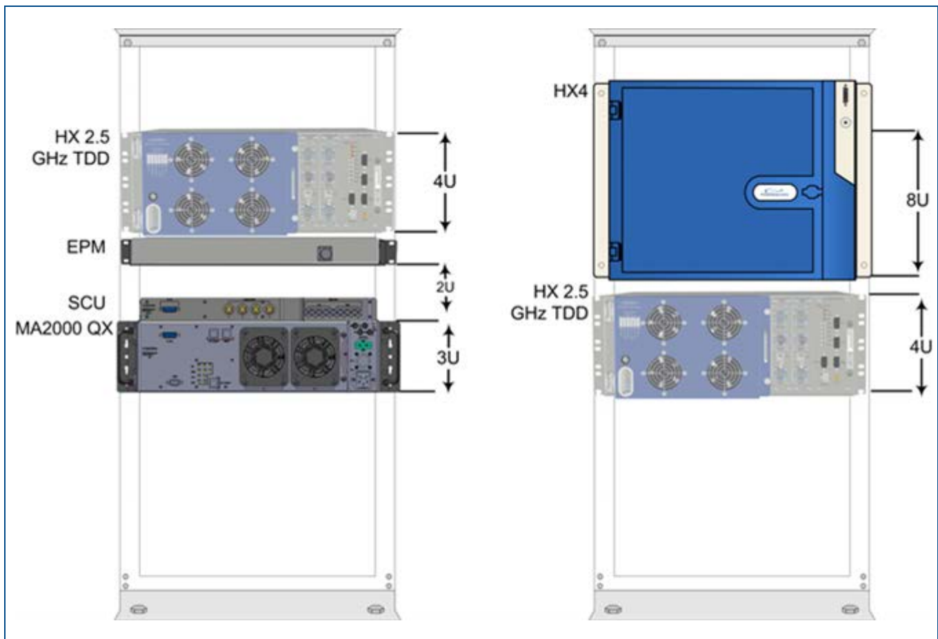
Examples of HX 2.5 GHz TDD Rack Installations with Additional HX4 and MA2000 QX Remotes | Figure 3-1
