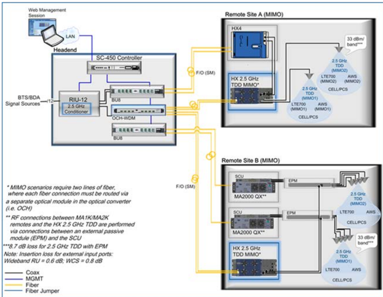
HX 2.5 GHz TDD – MIMO Architecture with an existing HX4 and MA2000 QX, Sharing a Common Headend
