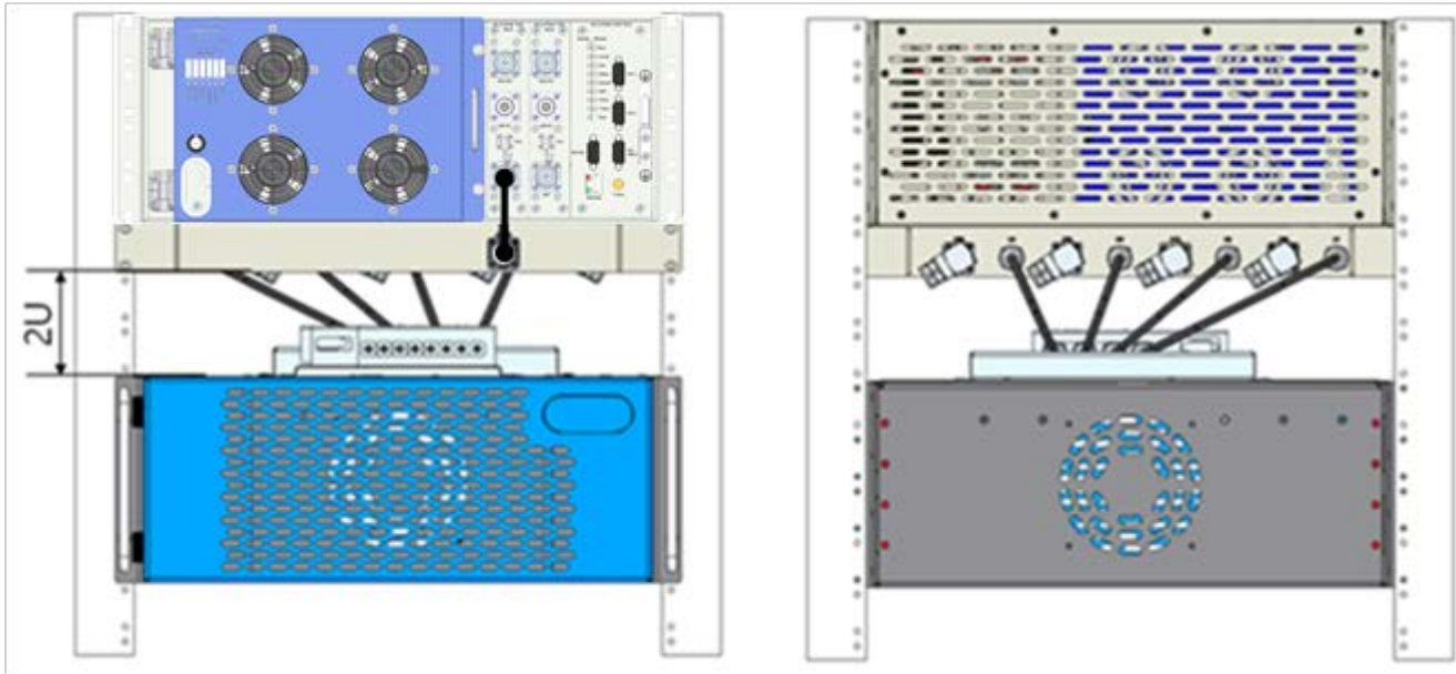
Examples of HX 2.5 GHz TDD Rack Installations with Additional MA2000 TSX Remote | Figure 3-2
