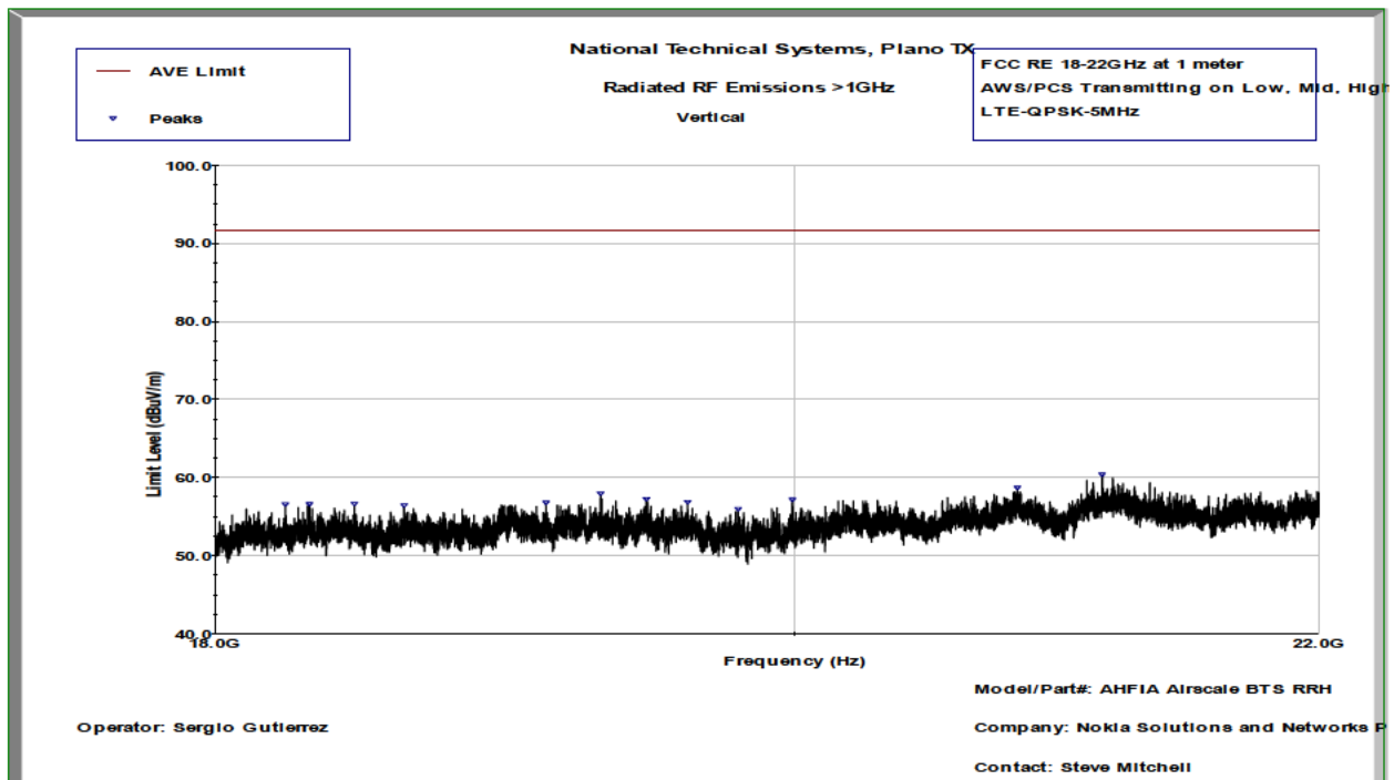
PCS/AWS Carriers 18-22GHz – Vertical at 1m
