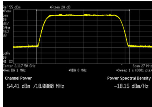
LTE15_Bottom Channel_Peak
