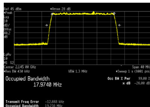
LTE20_256QAM
