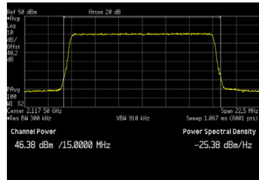
LTE15_Bottom Channel_Average
