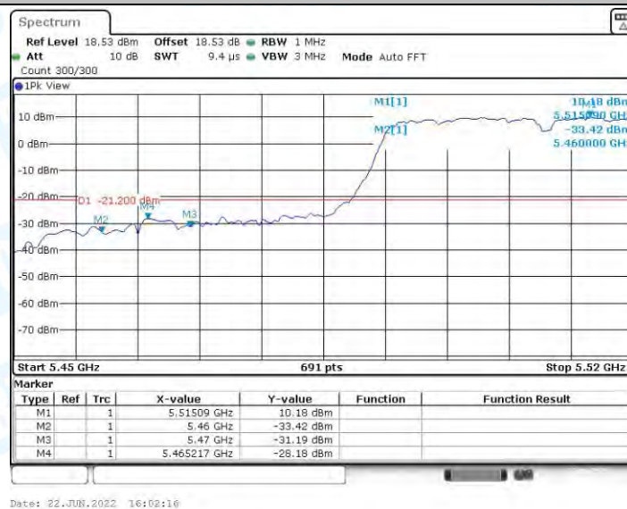
11AC40MIMO_Ant1_Low_5510_Peak
