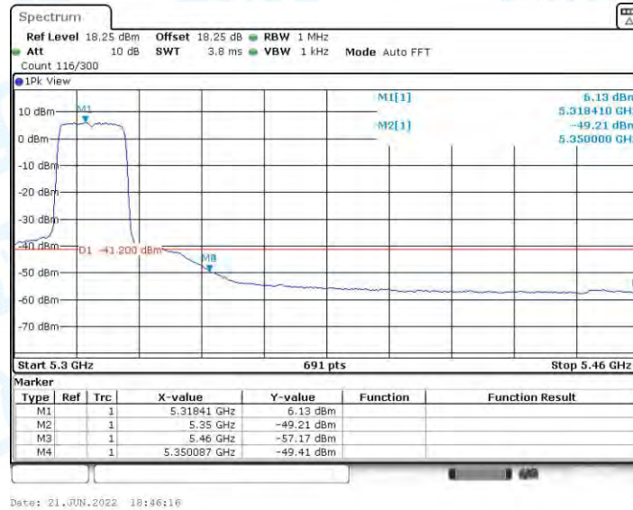
11A_Ant2_High_5320_AV
