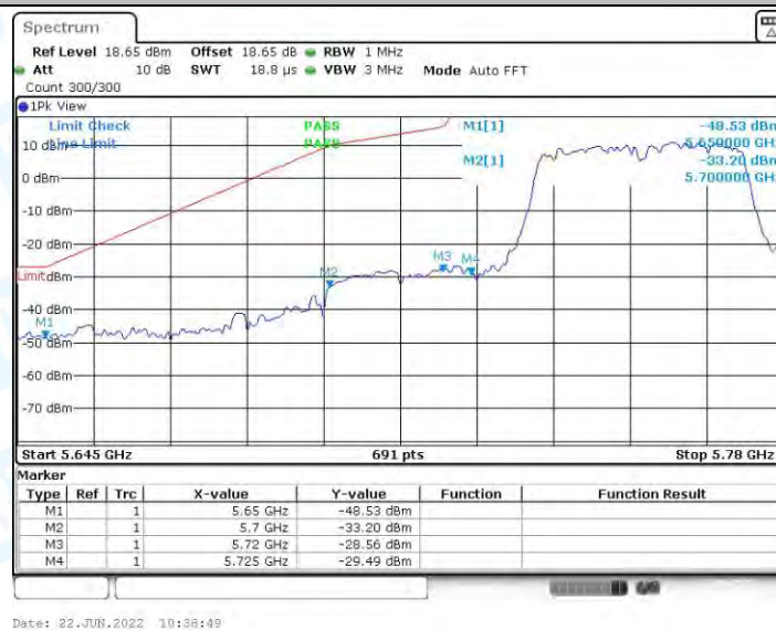
11N40MIMO_Ant1_Low_5755_Peak
