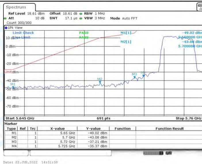
11AC20MIMO_Ant2_Low_5745_Peak
