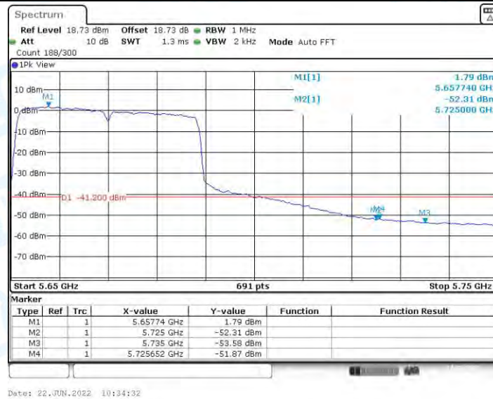
11N40MIMO_Ant2_High_5670_AV
