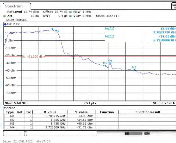
11N20MIMO_Ant2_High_5700_Peak
