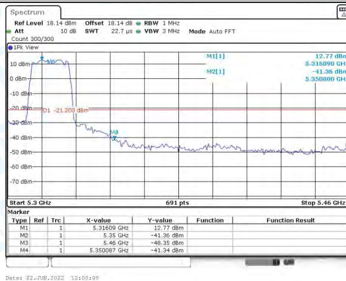
11AC20MIMO_Ant1_High_5320_Peak
