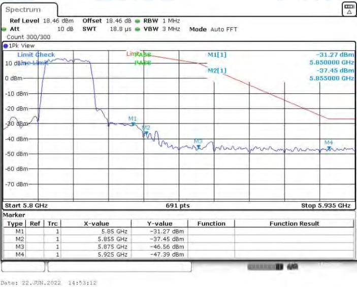
11AC20MIMO_Ant1_High_5825_Peak
