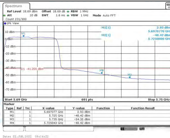
11N20MIMO_Ant1_High_5700_AV
