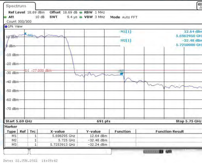
11AC20MIMO_Ant1_High_5700
