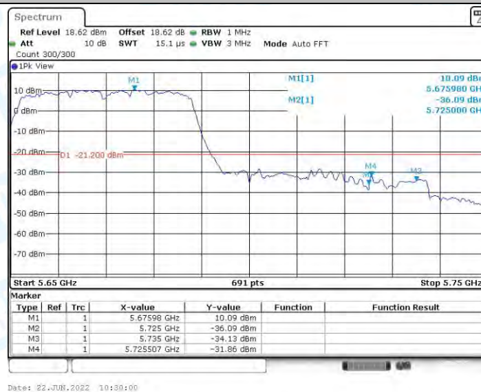
11N40MIMO_Ant1_High_5670_Peak
