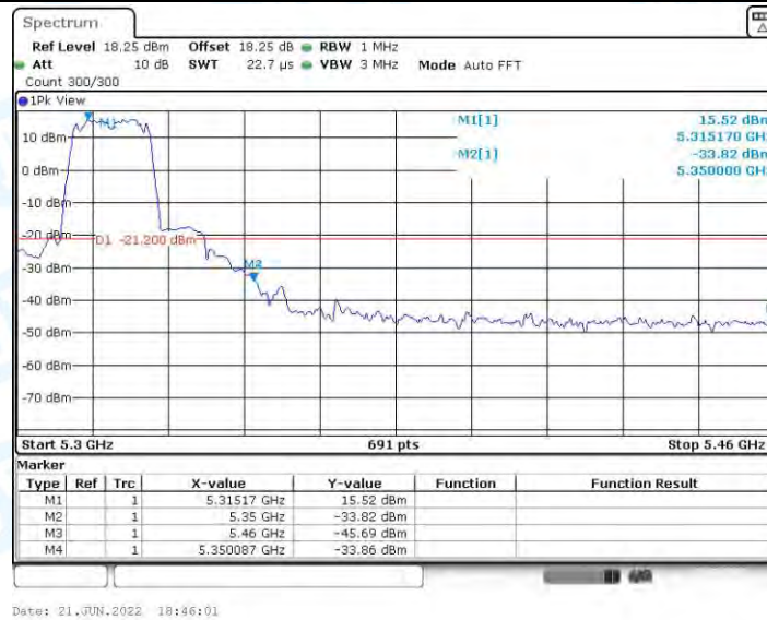
11A_Ant2_High_5320_Peak
