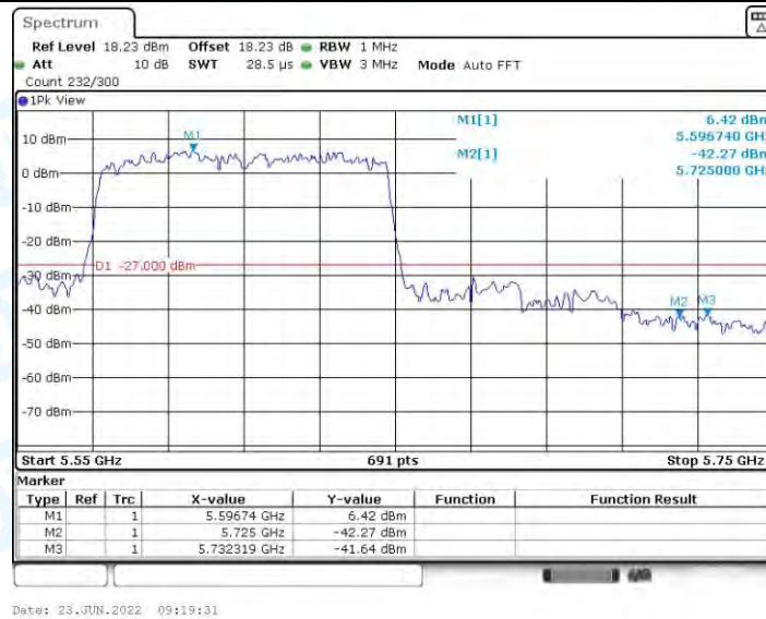
11AC80MIMO_Ant1_High_5610
