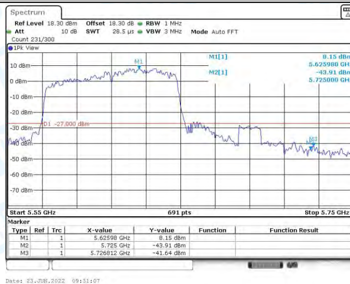
11AC80MIMO_Ant2_High_5610
