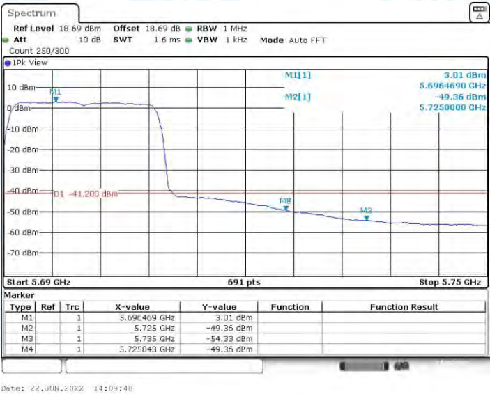
11AC20MIMO_Ant1_High_5700_AV
