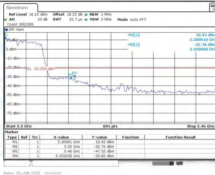
11N40MIMO_Ant2_High_5310_Peak
