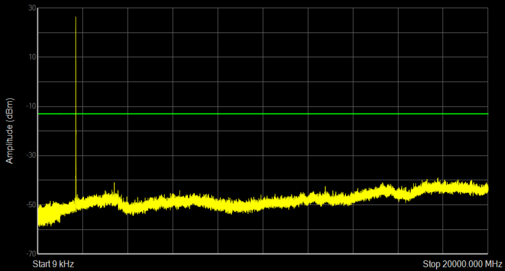
Band66 QPSK BW=5MHz Channel=131997 RB Size=1 Position=#0
