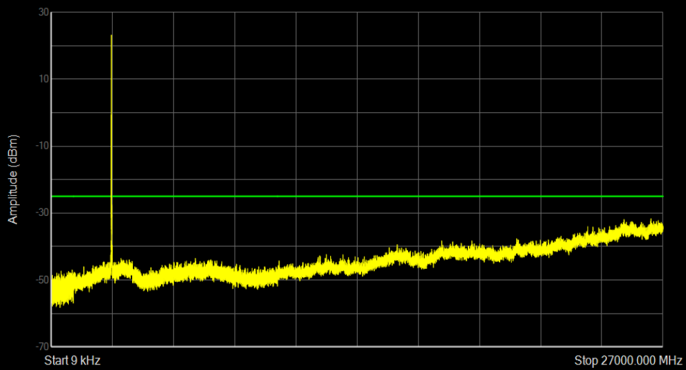
Band41 16QAM BW=20MHz Channel=41490 RB Size=1 Position=#0
