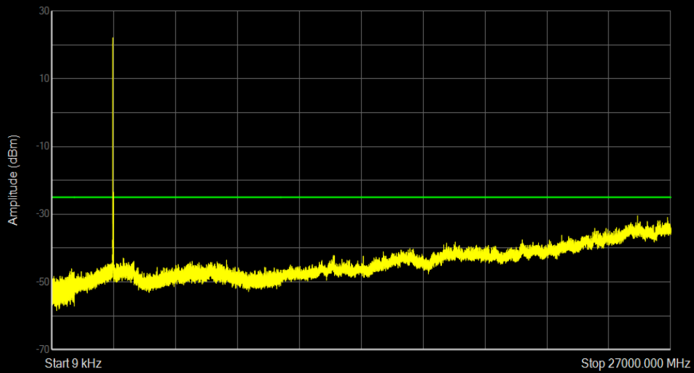
Band41 16QAM BW=15MHz Channel=41515 RB Size=1 Position=#0
