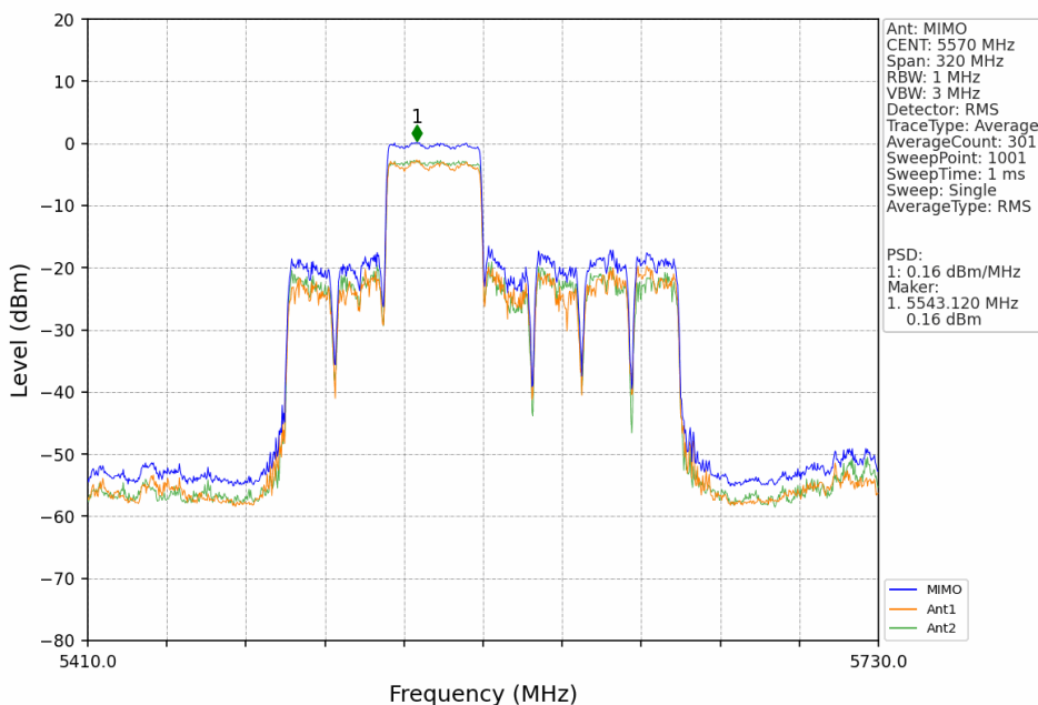
802.11ax(HEW160)_MCH_5570MHz_RU996_Right_MIMO_NTNV
