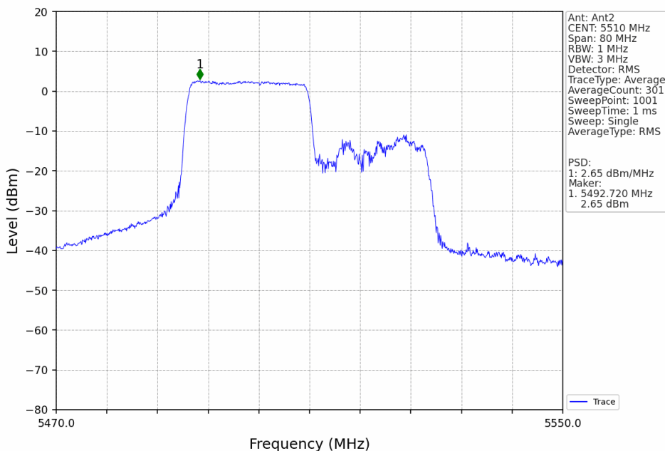
802.11ax(HEW40)_LCH_5510MHz_RU242_Left_MIMO_NTNV
