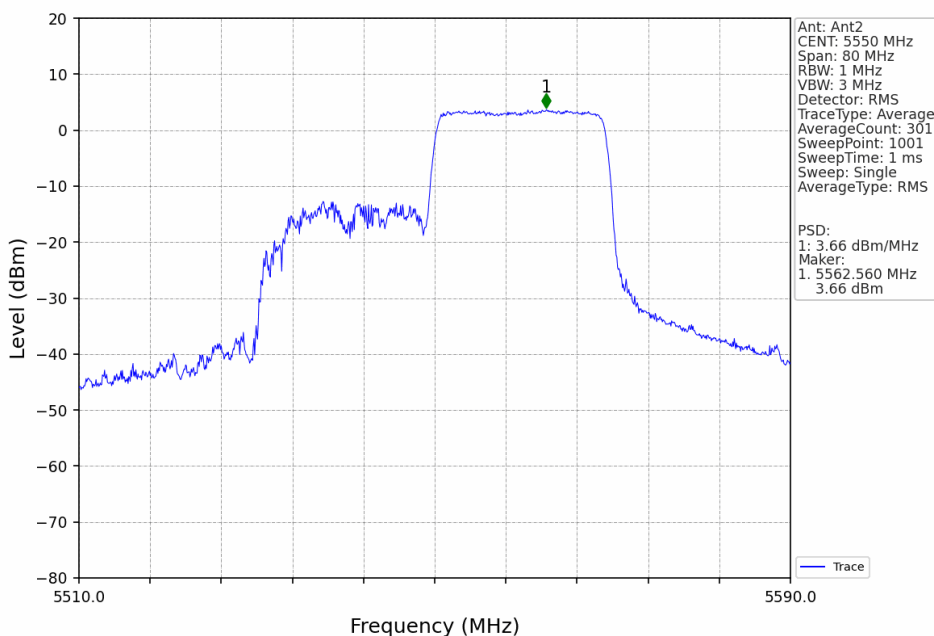
802.11ax(HEW40)_MCH_5550MHz_RU242_Right_MIMO_NTNV
