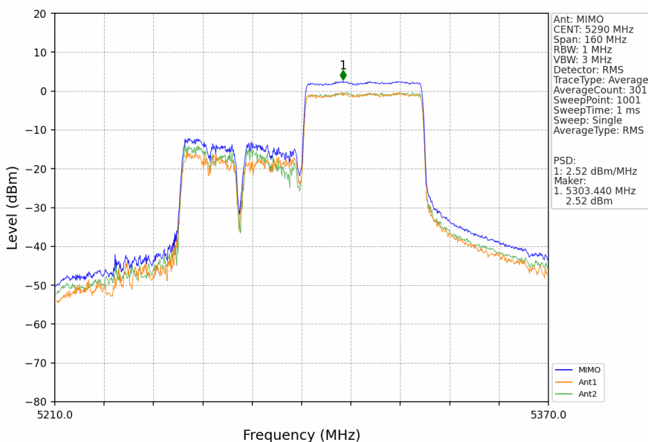
802.11ax(HEW80)_MCH_5290MHz_RU484_Right_MIMO_NTNV
