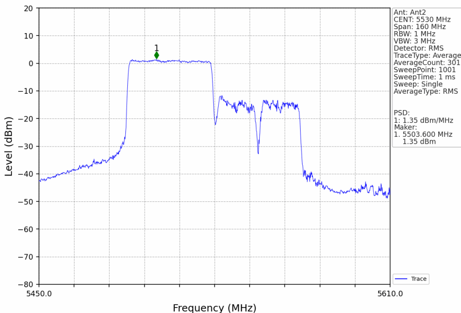
802.11ax(HEW80)_LCH_5530MHz_RU484_Left_MIMO_NTNV
