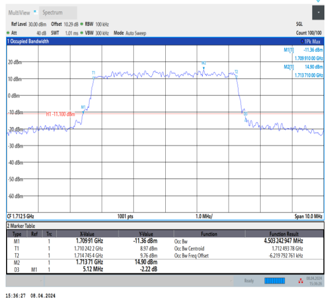
Band66-5MHz-16QAM-131997-25RB#0-PASS
