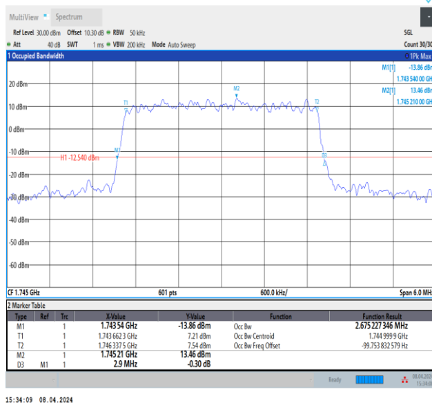
Band66-3MHz-64QAM-132322-15RB#0-PASS
