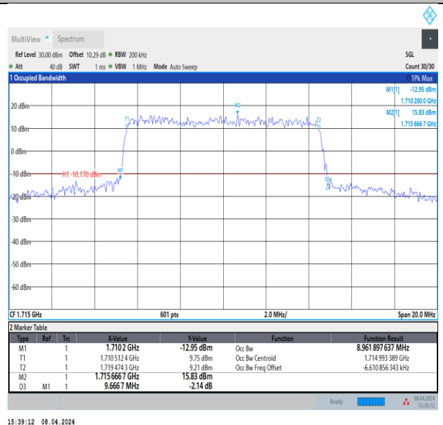
Band66-10MHz-QPSK-132022-50RB#0-PASS
