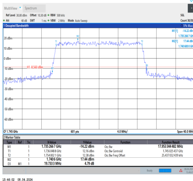
Band66-20MHz-QPSK-132322-100RB#0-PASS
