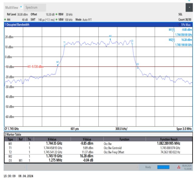
Band66-1.4MHz-QPSK-132322-6RB#0-PASS
