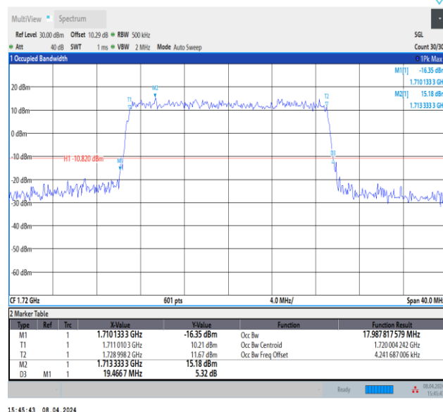
Band66-20MHz-64QAM-132072-100RB#0-PASS
