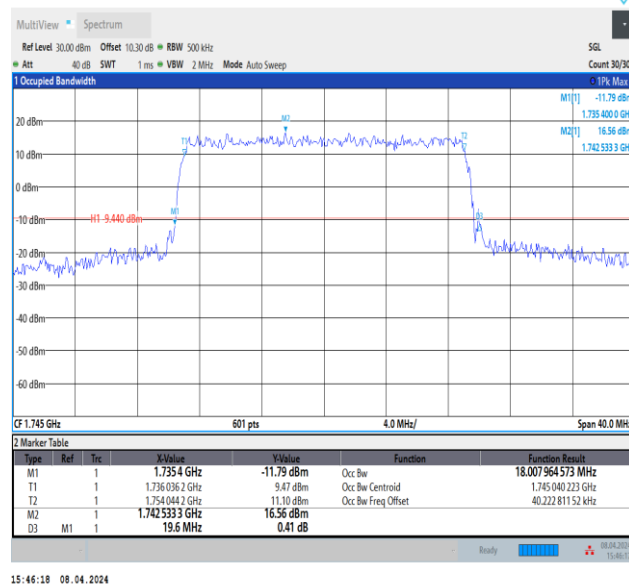
Band66-20MHz-16QAM-132322-100RB#0-PASS
