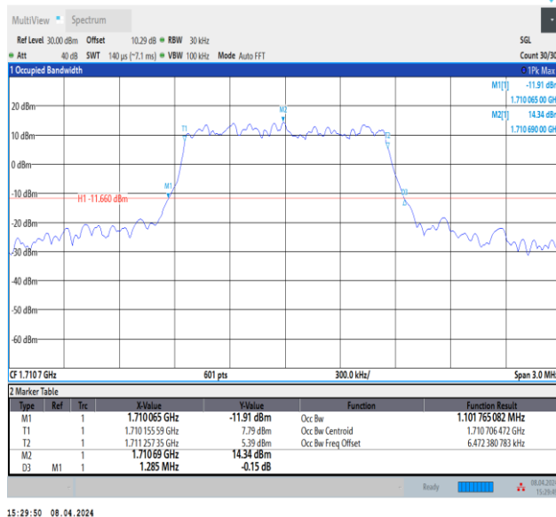
Band66-1.4MHz-64QAM-131979-6RB#0-PASS
