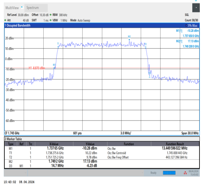
Band66-15MHz-QPSK-132322-75RB#0-PASS
