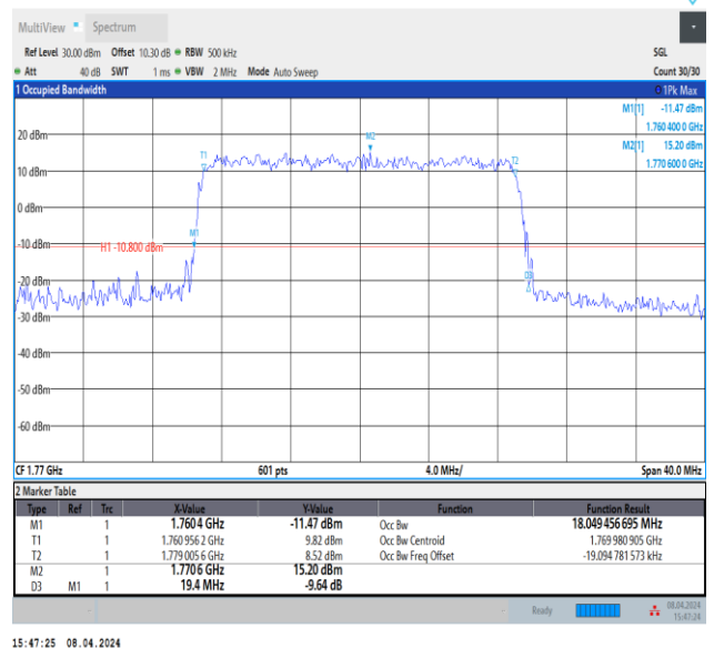
Band66-20MHz-64QAM-132572-100RB#0-PASS
