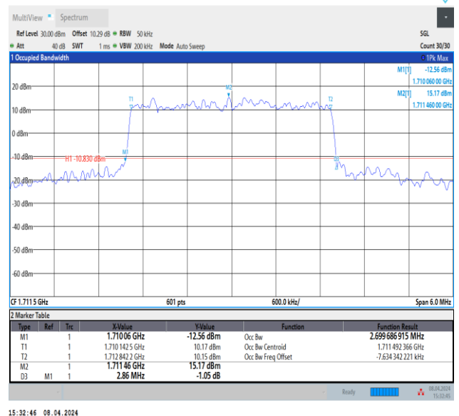
Band66-3MHz-QPSK-131987-15RB#0-PASS
