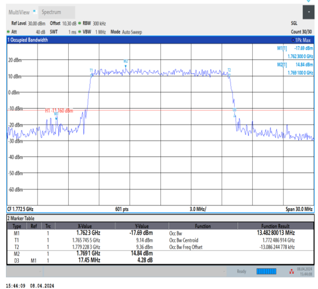
Band66-15MHz-16QAM-132597-75RB#0-PASS
