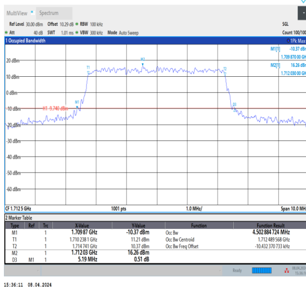
Band66-5MHz-QPSK-131997-25RB#0-PASS
