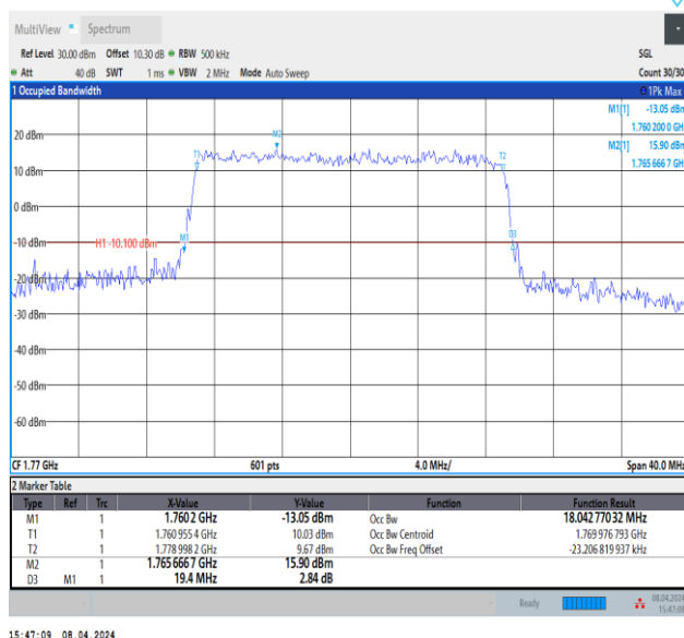
Band66-20MHz-16QAM-132572-100RB#0-PASS
