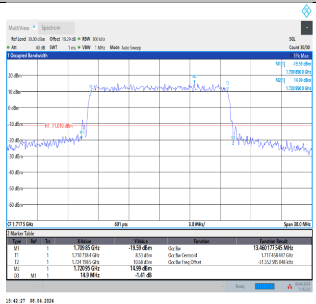
Band66-15MHz-16QAM-132047-75RB#0-PASS
