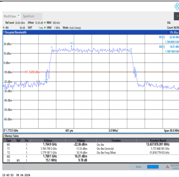
Band66-15MHz-QPSK-132597-75RB#0-PASS
