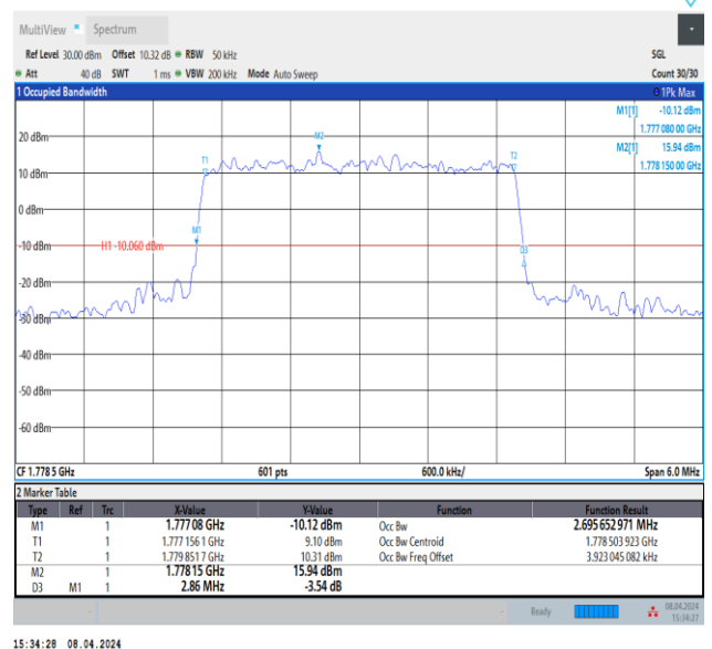
Band66-3MHz-QPSK-132657-15RB#0-PASS
