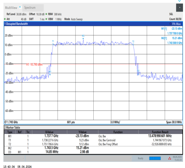
Band66-15MHz-64QAM-132322-75RB#0-PASS
