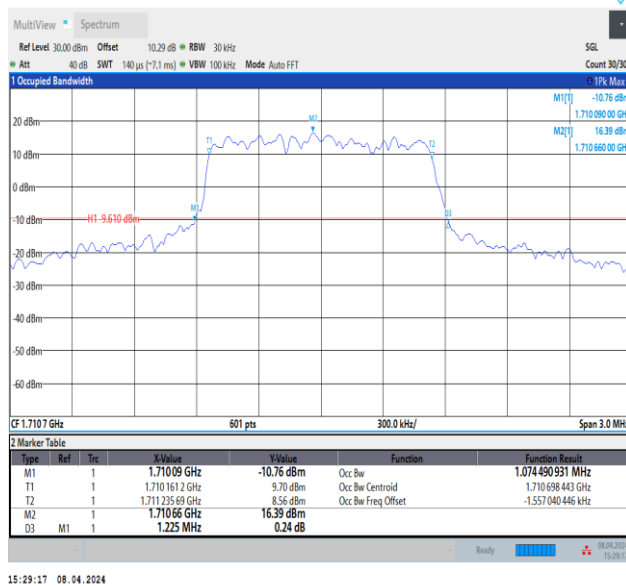
Band66-1.4MHz-QPSK-131979-6RB#0-PASS
