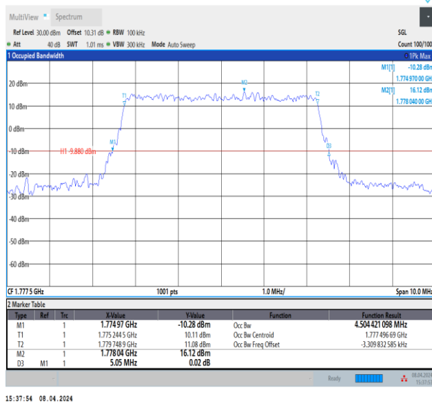
Band66-5MHz-QPSK-132647-25RB#0-PASS
