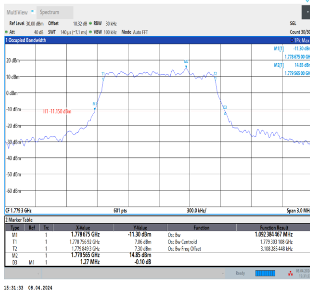
Band66-1.4MHz-64QAM-132665-6RB#0-PASS
