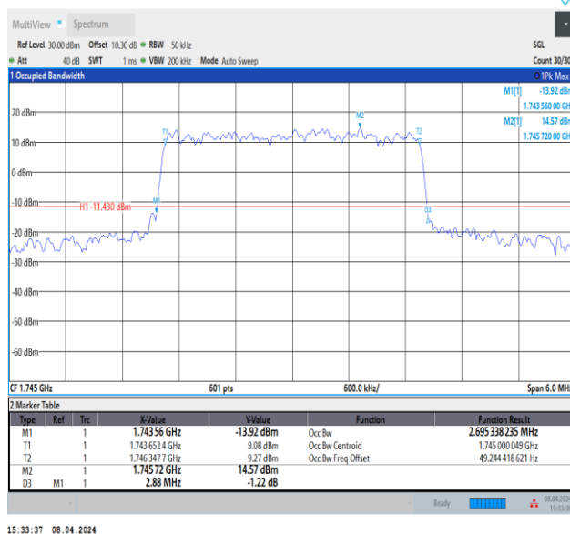
Band66-3MHz-QPSK-132322-15RB#0-PASS
