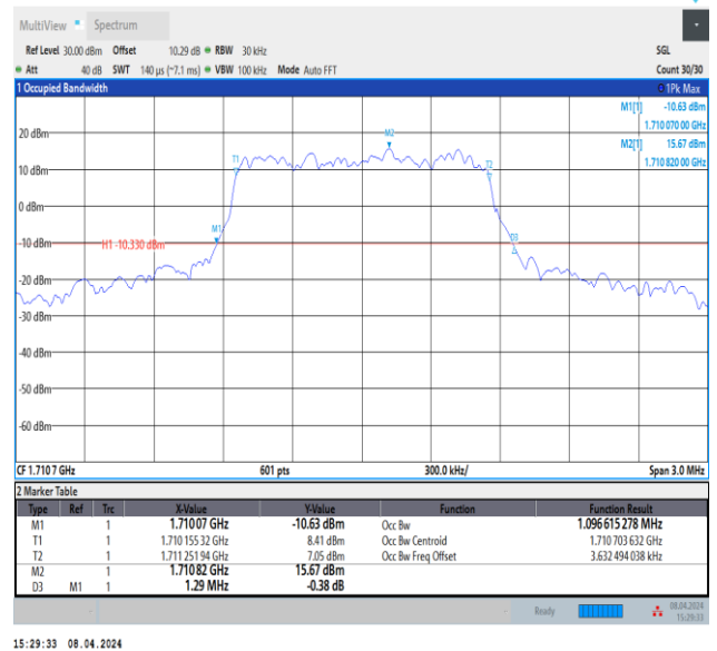
Band66-1.4MHz-16QAM-131979-6RB#0-PASS
