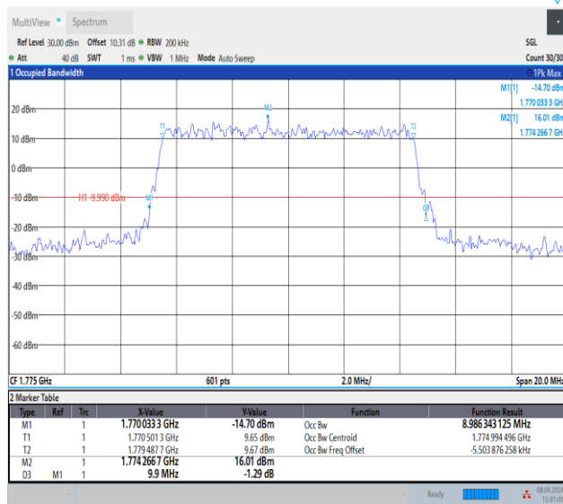
Band66-10MHz-16QAM-132622-50RB#0-PASS
