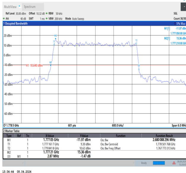
Band66-3MHz-16QAM-132657-15RB#0-PASS
