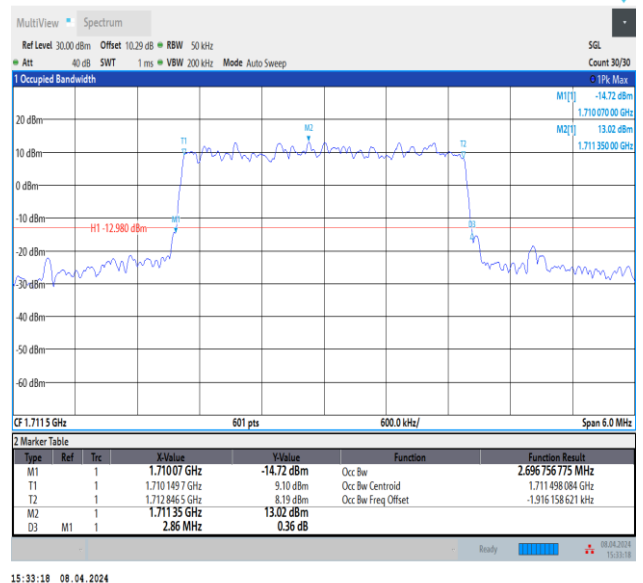
Band66-3MHz-64QAM-131987-15RB#0-PASS
