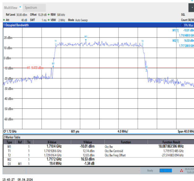
Band66-20MHz-16QAM-132072-100RB#0-PASS
