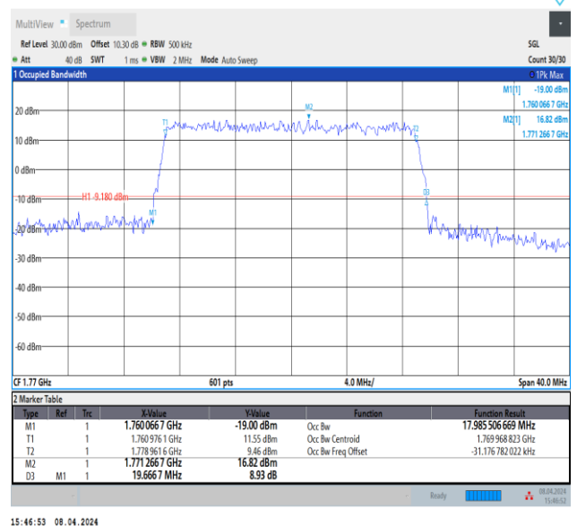
Band66-20MHz-QPSK-132572-100RB#0-PASS
