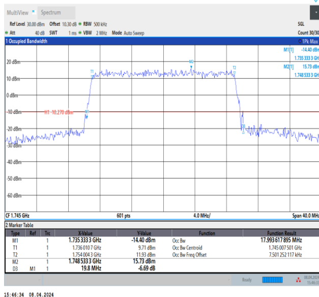
Band66-20MHz-64QAM-132322-100RB#0-PASS
