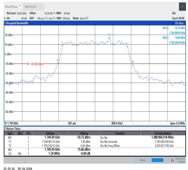
Band66-1.4MHz-64QAM-132322-6RB#0-PASS
