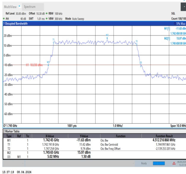
Band66-5MHz-16QAM-132322-25RB#0-PASS
