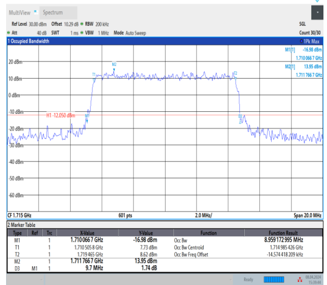
Band66-10MHz-64QAM-132022-50RB#0-PASS
