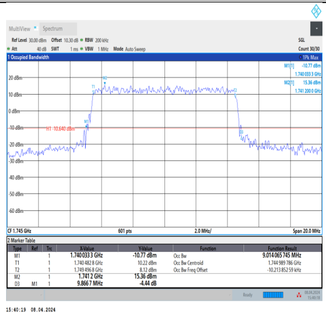
Band66-10MHz-16QAM-132322-50RB#0-PASS
