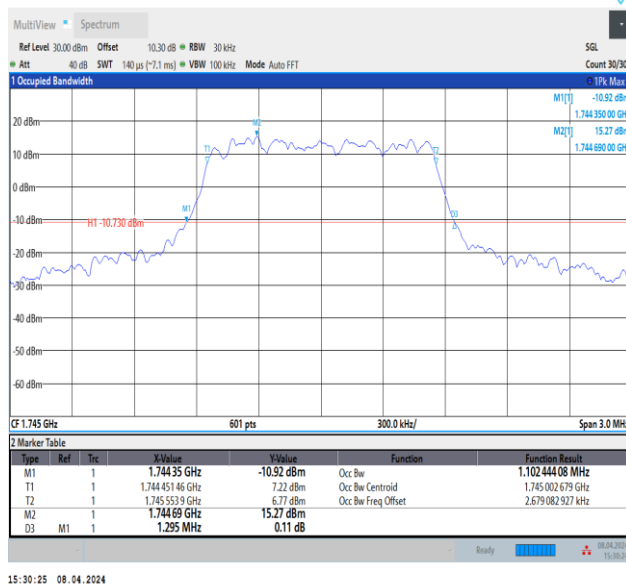
Band66-1.4MHz-16QAM-132322-6RB#0-PASS
