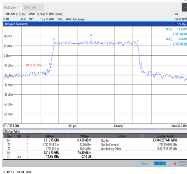
Band66-15MHz-QPSK-132047-75RB#0-PASS
