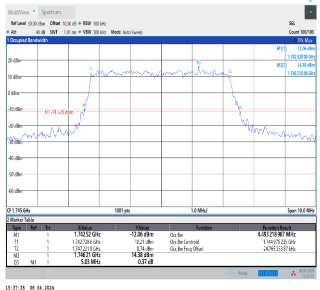
Band66-5MHz-64QAM-132322-25RB#0-PASS
