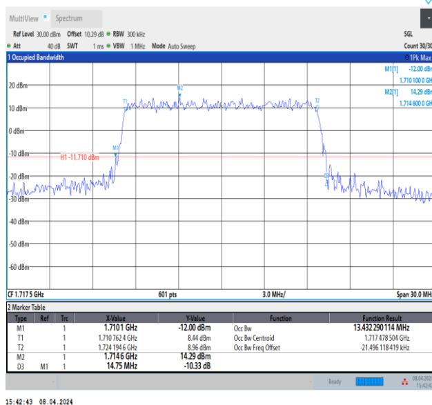
Band66-15MHz-64QAM-132047-75RB#0-PASS
