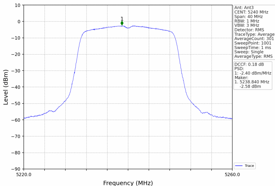
802.11ac(VHT20)_HCH_5240MHz_Ant3_NTNV
