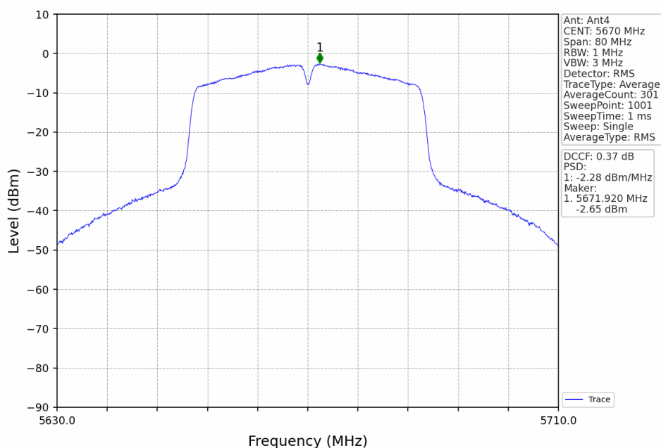
802.11n(HT40)_HCH_5670MHz_Ant4_NTNV
