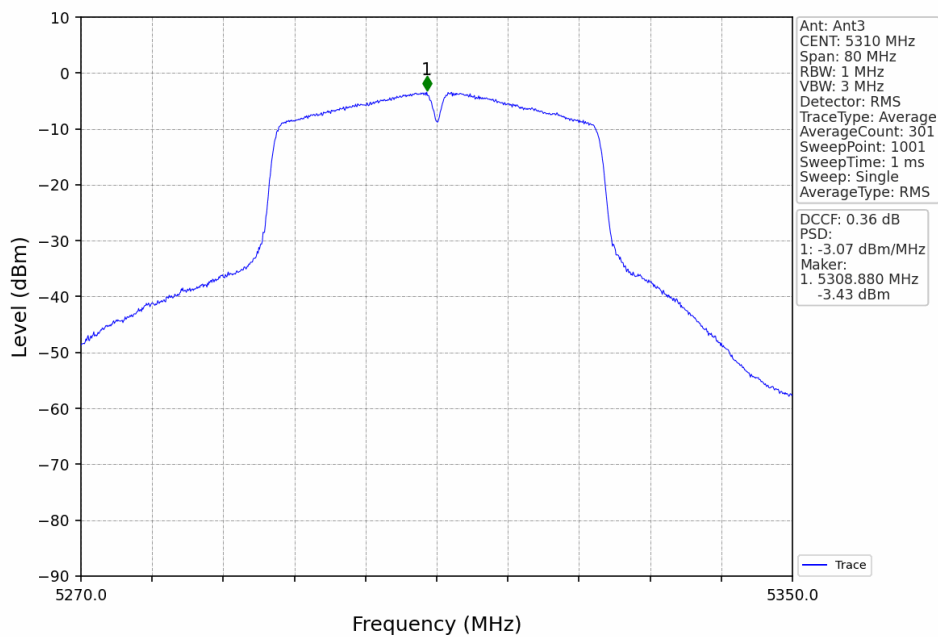
802.11n(HT40)_HCH_5310MHz_Ant3_NTNV
