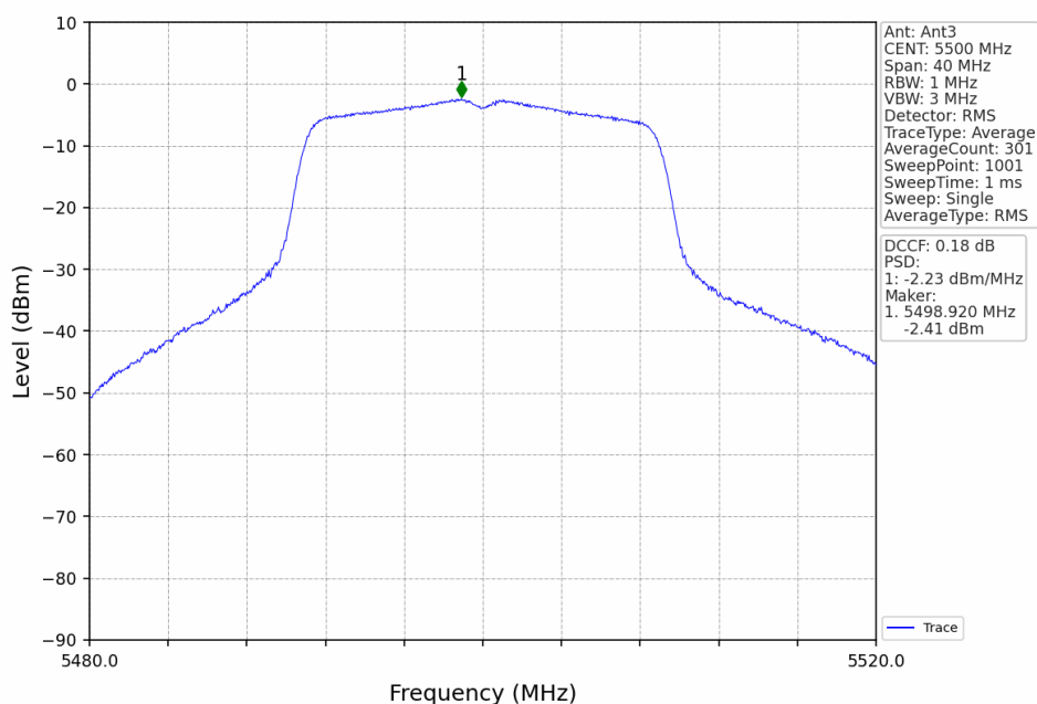
802.11ac(VHT20)_LCH_5500MHz_Ant3_NTNV
