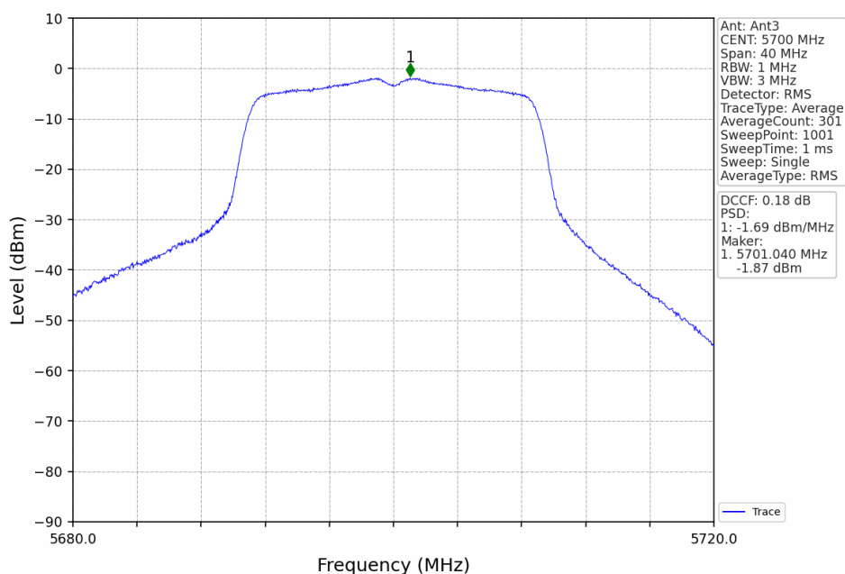
802.11n(HT20)_HCH_5700MHz_Ant3_NTNV
