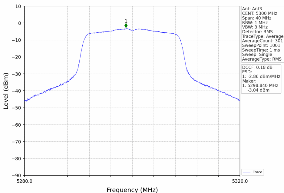
802.11ac(VHT20)_MCH_5300MHz_Ant3_NTNV
