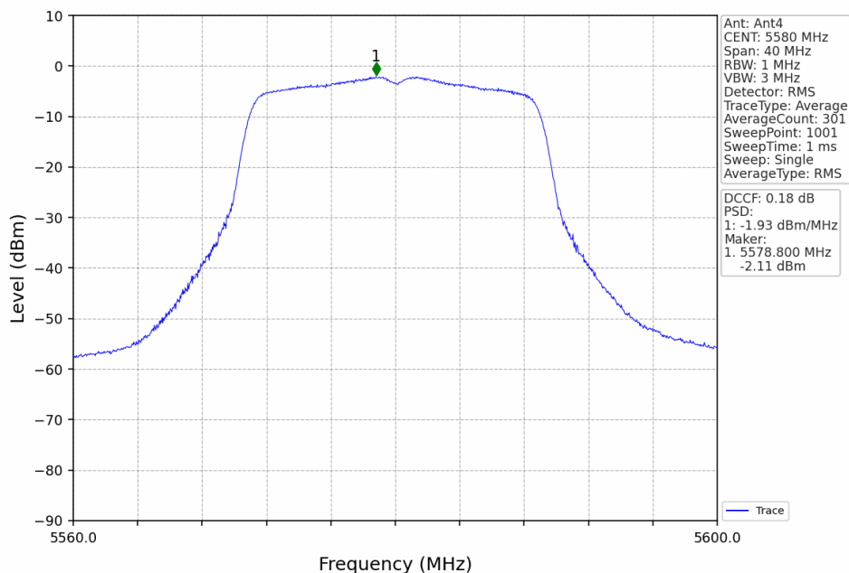
802.11ac(VHT20)_MCH_5580MHz_Ant4_NTNV
