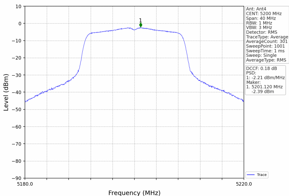
802.11ac(VHT20)_MCH_5200MHz_Ant4_NTNV
