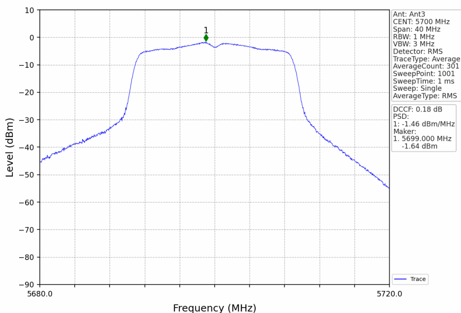
802.11ac(VHT20)_HCH_5700MHz_Ant3_NTNV
