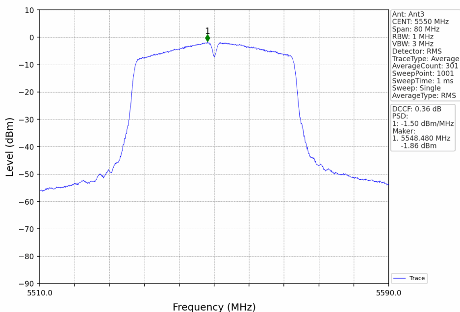
802.11n(HT40)_MCH_5550MHz_Ant3_NTNV
