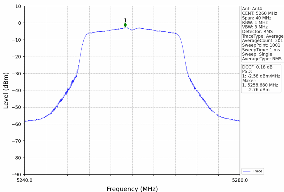
802.11ac(VHT20)_LCH_5260MHz_Ant4_NTNV
