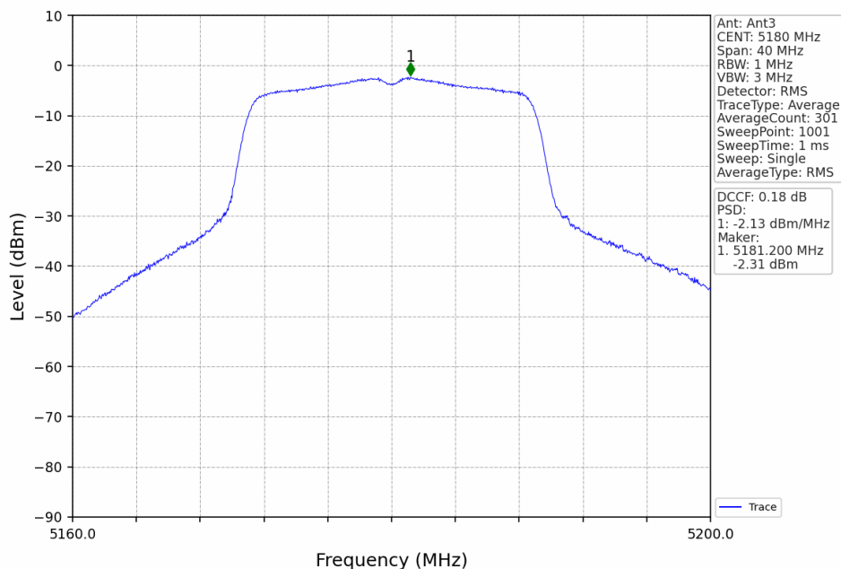
802.11ac(VHT20)_LCH_5180MHz_Ant3_NTNV
