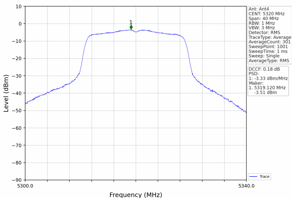
802.11ac(VHT20)_HCH_5320MHz_Ant4_NTNV
