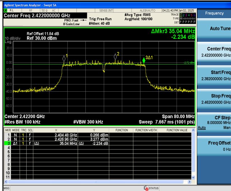
11N40SISO-Ant1-2422-PASS
