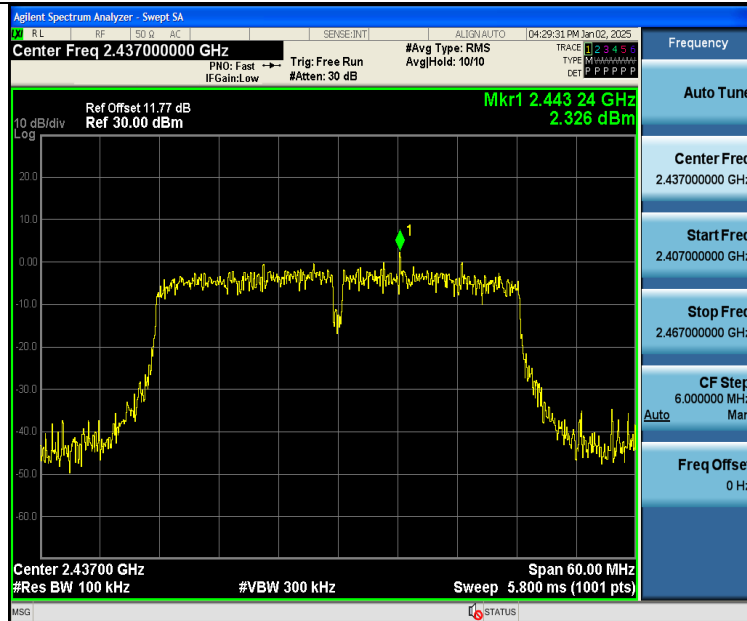
11N40SISO-Ant1-2437-0~Reference-PASS
