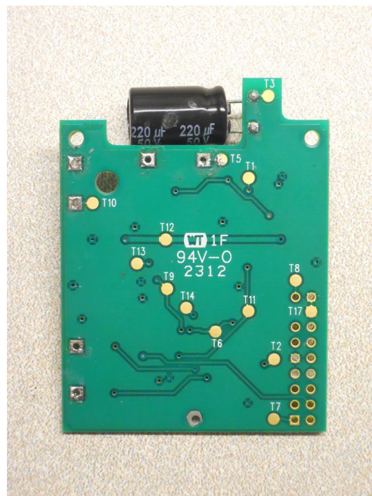
Inner Circuit Board Bottom View
