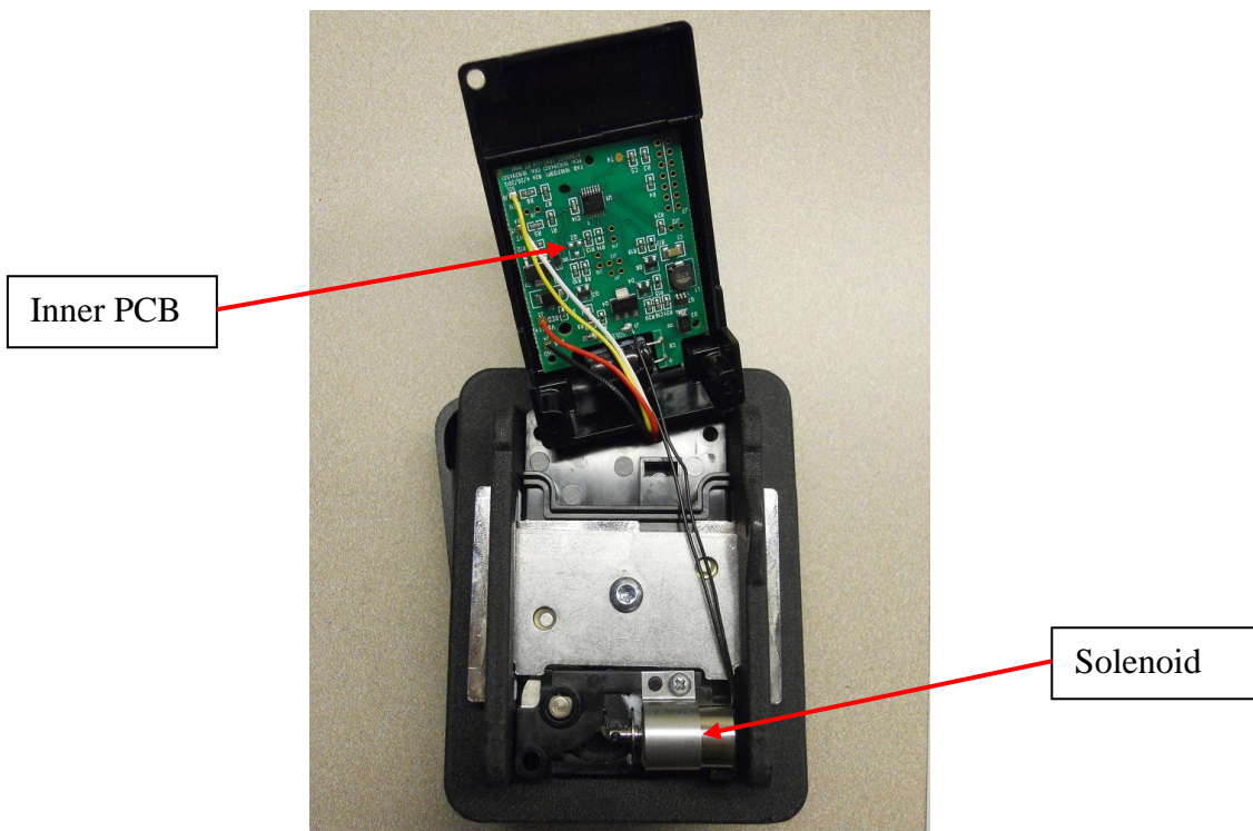
Inside Back Cover (Potting compound removed)
