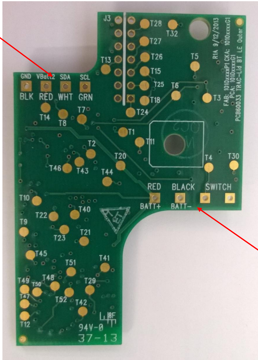
Outer Circuit Board Bottom View
