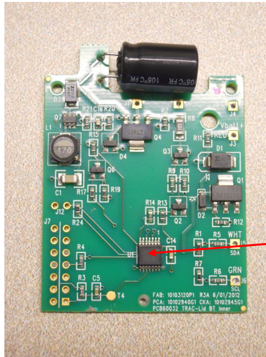
Inner Circuit Board Top View
