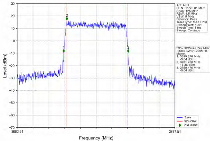
n77a_30kHz_SISO_NTNV_50MHz_CP-OFDM_64_QAM_3725.01MHz_Outer_Full
