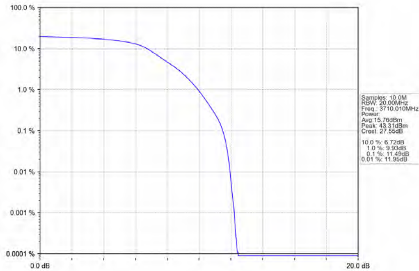
n77a_30kHz_SISO_NTNV_20MHz_DFT-s-OFDM QPSK_3710.01MHz_Outer_Full
