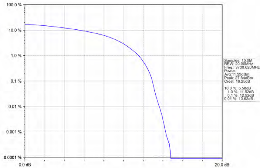
n77a_30kHz_SISO_NTNV_60MHz_DFT-s-OFDM_QPSK_3730.02MHz_Outer_Full
