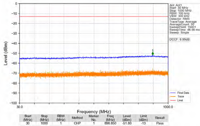
n77a_30kHz_SISO_NTNV_20MHz_CP-OFDM_QPSK_3840MHz_Edge_1RB_Left
