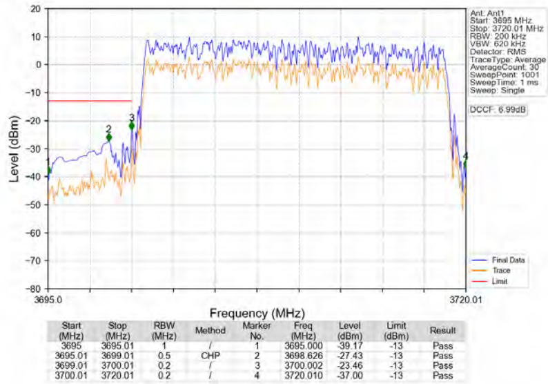
n77a_30kHz_SISO_NTNV_20MHz_DFT-s-OFDM_QPSK_3710.01MHz_Outer_Full
