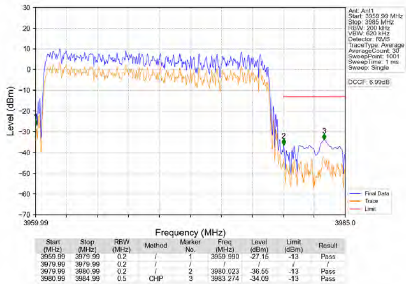
n77a_30kHz_SISO_NTNV_20MHz_DFT-s-OFDM_QPSK_3969.99MHz_Outer_Full
