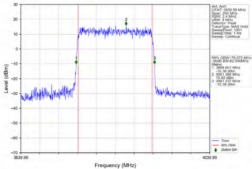
n77a_30kHz_SISO_NTNV_80MHz_CP-OFDM_QPSK_3939.99MHz_Outer_Full
