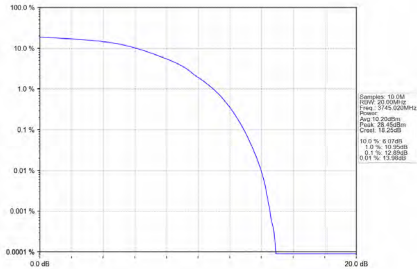
n77a_30kHz_SISO_NTNV_90MHz_DFT-s-OFDM QPSK_3745.02MHz_Outer_Full
