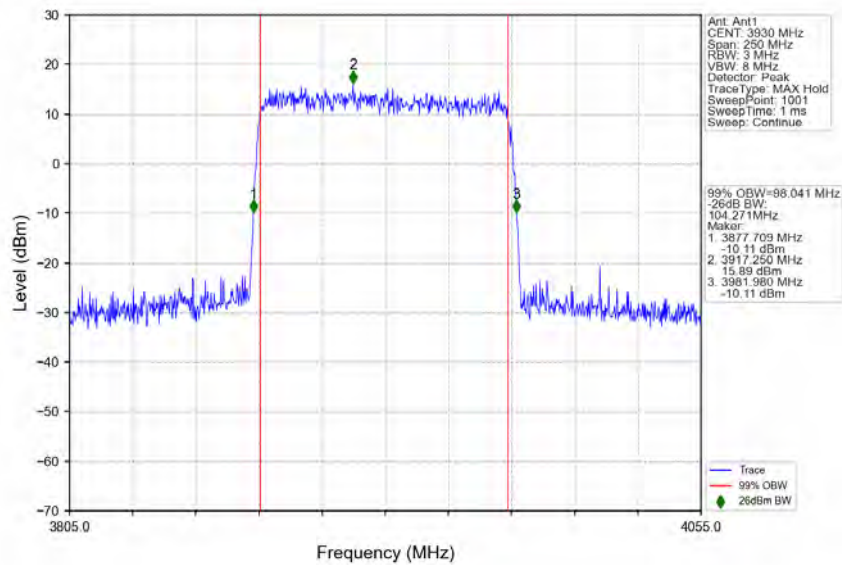
n77a_30kHz_SISO_NTNV_100MHz_CP-OFDM_64_QAM_3930MHz_Outer_Full
