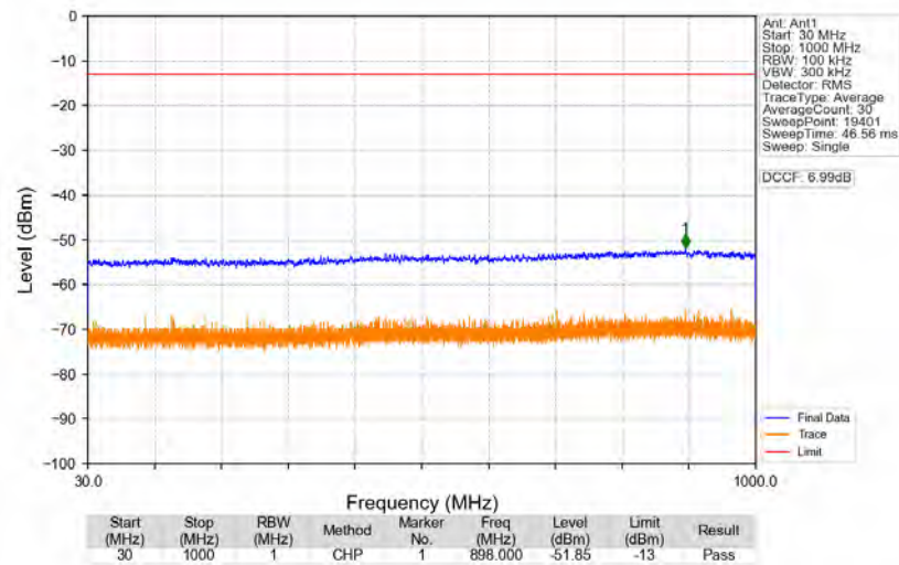
n77a_30kHz_SISO_NTNV_20MHz_DFT-s-OFDM_QPSK_3969.99MHz_Edge_1RB_Right
