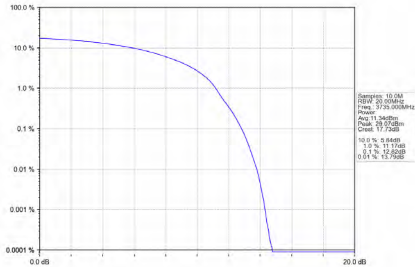
n77a_30kHz_SISO_NTNV_70MHz_DFT-s-OFDM_QPSK_3735MHz_Outer_Full
