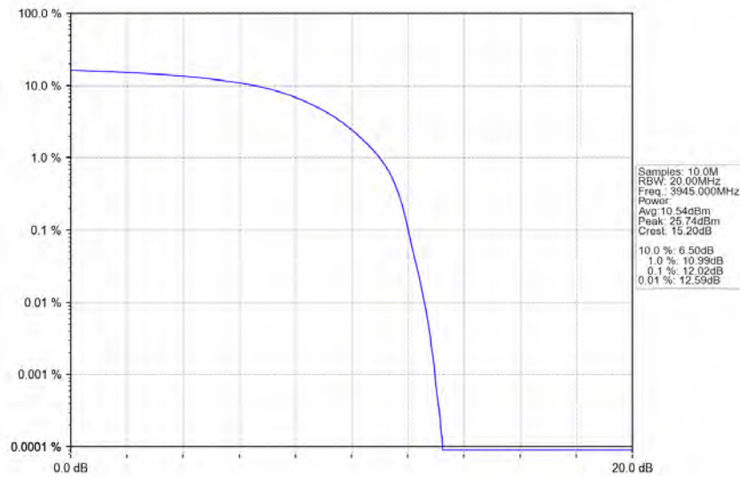
n77a_30kHz_SISO_NTNV_70MHz_DFT-s-OFDM_PI/2_BPSK_3945MHz_Outer_Full
