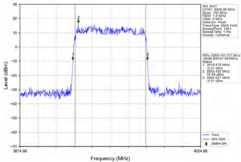
n77a_30kHz_SISO_NTNV_60MHz_DFT-s-OFDM_64_QAM_3949.98MHz_Outer_Full
