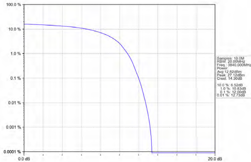
n77a_30kHz_SISO_NTNV_40MHz_DFT-s-OFDM_QPSK_3840MHz_Outer_Full
