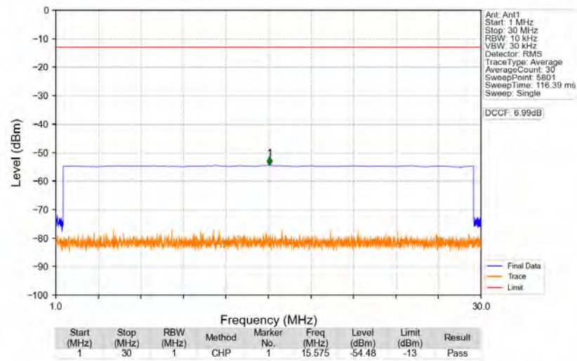
n77a_30kHz_SISO_NTNV_20MHz_DFT-s-OFDM_QPSK_3969.99MHz_Edge_1RB_Right
