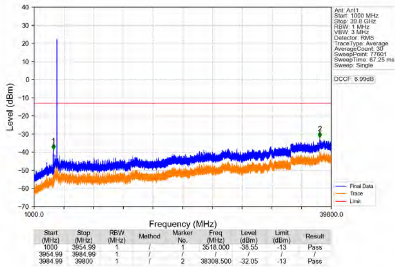
n77a_30kHz_SISO_NTNV_20MHz_DFT-s-OFDM_PI/2_BPSK_3969.99MHz_Edge_1RB_Right
