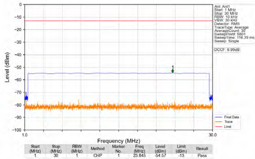
n77a_30kHz_SISO_NTNV_20MHz_DFT-s-OFDM_QPSK_3710.01MHz_Edge_1RB_Left
