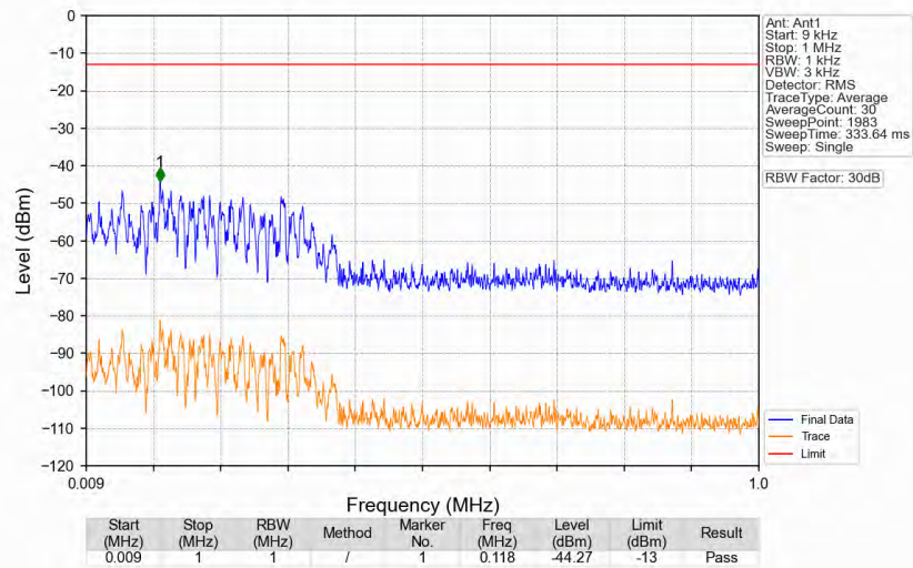
n77a_30kHz_SISO_NTNV_20MHz_DFT-s-OFDM_QPSK_3969.99MHz_Edge_1RB_Right
