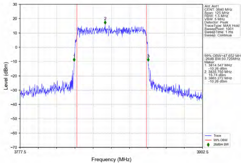
n77a_30kHz_SISO_NTNV_50MHz_CP-OFDM_16_QAM_3840MHz_Outer_Full
