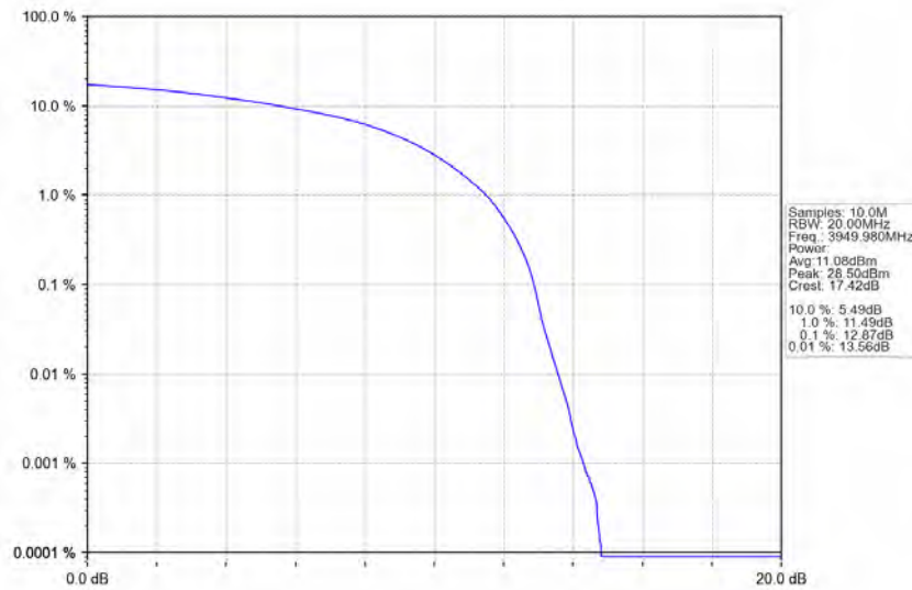
n77a_30kHz_SISO_NTNV_60MHz_DFT-s-OFDM_QPSK_3949.98MHz_Outer_Full
