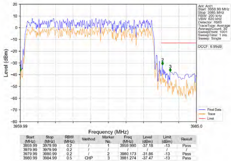
n77a_30kHz_SISO_NTNV_20MHz_DFT-s-OFDM_PI/2_BPSK_3969.99MHz_Outer_Full
