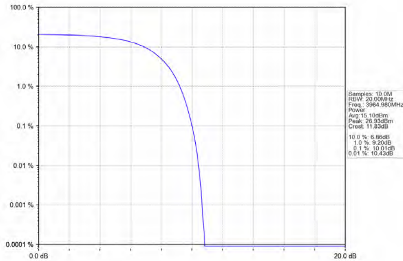
n77a_30kHz_SISO_NTNV_30MHz_DFT-s-OFDM_PI/2_BPSK_3964.98MHz_Outer_Full
