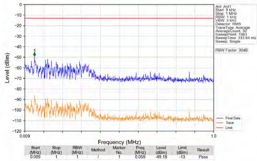
n77a_30kHz_SISO_NTNV_20MHz_DFT-s-OFDM_QPSK_3840MHz_Edge_1RB_Left
