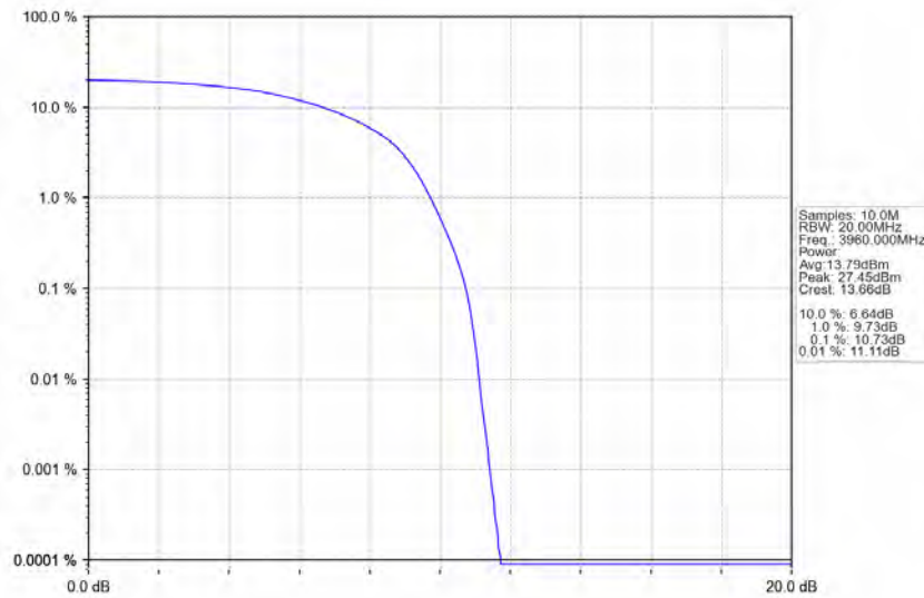
n77a_30kHz_SISO_NTNV_40MHz_DFT-s-OFDM_PI/2_BPSK_3960MHz_Outer_Full
