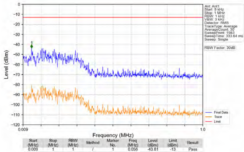
n77a_30kHz_SISO_NTNV_20MHz_DFT-s-OFDM_QPSK_3710.01MHz_Edge_1RB_Left
