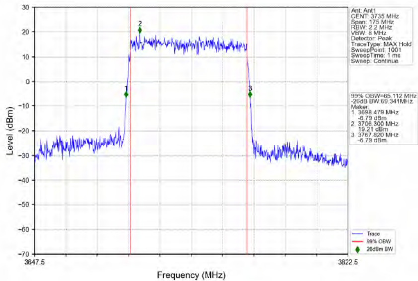
n77a_30kHz_SISO_NTNV_70MHz_DFT-s-OFDM_QPSK_3735MHz_Outer_Full
