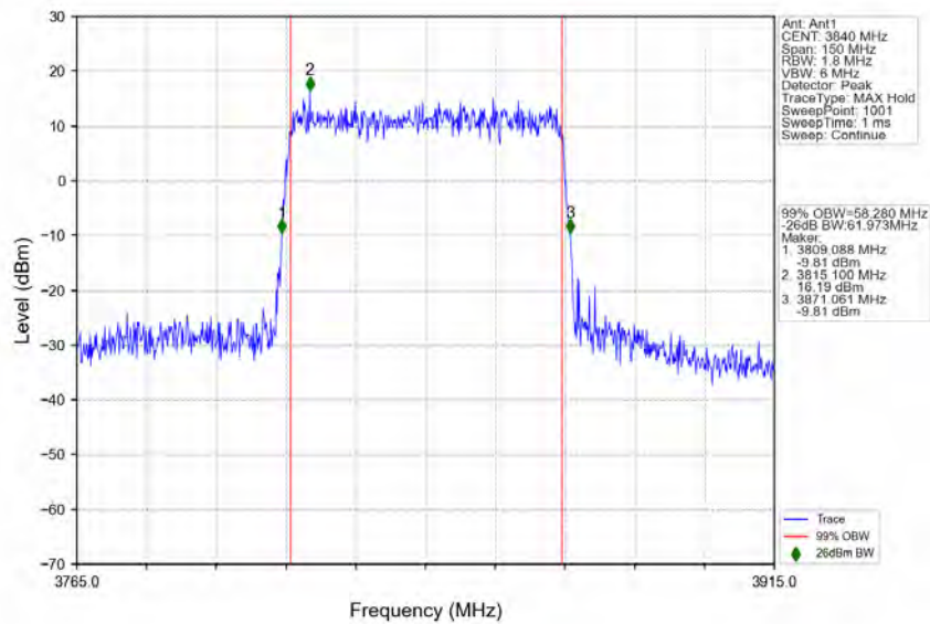
n77a_30kHz_SISO_NTNV_60MHz_CP-OFDM_16_QAM_3840MHz_Outer_Full
