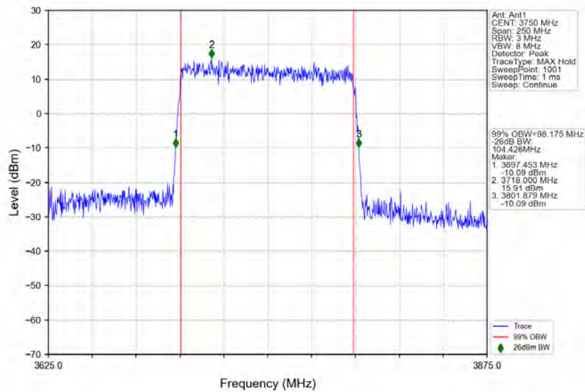
n77a_30kHz_SISO_NTNV_100MHz_CP-OFDM_64_QAM_3750MHz_Outer_Full
