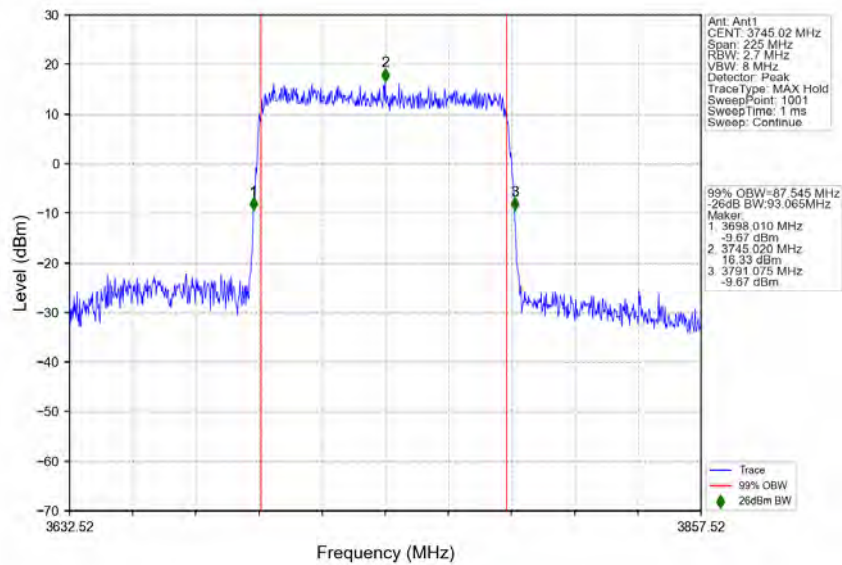
n77a_30kHz_SISO_NTNV_90MHz_DFT-s-OFDM_64_QAM_3745.02MHz_Outer_Full
