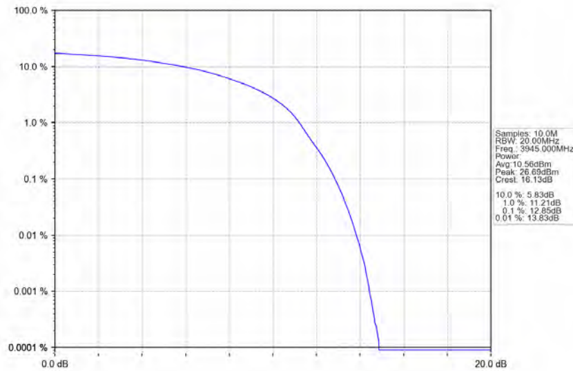
n77a_30kHz_SISO_NTNV_70MHz_DFT-s-OFDM_QPSK_3945MHz_Outer_Full
