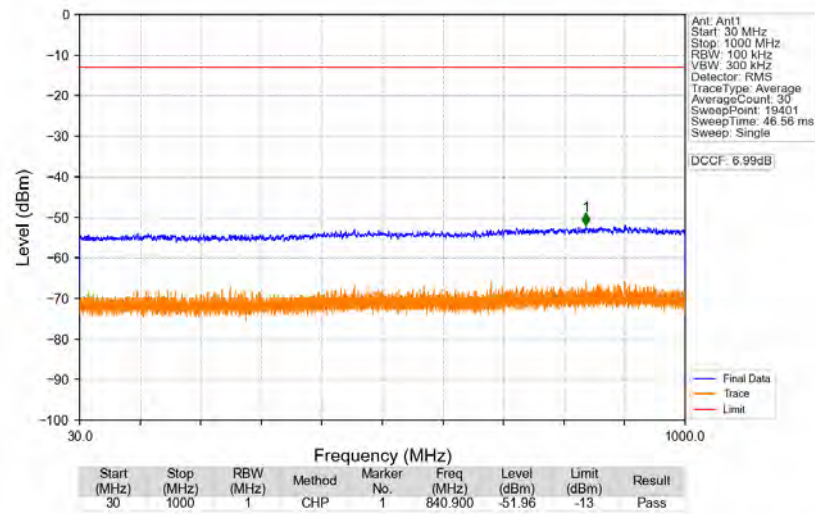
n77a_30kHz_SISO_NTNV_20MHz_DFT-s-OFDM_QPSK_3710.01MHz_Edge_1RB_Left
