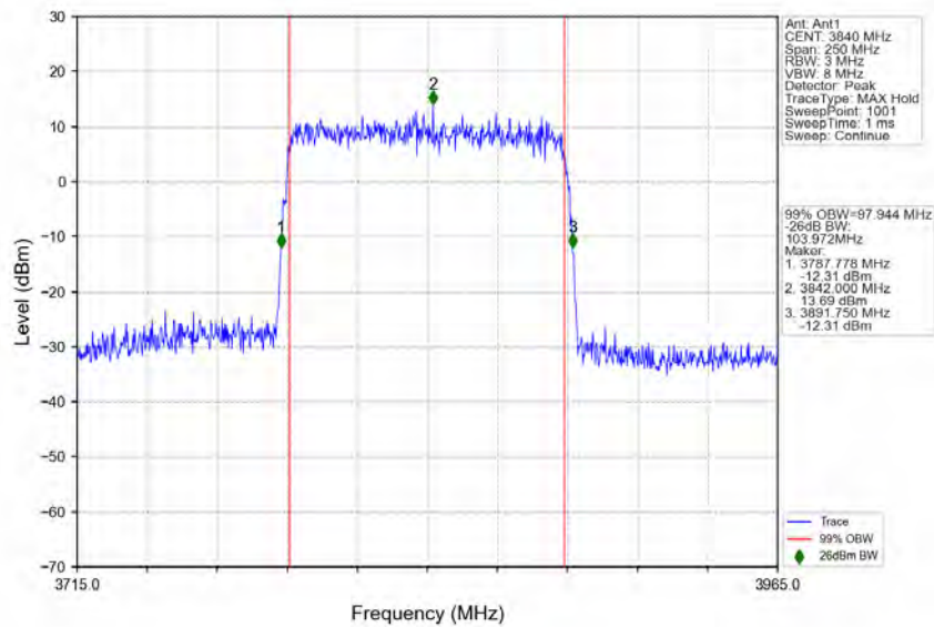
n77a_30kHz_SISO_NTNV_100MHz_CP-OFDM_256_QAM_3840MHz_Outer_Full
