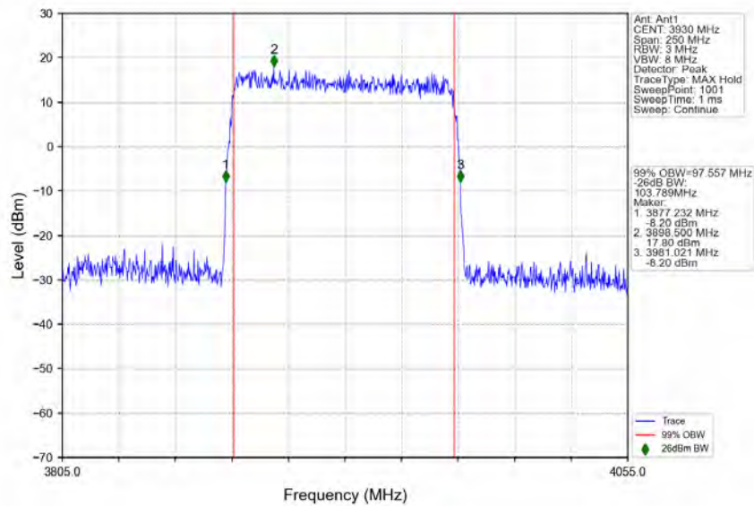
n77a_30kHz_SISO_NTNV_100MHz_DFT-s-OFDM_QPSK_3930MHz_Outer_Full
