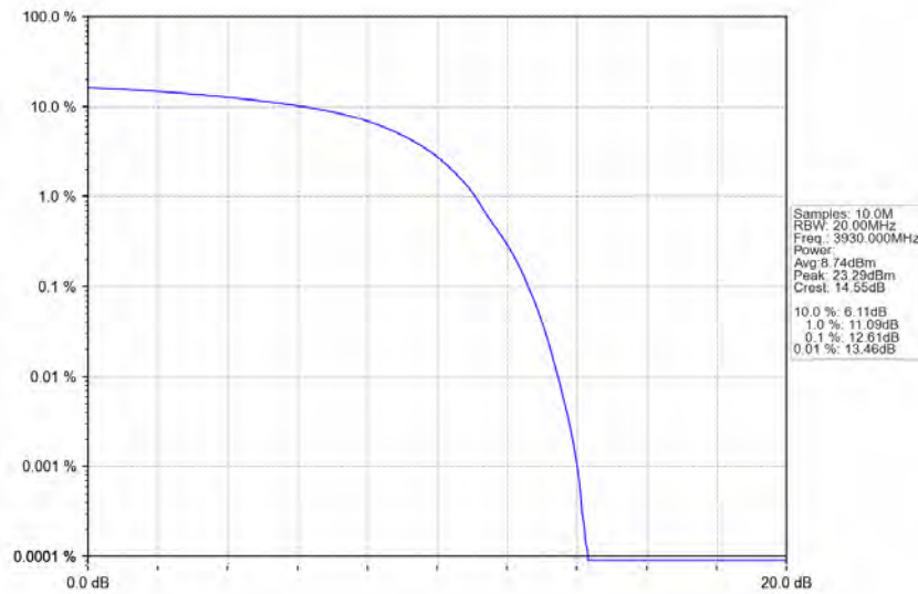
n77a_30kHz_SISO_NTNV_100MHz_DFT-s-OFDM_PI/2_BPSK_3930MHz_Outer_Full
