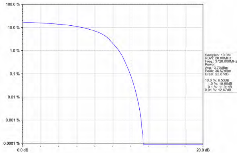
n77a_30kHz_SISO_NTNV_40MHz_DFT-s-OFDM_QPSK_3720MHz_Outer_Full
