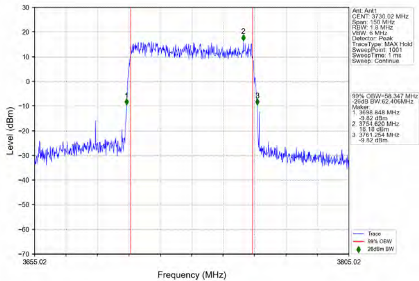
n77a_30kHz_SISO_NTNV_60MHz_DFT-s-OFDM_64_QAM_3730.02MHz_Outer_Full
