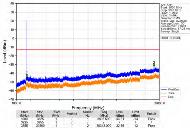
n77a_30kHz_SISO_NTNV_20MHz_CP-OFDM_QPSK_3840MHz_Edge_1RB_Left
