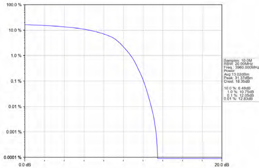
n77a_30kHz_SISO_NTNV_40MHz_DFT-s-OFDM_QPSK_3960MHz_Outer_Full
