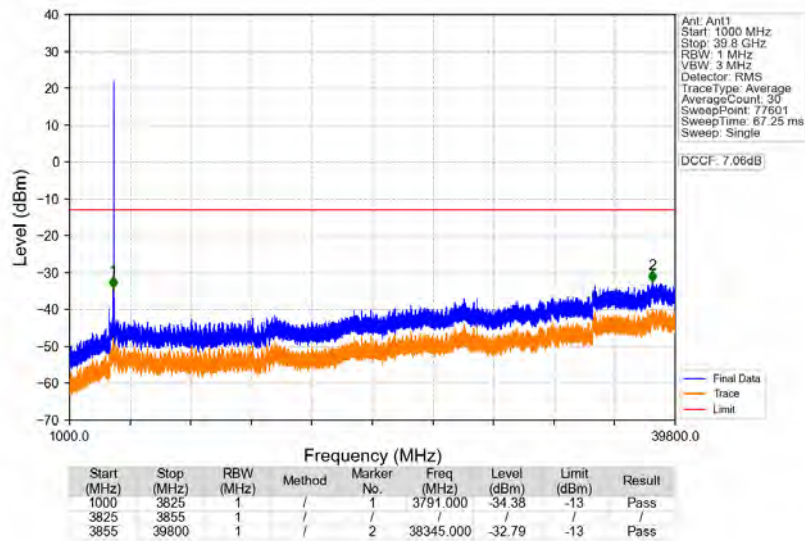
n77a_30kHz_SISO_NTNV_20MHz_DFT-s-OFDM_QPSK_3840MHz_Edge_1RB_Left
