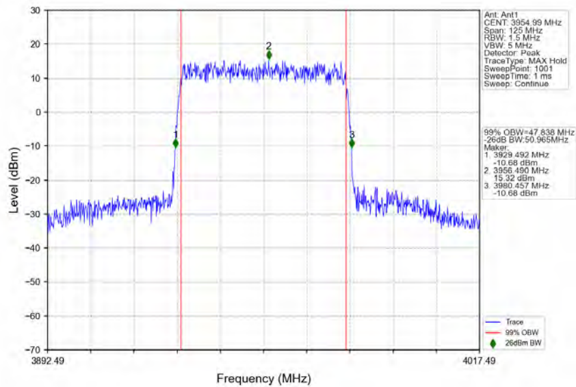
n77a_30kHz_SISO_NTNV_50MHz_CP-OFDM_QPSK_3954.99MHz_Outer_Full
