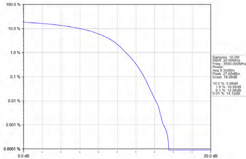
n77a_30kHz_SISO_NTNV_100MHz_DFT-s-OFDM_QPSK_3930MHz_Outer_Full
