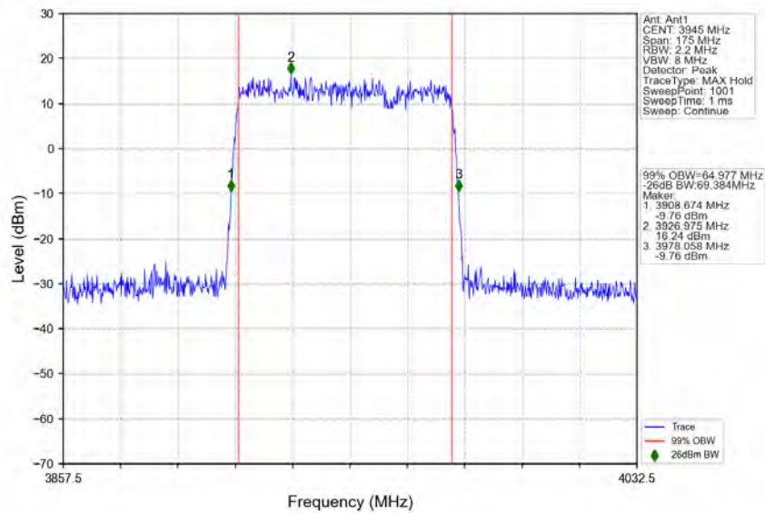
n77a_30kHz_SISO_NTNV_70MHz_DFT-s-OFDM_64_QAM_3945MHz_Outer_Full
