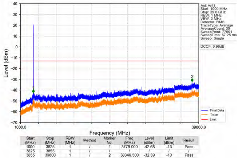
n77a_30kHz_SISO_NTNV_20MHz_DFT-s-OFDM_PI/2_BPSK_3840MHz_Edge_1RB_Left
