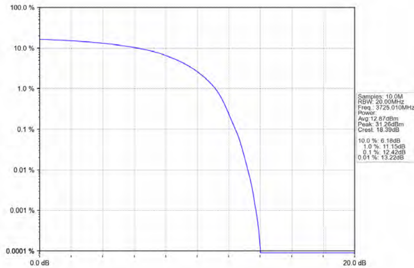
n77a_30kHz_SISO_NTNV_50MHz_DFT-s-OFDM QPSK_3725.01MHz_Outer_Full
