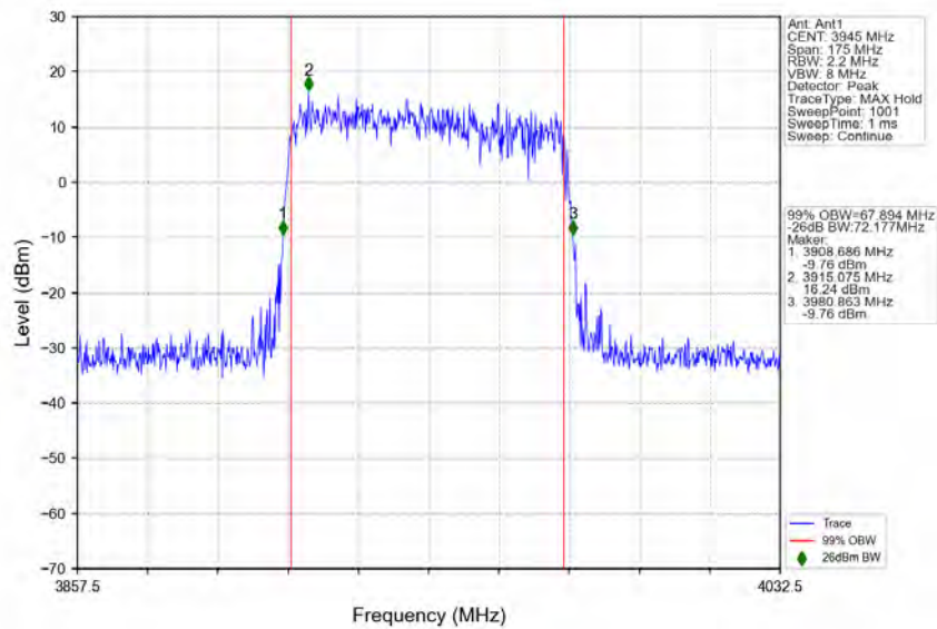
n77a_30kHz_SISO_NTNV_70MHz_CP-OFDM_64_QAM_3945MHz_Outer_Full
