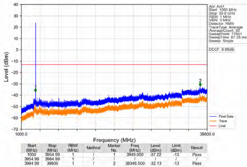
n77a_30kHz_SISO_NTNV_20MHz_DFT-s-OFDM_QPSK_3969.99MHz_Edge_1RB_Right
