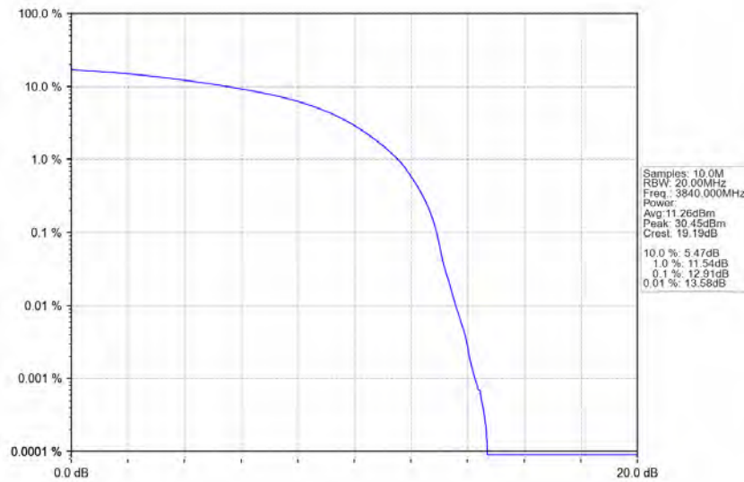
n77a_30kHz_SISO_NTNV_60MHz_DFT-s-OFDM_QPSK_3840MHz_Outer_Full
