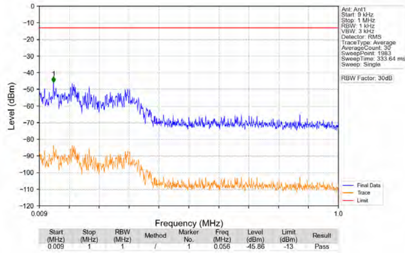
n77a_30kHz_SISO_NTNV_20MHz_DFT-s-OFDM_PI/2_BPSK_3840MHz_Edge_1RB_Left
