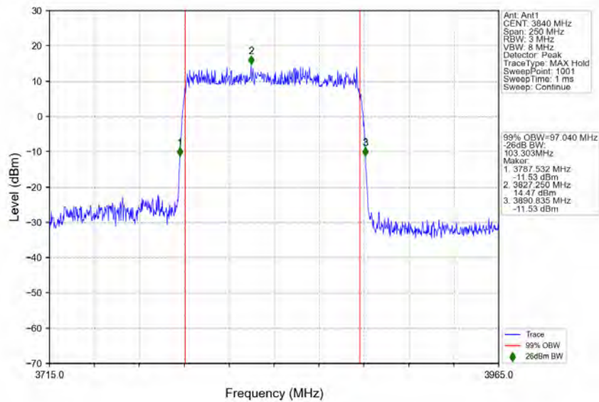
n77a_30kHz_SISO_NTNV_100MHz_DFT-s-OFDM_256_QAM_3840MHz_Outer_Full
