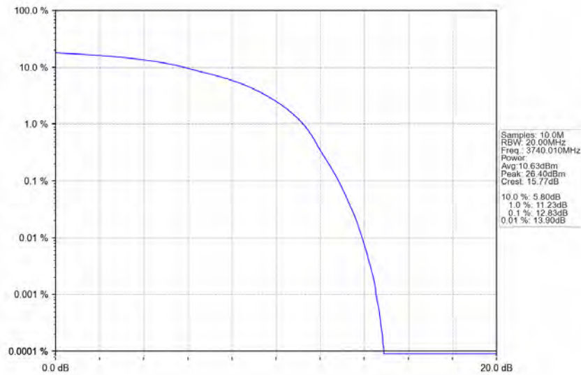
n77a_30kHz_SISO_NTNV_80MHz_DFT-s-OFDM QPSK_3740.01MHz_Outer_Full
