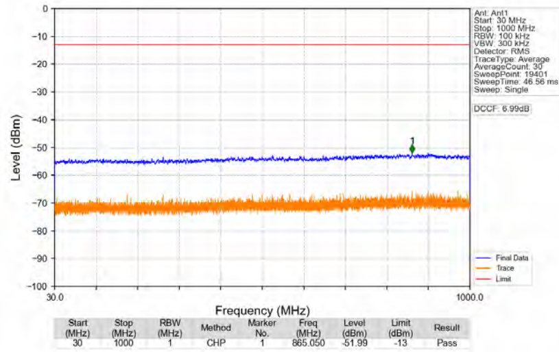
n77a_30kHz_SISO_NTNV_20MHz_DFT-s-OFDM_PI/2_BPSK_3840MHz_Edge_1RB_Left
