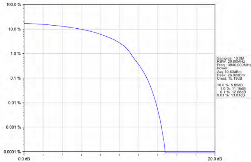
n77a_30kHz_SISO_NTNV_70MHz_DFT-s-OFDM_QPSK_3840MHz_Outer_Full
