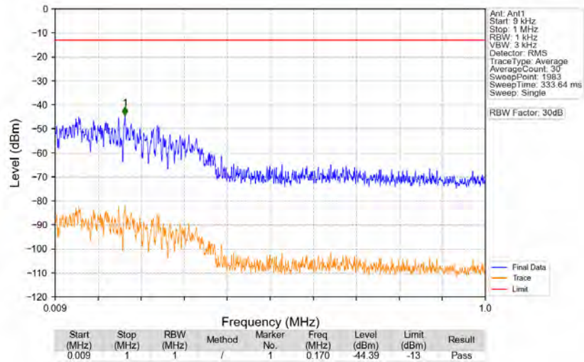
n77a_30kHz_SISO_NTNV_20MHz_CP-OFDM_QPSK_3710.01MHz_Edge_1RB_Left
