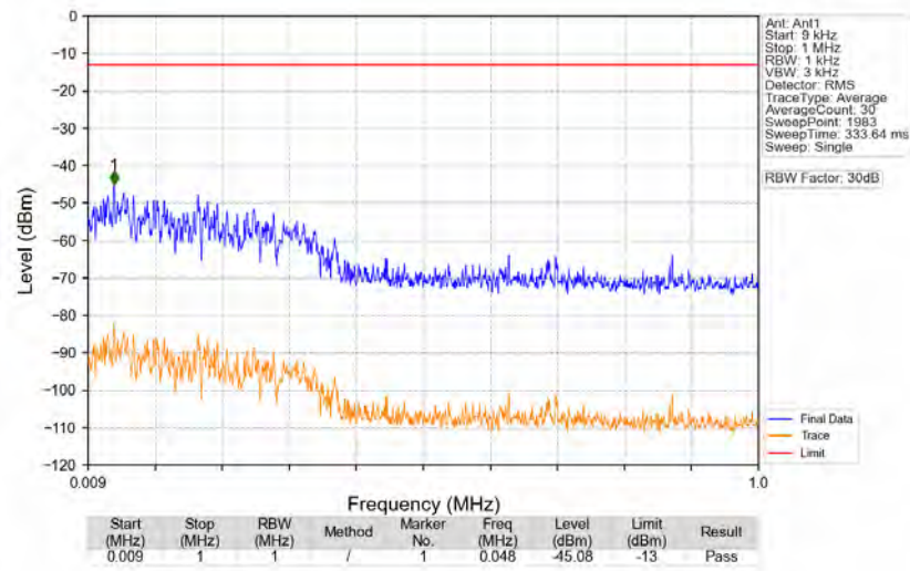
n77a_30kHz_SISO_NTNV_20MHz_CP-OFDM_QPSK_3840MHz_Edge_1RB_Left
