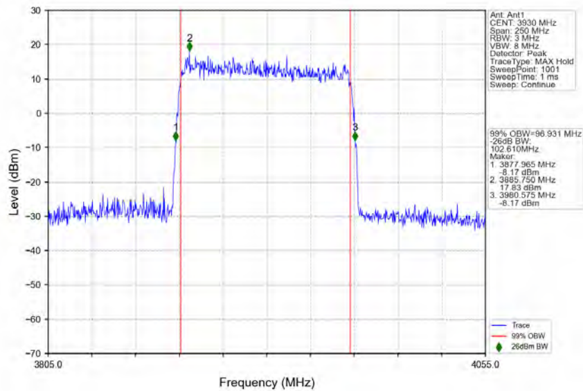
n77a_30kHz_SISO_NTNV_100MHz_DFT-s-OFDM_64_QAM_3930MHz_Outer_Full
