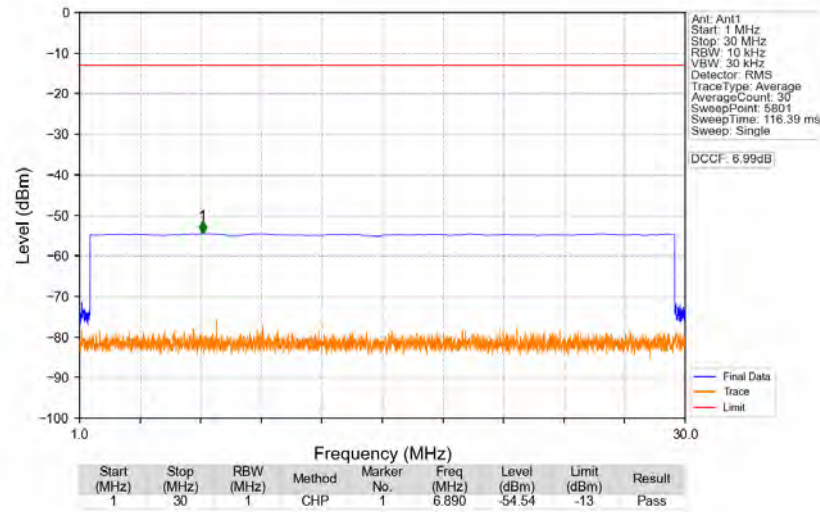
n77a_30kHz_SISO_NTNV_20MHz_DFT-s-OFDM_PI/2_BPSK_3840MHz_Edge_1RB_Left
