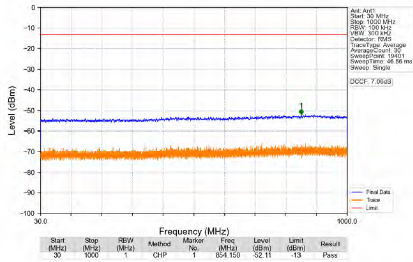
n77a_30kHz_SISO_NTNV_20MHz_DFT-s-OFDM_QPSK_3840MHz_Edge_1RB_Left
