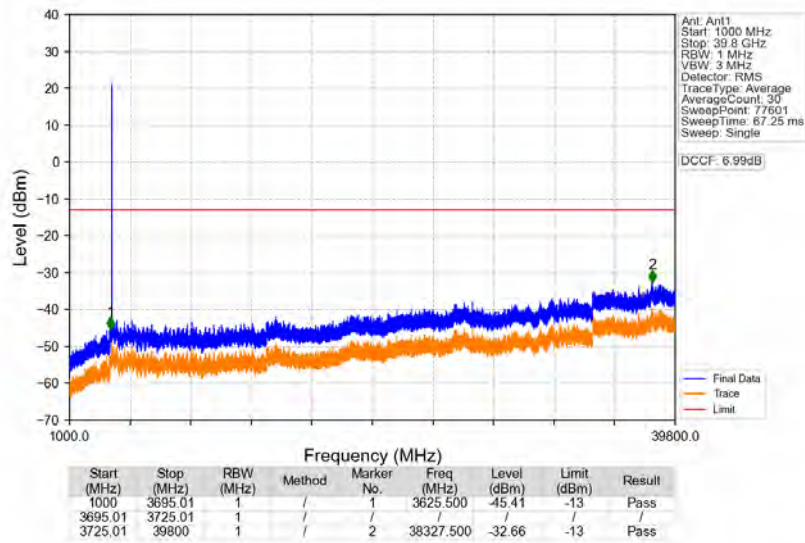
n77a_30kHz_SISO_NTNV_20MHz_DFT-s-OFDM_PI/2_BPSK_3710.01MHz_Edge_1RB_Left
