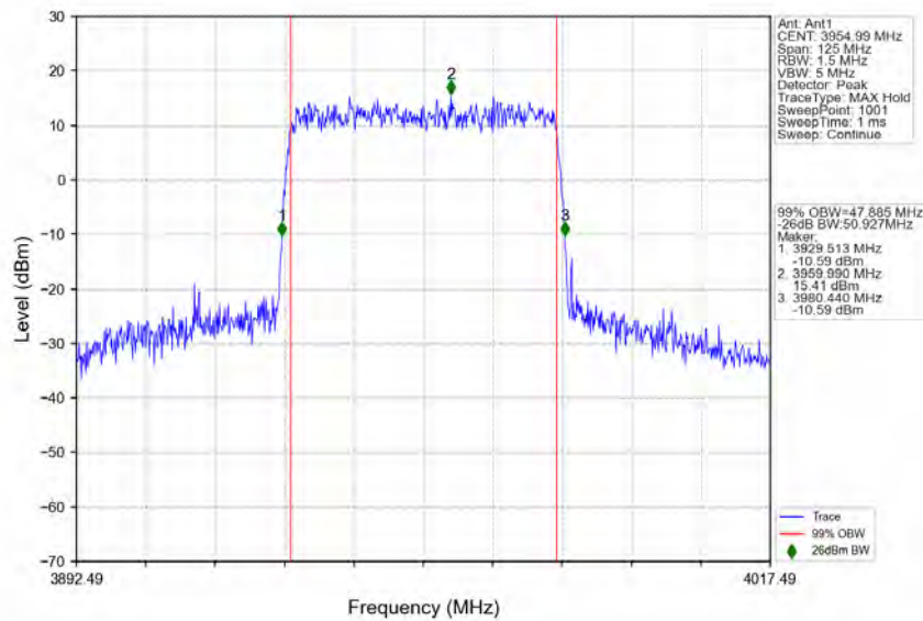
n77a_30kHz_SISO_NTNV_50MHz_CP-OFDM_64_QAM_3954.99MHz_Outer_Full
