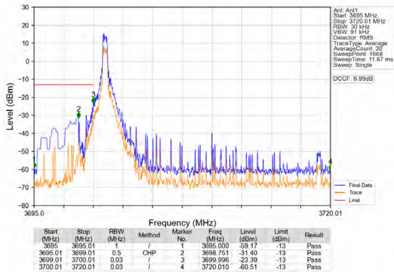
n77a_30kHz_SISO_NTNV_20MHz_DFT-s-OFDM_QPSK_3710.01MHz_Edge_1RB_Left
