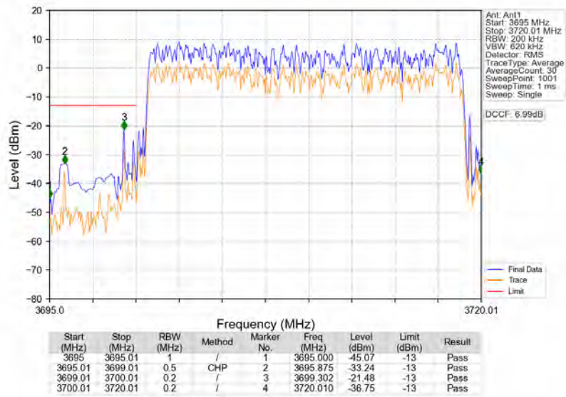
n77a_30kHz_SISO_NTNV_20MHz_DFT-s-OFDM_PI/2_BPSK_3710.01MHz_Outer_Full
