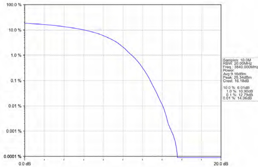
n77a_30kHz_SISO_NTNV_100MHz_DFT-s-OFDM_QPSK_3840MHz_Outer_Full
