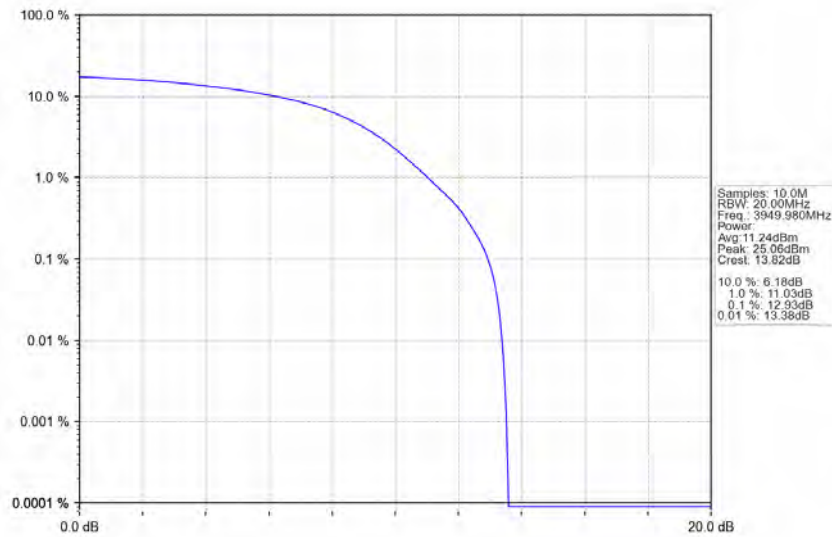
n77a_30kHz_SISO_NTNV_60MHz_DFT-s-OFDM_PI/2_BPSK_3949.98MHz_Outer_Full
