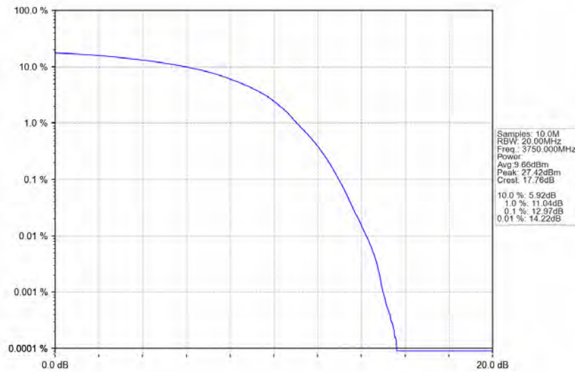
n77a_30kHz_SISO_NTNV_100MHz_DFT-s-OFDM_QPSK_3750MHz_Outer_Full
