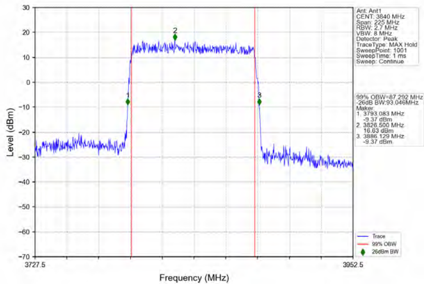
n77a_30kHz_SISO_NTNV_90MHz_DFT-s-OFDM_16_QAM_3840MHz_Outer_Full
