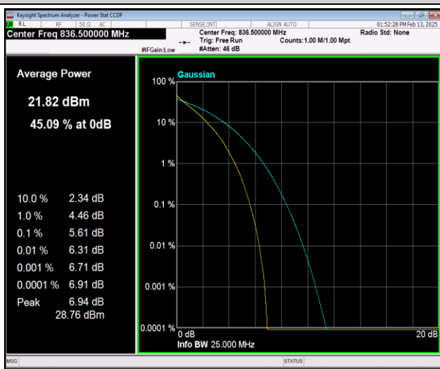
Band5-10MHz-64QAM-20525-50RB#0
