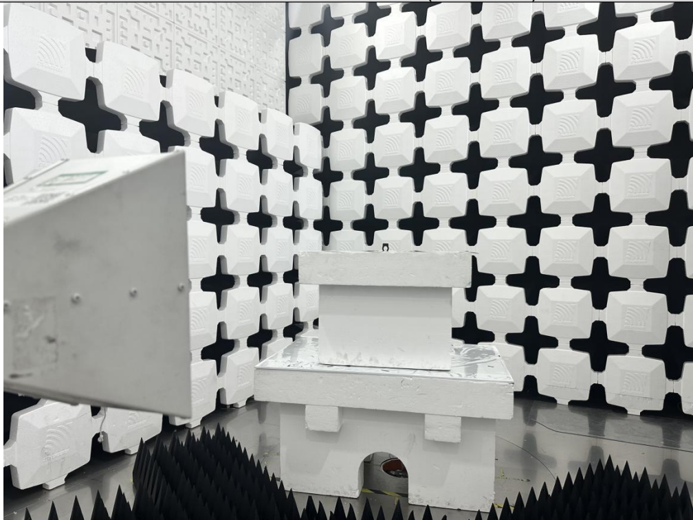
Conducted Test(SRD, 2405)
