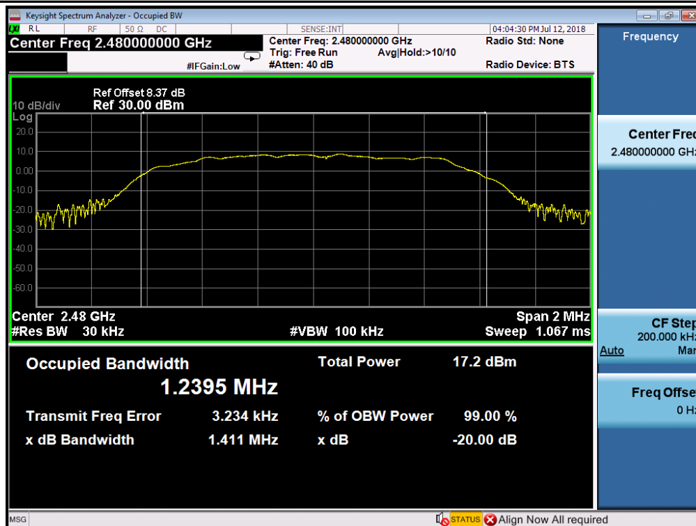
20 dB Bandwidth_3DH5_2480
