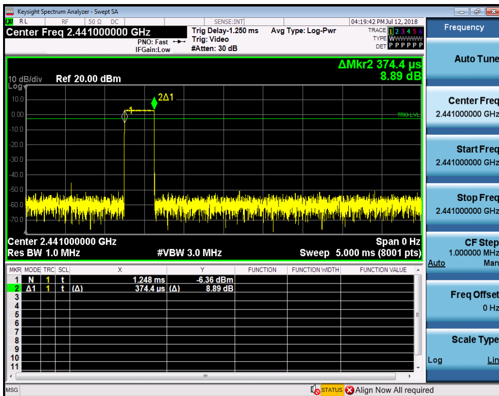
Dwell Time_DH1_2441
