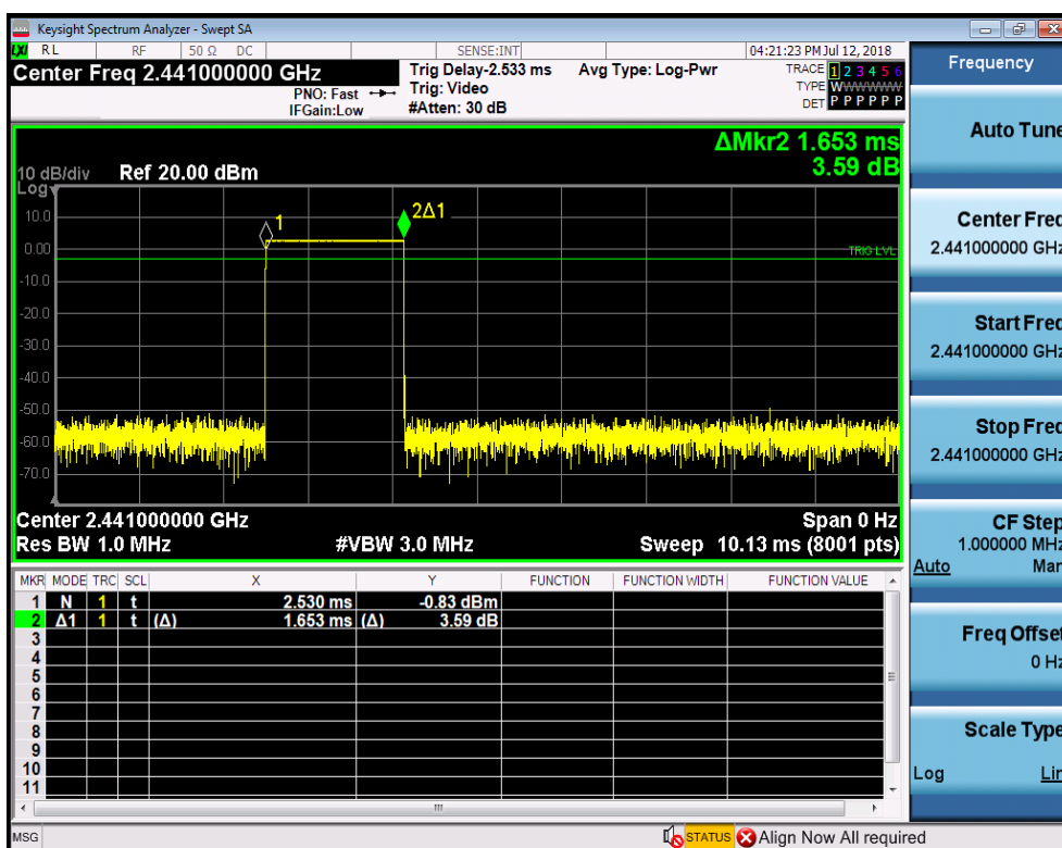
Dwell Time_DH3_2441
