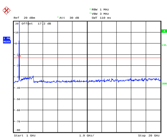
WCDMA Band IV CH-Middle 1GHz ~20GHz
