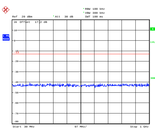
WCDMA Band IV CH-Middle 30MHz~1GHz
