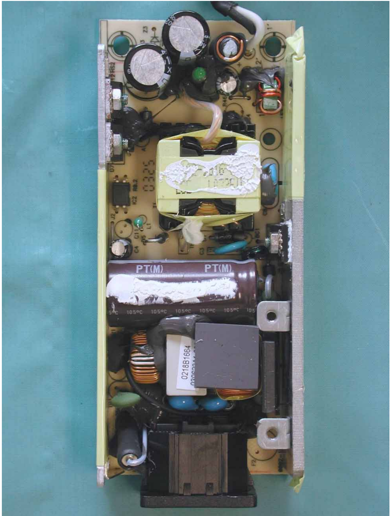
PCB Layout (Li Shin)
