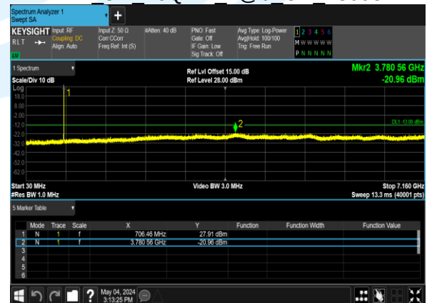
B12 3M 16QAM 1@0 CH 23095
